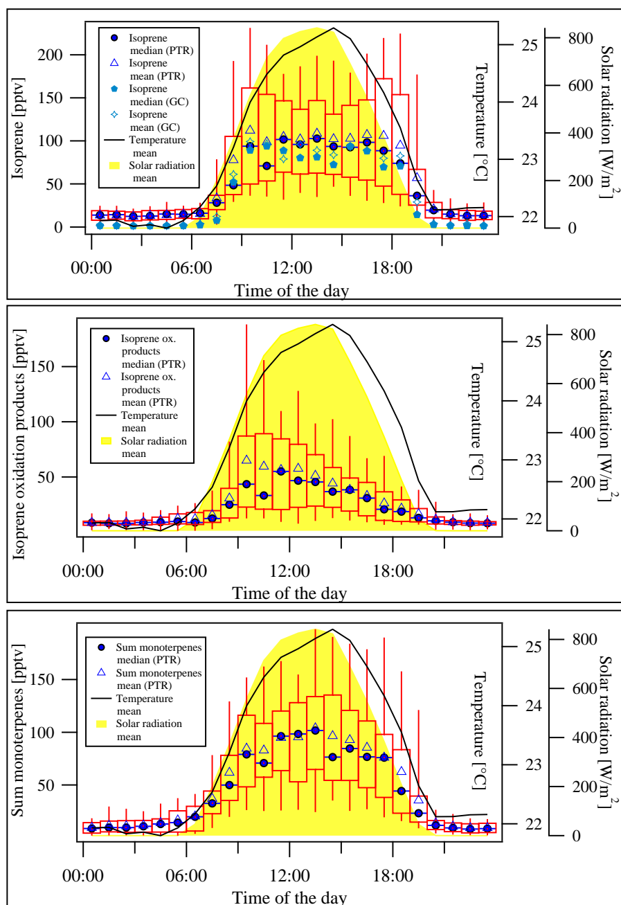
Figure 3. Box and whiskers plots of isoprene, the oxidations products of isoprene and the sum of monoterpenes for the whole campaign with a 1 h time resolution as measured by the PTR-TOF-MS. For comparison the median and mean isoprene values measured by GC-MS were added in the upper panel. To calculate the boxplots PTR-TOF-MS data with a time resolution of 10 min and GC-MS data with a 45 min time resolution (20 min sampling time) were used. The contaminations in isoprene and the monoterpenes determined by comparing GC-MS and PTR-TOF-MS data were cut. The box contains 50 % of the data. 25 % of the data lie below the lower end of the box, 75 % below the upper end. The whiskers present the 5–95 % range of the data.
