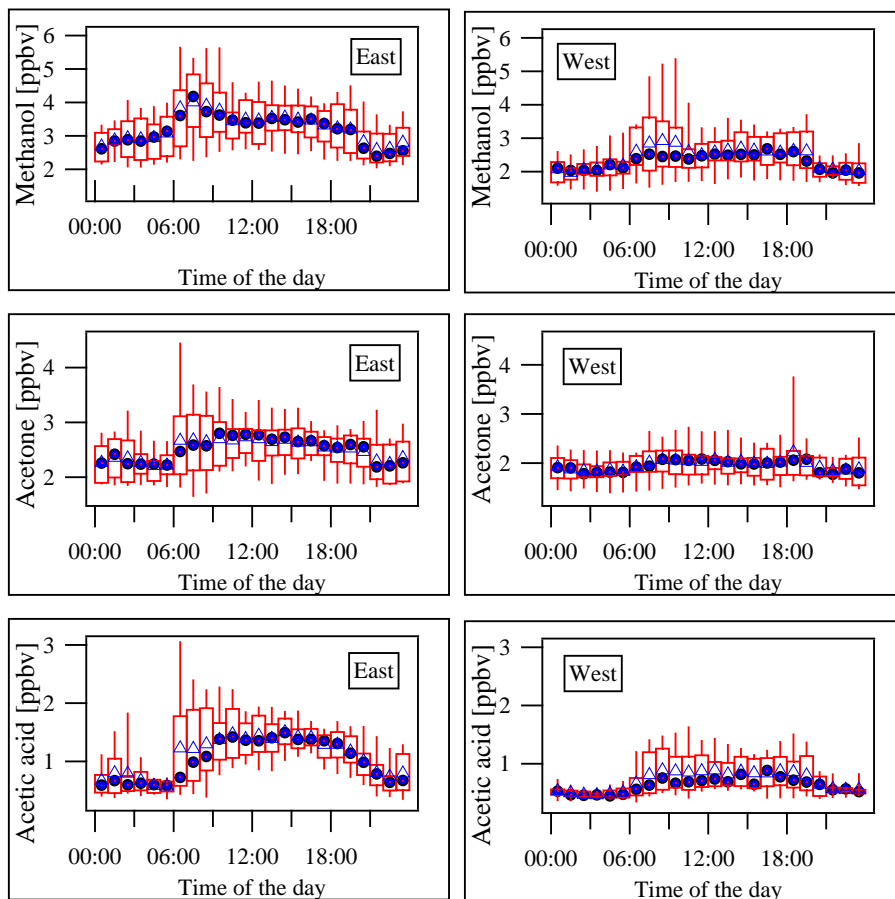
Figure 4. Box and whiskers plot of acetone, methanol and acetic acid when the site was within the PBL. The triangles refer to mean and the circles to median values. The box contains 50 % of the data. 25 % of the data lie below the lower end of the box, 75 % below the upper end. The whiskers present the 5–95 % range of the data.
