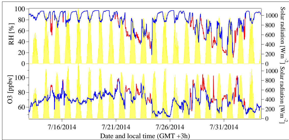
Figure 7. Ozone in ppbv, relative humidity in % and solar radiation in \text{Wm}^{-2} (10 min mean values). The red data points are influenced by air masses from the residual layer/free troposphere.
