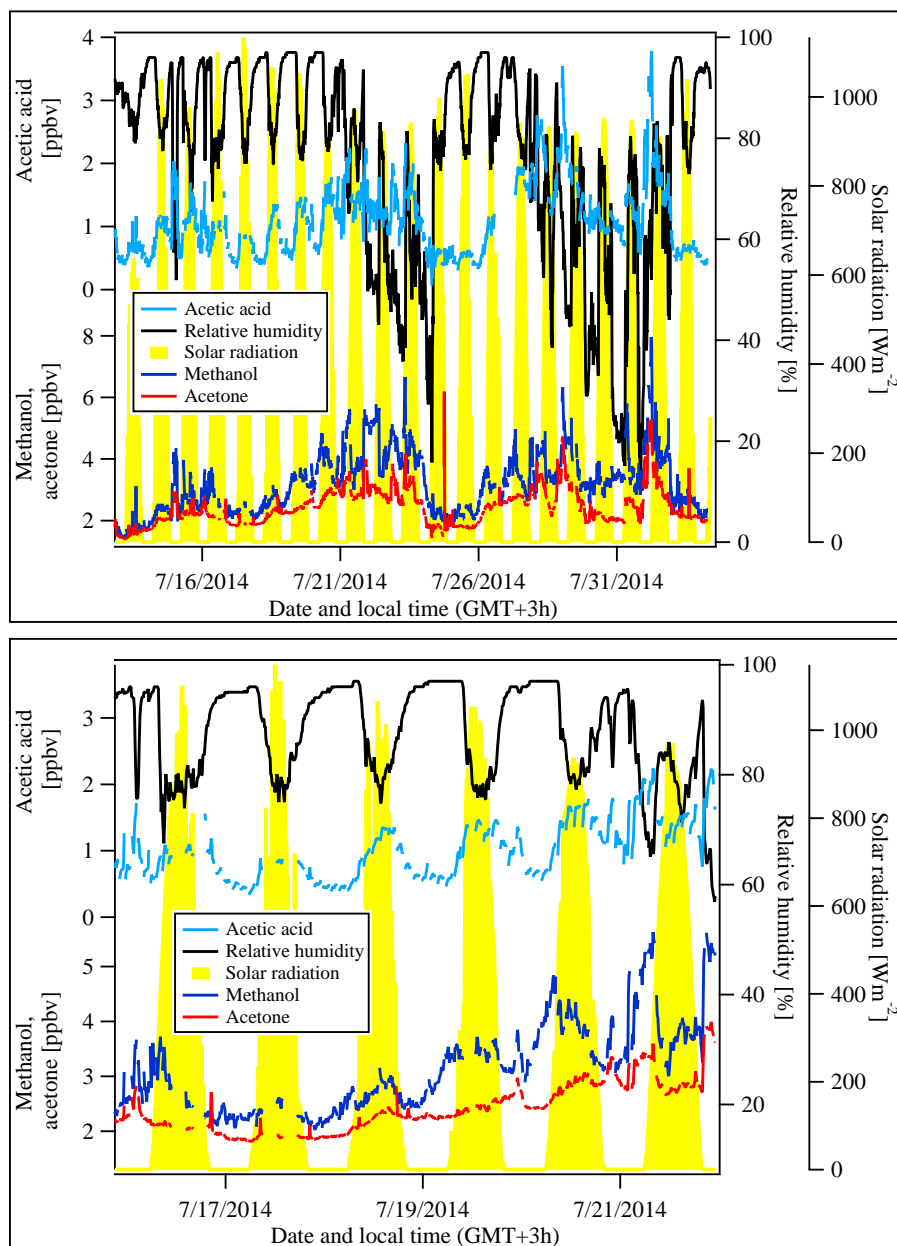
Figure 5. Mixing ratios of acetic acid, acetone and methanol in ppbv, relative humidity in % and solar radiation in \text{Wm}^{-2} (10 min mean values) as a function of time. The lower panel is a zoom in from 16 to 21 July.
