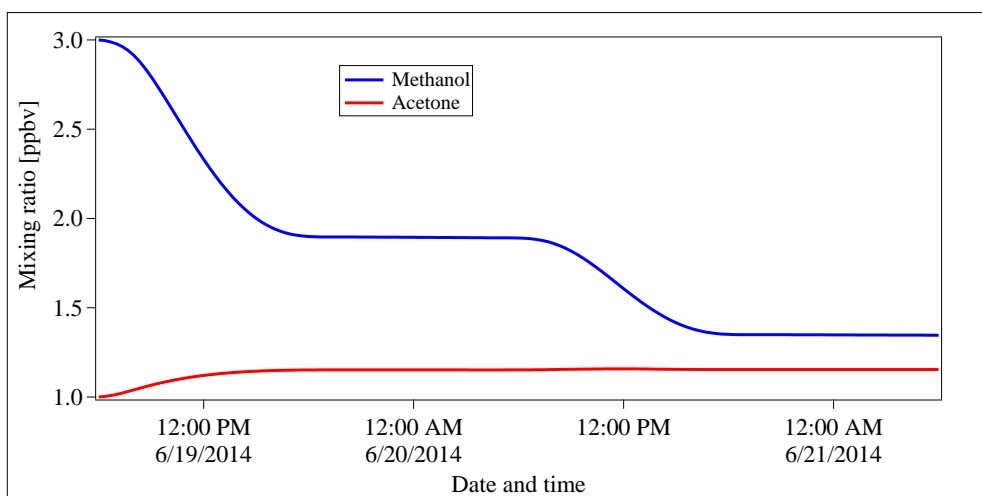
Figure 8. Modeled mixing ratios of methanol and acetone in ppbv over the period of 48 h starting at 6 am. Initial values originate from the MOM chemistry in the global model EMAC (Jöckel et al., 2016).
