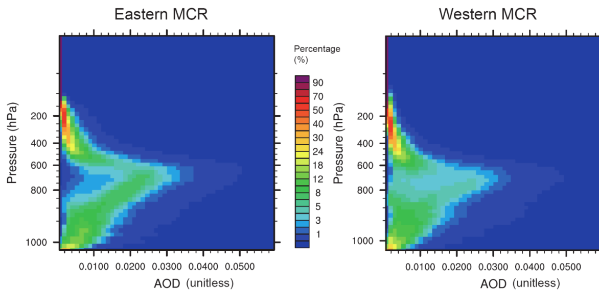
Figure. 5 AOD CFADs (Contoured Frequency Altitude Diagrams) for the eastern and western MCR regions (based on the first 96 hour forecasts for Jul.8-Sep. 18)
