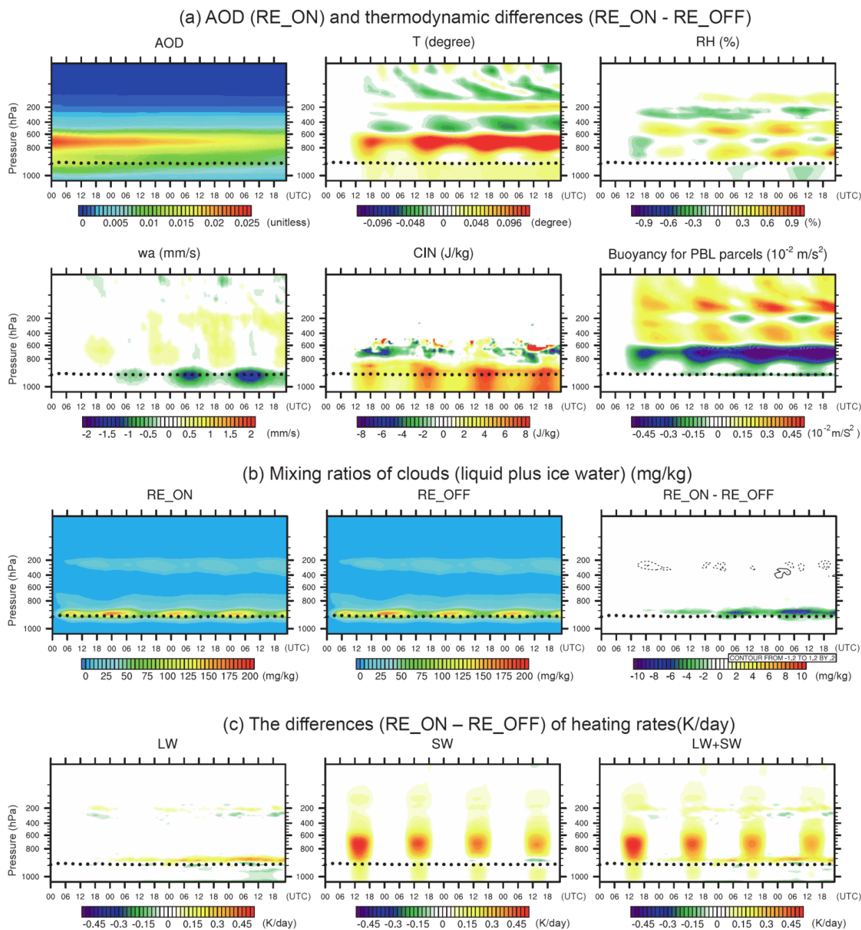
Figure 7. Same as Fig. 6 but for the “Elevated Dust” in the western MCR.
