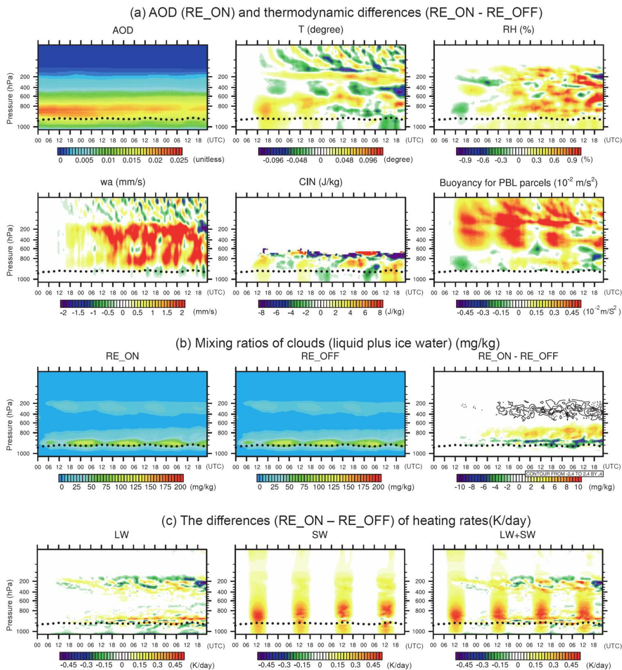
Figure 8. Same as Fig. 6 but for the “Deep Layer of Dust” in the eastern MCR.
