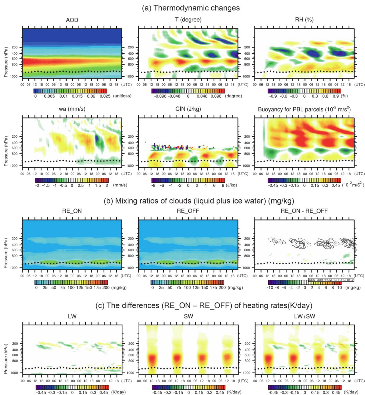
Figure 6. Averaged parameters as a function of pressure layers in hPa (y-axis) and the first 96-hour forecast time (x-axis, in UTC time) of the “Elevated Dust” in the eastern MCR from two experiments (Jul. 8 - Sep 18). (a) AOD from RF_ON, and differences (RE_ON - RE_OFF) for temperature (degree), relative humidity (%), vertical velocity (mm/s), CIN (J/kg) and Buoyancy for boundary layer parcels ( 10^{-2} \text{ m/s}^2 ). (b) mixing ratios of clouds (liquid plus ice water) (mg/kg); the RE_ON - RE_OFF differences of ice clouds were given as contour lines (negative values in dash lines). (c) the differences of heating rates (K/day) due to LW, SW and LW+SW radiative effects respectively. Black dots indicate the top of boundary layer.
