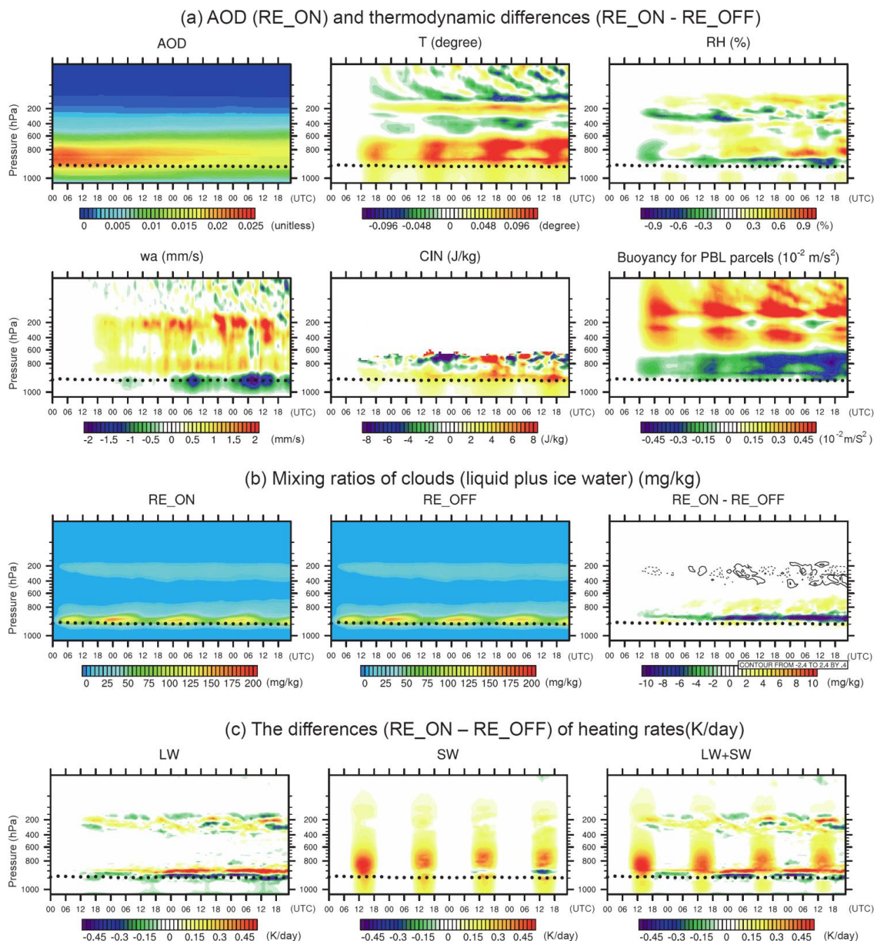
Figure 9. Same as Fig. 6, but for the “Deep Layer of Dust” in the western MCR.
