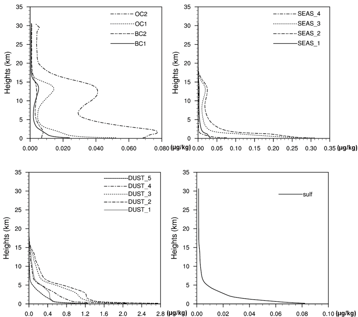
5 Figure 1. Domain-averaged standard deviations of background errors ( \mu\text{g/kg} ) as a function of height for each aerosol variable.
