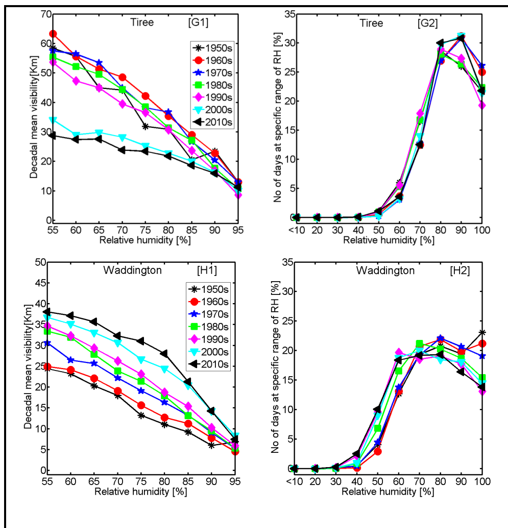
Figure 4 Decadal visibility at specific range of relative humidity (left side) and number of days in % during different relative humidity (right side)
