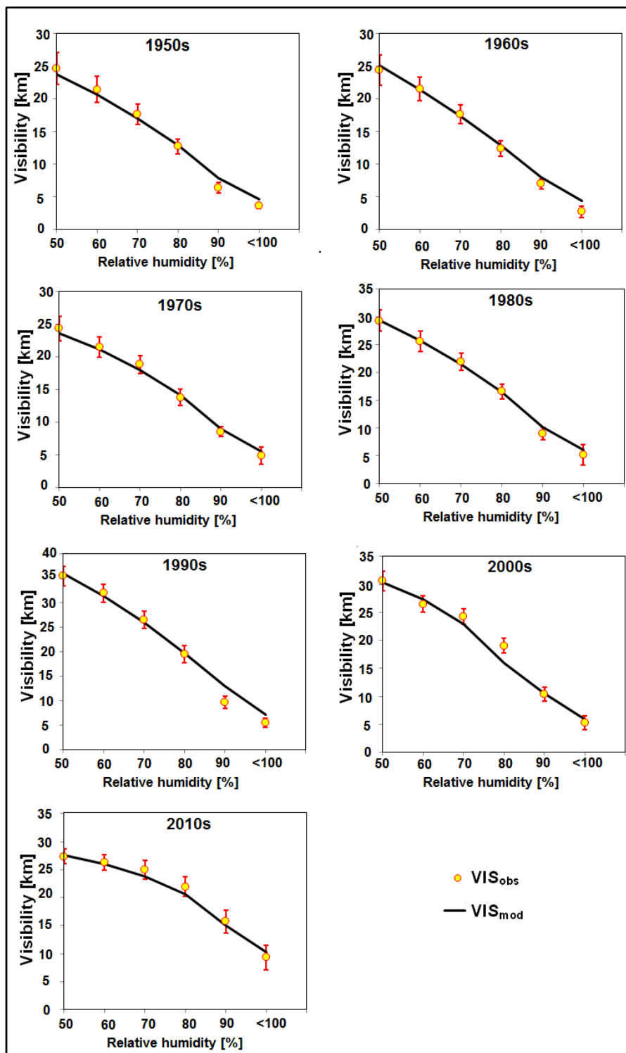
Figure 6 Comparisons of modelled and observed visibility at specific range of RH using Eq. (4) at Heathrow station. The observed visibility is presented with standard error bars at 95 % confidence interval.
