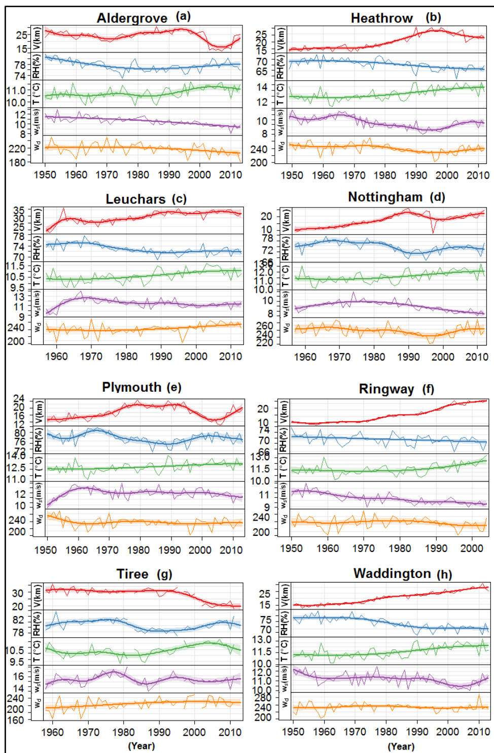
Figure 5 Time-series of meteorological components relative humidity (RH), air temperature (T), wind speed ( w_s ), and wind direction ( w_d ) including visibility (V), where shaded lines show smooth fit line at 95 % confidence interval.
