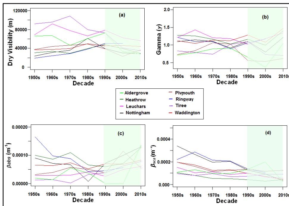
Figure 7 Model output parameters a) Dry visibility, b) gamma and c) absorption coefficient and d) scattering coefficient at 75 % n.b. from 1950s to 2010s. The green shaded region shows the start of visiometer era at most of the stations (see supplementary Table S1 to see the starting year of visiometer measurement).
