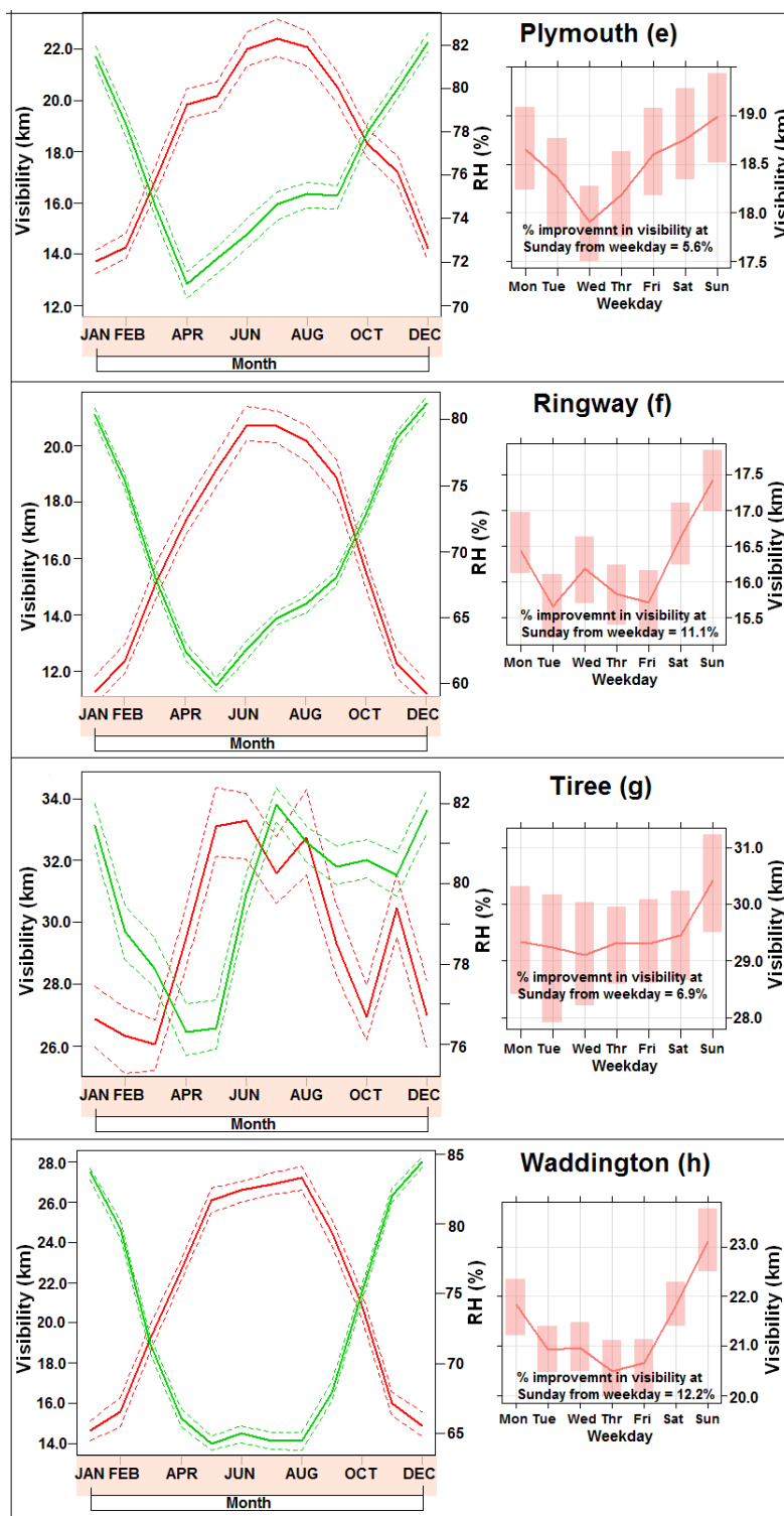
Figure 3 Mean monthly visibility and RH (Left-side) and average weekday visibility (Right-side) at all eight sites: a) Aldergrove b) Heathrow c) Leuchars d) Nottingham e) Plymouth f) Ringway g) Tiree h) Waddington.
