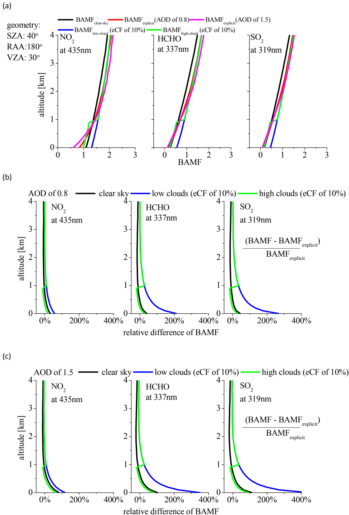
Figure 16: (a) simulated BAMF_{clear-sky} , BAMF_{explicit} for AOD of 0.8 and 1.5, BAMF_{low-cloud} (cloud at surface) and BAMF_{high-cloud} (cloud at 1km) of NO_2 at 435nm, HCHO at 337nm and SO_2 at 319nm for one typical satellite observation (SZA of 40°, RAA of 180° and VZA of 30°). An effective cloud fraction of 10% is used in the calculations. (b) Relative differences of BAMF_{clear-sky} , BAMF_{low\ clouds} and BAMF_{high-clouds} compared to BAMF_{explicit} for AOD of 0.8. (c) Same with (b) but BAMF_{explicit} for AOD of 1.5.
