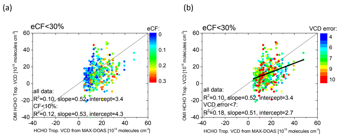
Figure 6: (a) HCHO tropospheric VCDs for OMI pixels for eCF < 30% are plotted against those derived from MAX-DOAS observations with the color map of eCF; the linear regression parameters are acquired for eCF < 30% and for eCF < 10%, respectively. (b) Scattered plots are same as in (a), but with the color map of VCD fit error; linear regression parameters are acquired for all data and for VCD fit error < 7 \times 10^{15} molecules cm^{-2} .
