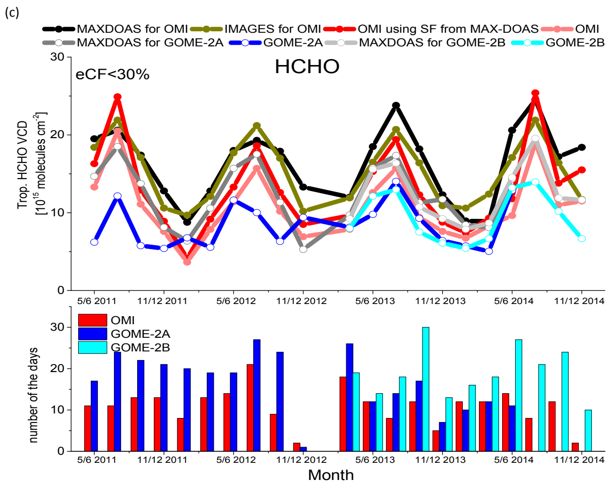
Figure 12: Bi-monthly averaged tropospheric VCDs of NO 2 (a), SO 2 (b), and HCHO (c) derived from coincident satellite and MAX-DOAS observations for eCF <30%. Also shown are the corresponding CTM results (TM4 for NO 2 , IMAGES for SO 2 and HCHO). In all subfigures
