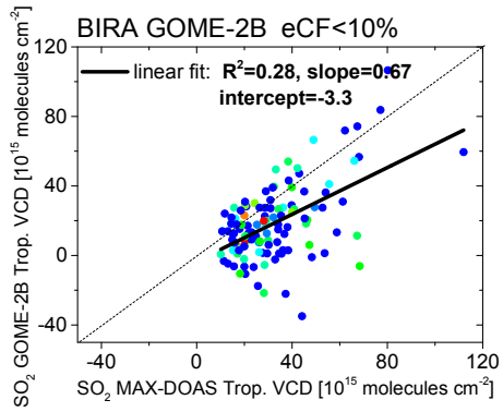
Figure 4: Daily averaged OMI SO 2 tropospheric VCDs from BIRA (a) and NASA (b), GOME -2A SO 2 tropospheric VCDs from BIRA (c) and DLR (d) and GOME-2B SO 2 tropospheric VCDs from BIRA (e) for eCF < 10% plotted versus the coincident MAX-DOAS results. The colors indicate the eCF.
