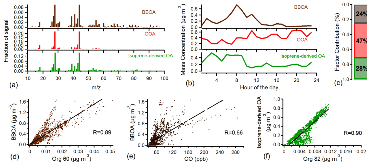
5 Figure 6: (a) Mass spectra, (b) diurnal trends, (c) contribution and (d), (e), (f) correlations for the PMF 3-factor solution for background periods including BBOA, OOA and isoprene-derived OA factors.
