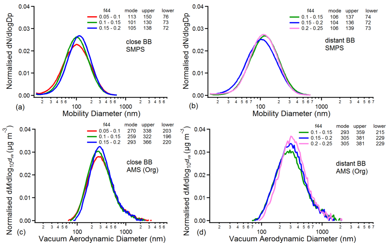
5 Figure 5: SMPS size distributions (dN/dlogDp, normalised to total particle number concentration, versus mobility diameter) binned by the AMS f44 for close (a) and distant (b) BB periods and AMS size distributions (dM/dlog 10 d va , normalised to total OA concentration, versus vacuum aerodynamic diameter) binned by the AMS f44 for close (c) and distant (d) BB periods.
