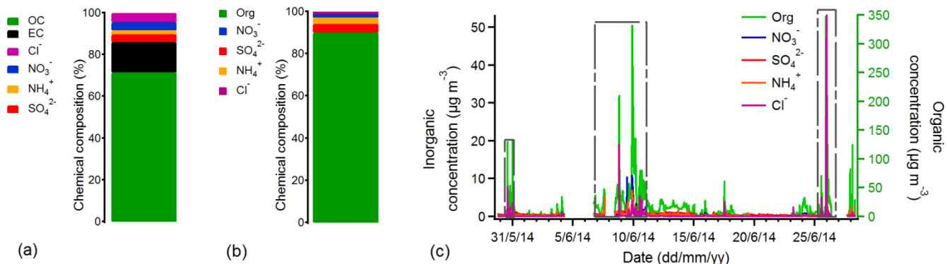
Figure 1: Contributions of (a) OC, EC and inorganics collected on filters and the contribution of (b) AMS OA and inorganics in non-refractory submicron aerosol, as well as (c) their time series. Close BB periods are marked in the AMS time series with grey dashed boxes. The distant BB periods cover all days of the measurement other than days included in close BB periods. Gaps in the AMS time series indicate gaps in the sampling.
