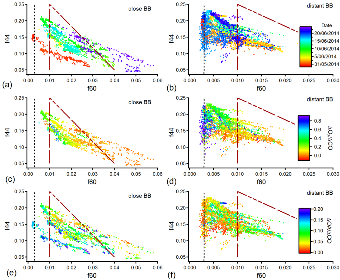
Figure 4: f44 vs. f60 coloured by date for (a) close and (b) distant BB periods, by \Delta\text{O}_3/\Delta\text{CO} ratio for (c) close and (d) distant BB periods, and by \Delta\text{OA}/\Delta\text{CO} ratio for (e) close and (f) distant BB periods (vertical dashed black lines refer to the f60 background level of 0.003). Red dashed lines refer to the ambient BBOA-related data space introduced by (Cubison et al., 2011). Note: ozone data from the 29 th of May until the 1 st of June were not available.
