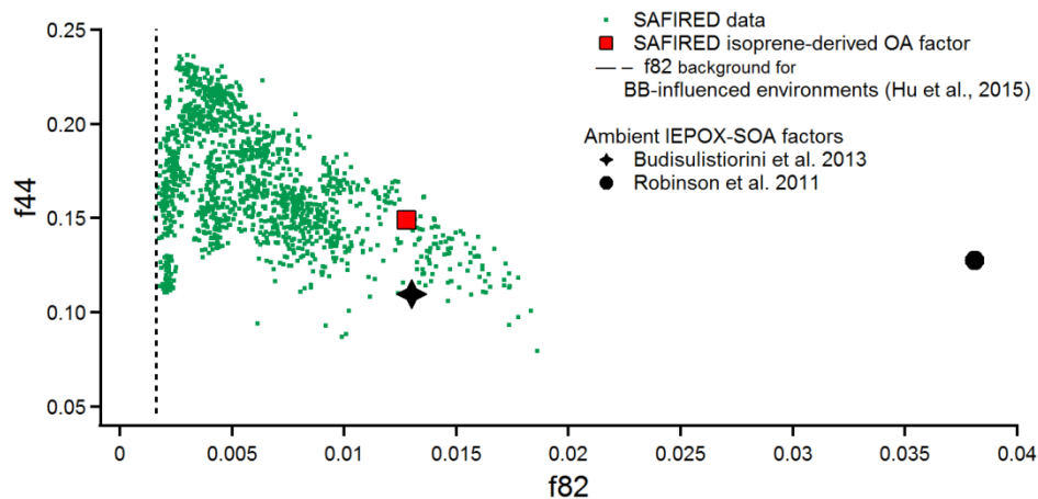
10 Figure 7: f_{44} ( \text{CO}_2^+ ) vs. f_{82} ( \text{C}_5\text{H}_6\text{O}^+ ) for the SAFIRED data; The isoprene-derived OA factor from SAFIRED and two other ambient campaigns (Budisulistiorini et al., 2013; Robinson et al., 2011) are marked. Vertical black dashed line indicates proposed background f_{82} value in environments strongly influenced by BB (Hu et al., 2015).
