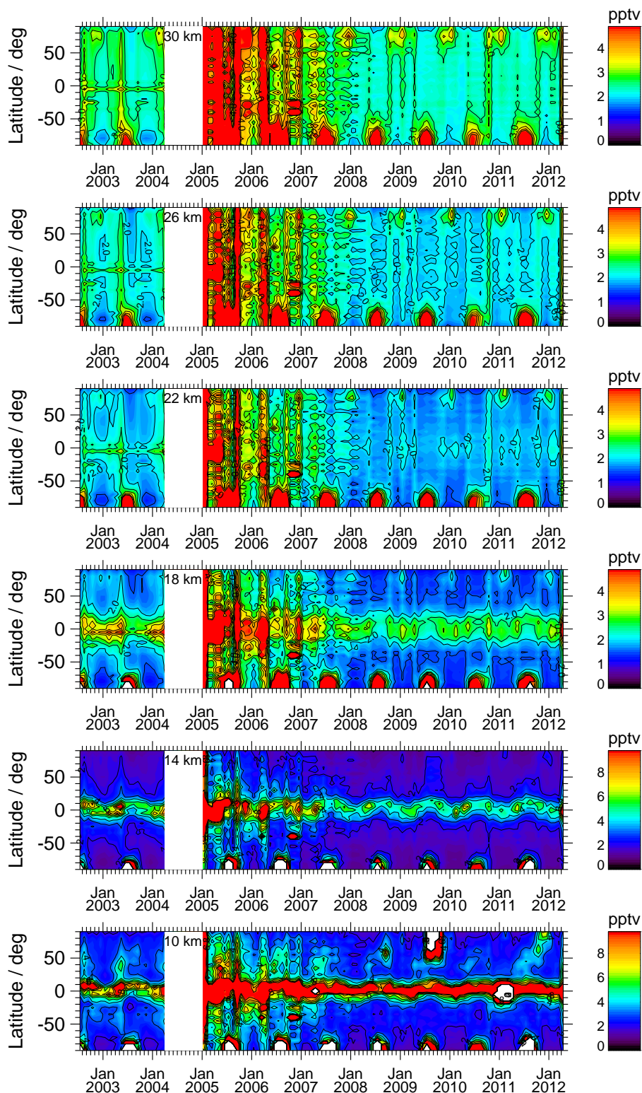
Time series of the ESD of the bin-averaged OCS values measured by MIPAS at 30 km, 26 km, 22 km, 18 km, 14 km and 10 km (top to bottom). The white area in 2004 is a data gap due to operational shutdown of MIPAS and the remaining white areas are caused by cloud contamination. Note the different colour ranges. Values outside of the colour ranges are also labelled in black or red, respectively.
