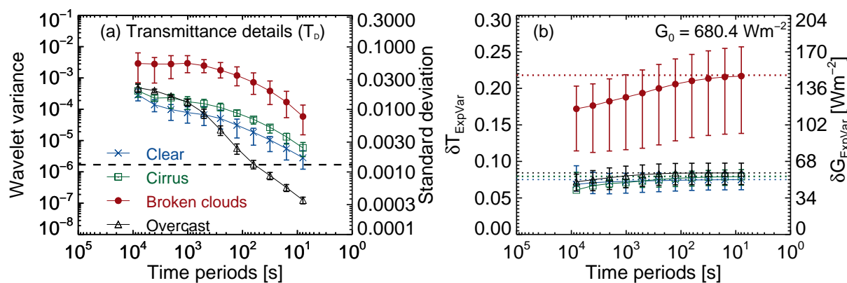
Figure 5. (a) Wavelet variance, and the (b) cumulative variance (from Eq. 1) of global transmittance from all the pyranometer stations in the observation domain as a function of considered frequency/averaging period for cases during the HOPE campaign. The vertical bars around the mean value represent the observed minimum and maximum variances. The dashed horizontal lines in (b) denote the total variance of the original time series averaged across all stations within the observation domain.
