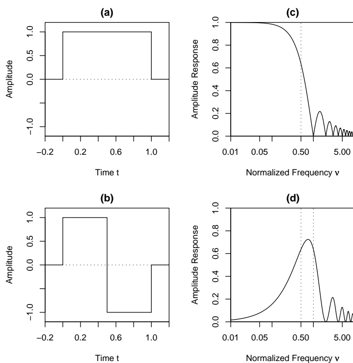
Figure 1. Time representation of the Haar (a) scaling and (b) wavelet function, and the frequency response of the associate (c) lowpass and (d) bandpass filters. Adopted from Deneke et al. (2009).
