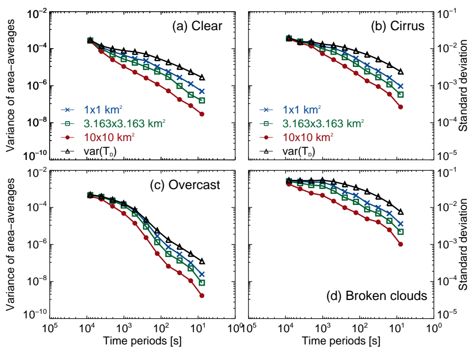
Figure 8. Power spectrum of spatially averaged transmittance as a function of frequency under different sky conditions: (a) clear, (b) cirrus, (c) overcast, and (d) broken clouds. var(T_D) denotes the power spectrum of a point measurement of global transmittance as shown in figure 5a).
