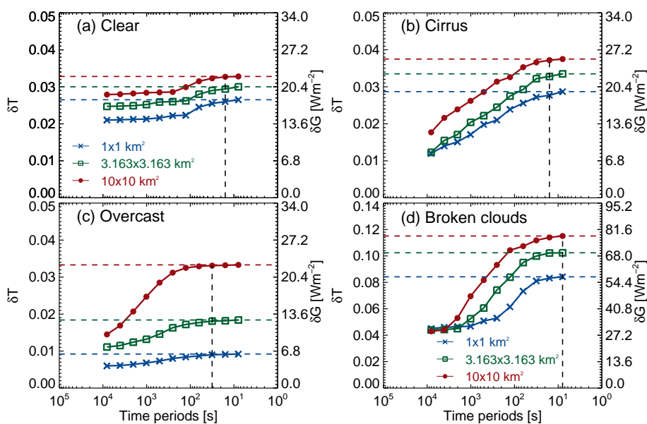
Figure 10. Area averaging error in the global transmittance ( \delta T ) and corresponding global radiation ( \delta G , in \text{W m}^{-2} ) with different sky conditions: (a) clear, (b) cirrus, (c) overcast, and (d) broken clouds for different domain sizes represented as a function of averaging time periods. The dashed horizontal lines correspond to the maximum deviation observed for the different domain sizes. Dashed vertical lines represent the minimum averaging time above which the area averaging errors are less sensitive at different spatial resolutions.
