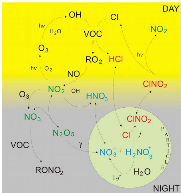
Fig. 1. Gas- and aqueous-phase chemical processes forming CINO_2 and particulate nitrate indicating the role of CINO_2 in modifying the effect of N_2O_5 uptake on the chemical lifetime of NO_x and photochemical RO_2 generation.
