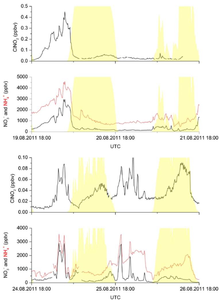
Fig. 4. Zoom-in on particle-nitrate and CINO 2 formation on 4 nights. Global radiation (yellow) is plotted to separate day-night periods and indicate the day-to-day, relative photochemical activity. Note that the CINO 2 plotted for these days was measured at m/z = 161.9 and therefore contains a contribution from HCl, hence the apparent daytime production.
