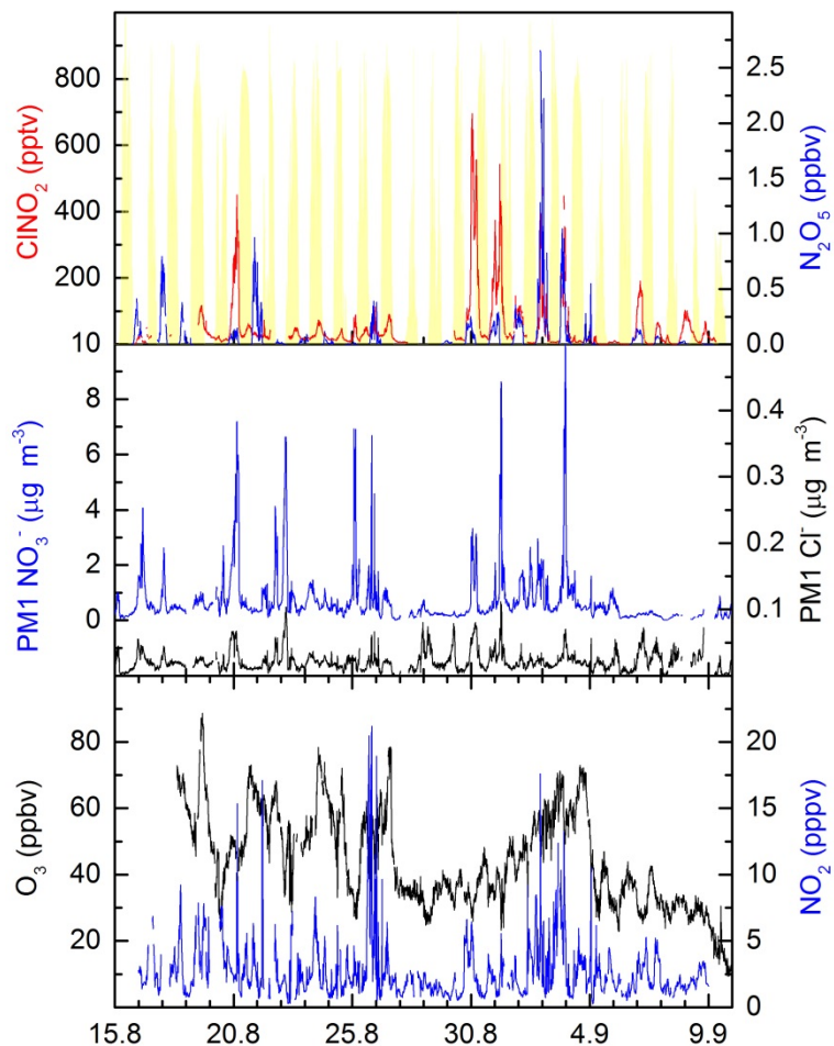
Fig. 3. Time series of CINO 2 and its precursor, N 2 O 5 . Global radiation (yellow) is plotted to separate day-night periods and to indicate the day-to-day, relative photochemical activity. The precursors to N 2 O 5 (NO 2 and O 3 ) are shown as are the AMS measurement of particulate nitrate (as in Fig. 2) and chloride.
