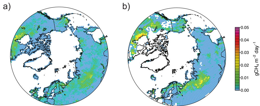
Figure 5. Wetland emissions estimates (units \text{gCH}_4 \text{ m}^{-2} \text{ day}^{-1} ) from LPX-Bern (a) and LPJ-DGVM (b).
