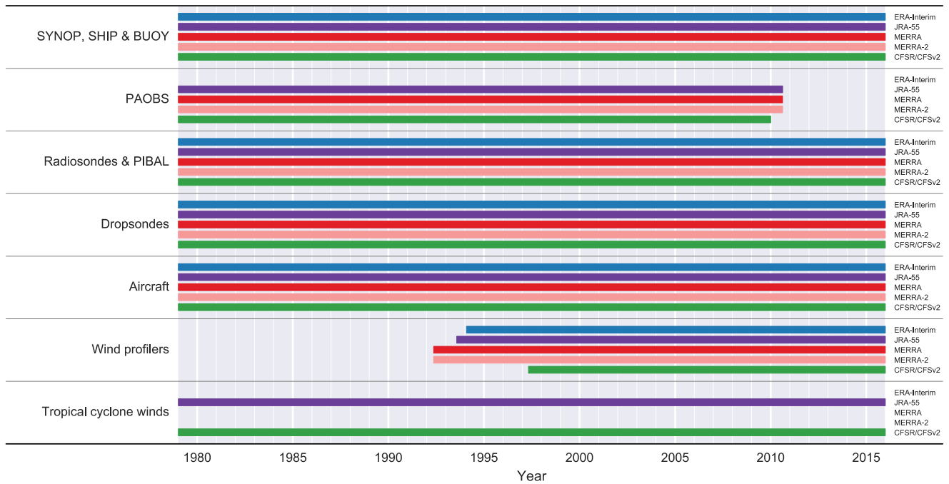
5 Figure 6. Timelines of conventional observations assimilated by the ERA-Interim (blue), JRA-55 (purple), MERRA (dark red), MERRA-2 (light red), and CFSR (green) reanalysis systems. See Appendix A for acronym definitions.
