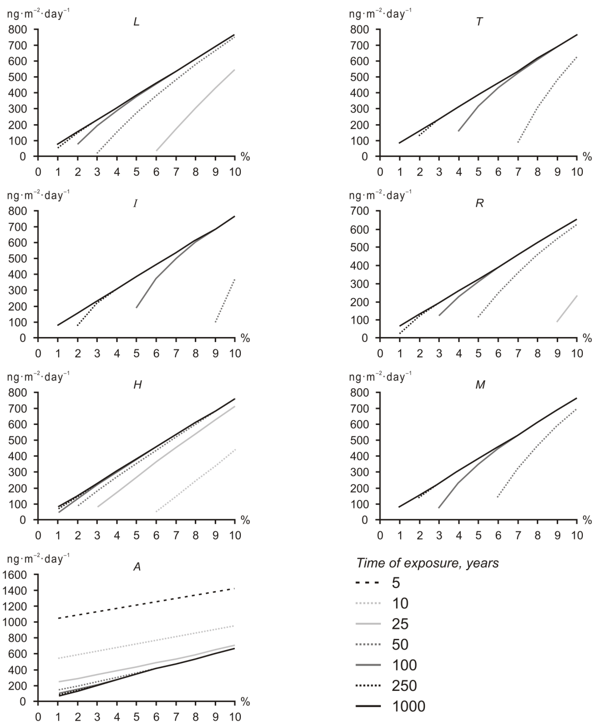
Figure 2: The critical loads of BaP ( \text{ng} \cdot \text{m}^{-2} \cdot \text{day}^{-1} ) plotted against its degradation intensities (%) and exposure time (years) for the different land-use zones in the Eastern Administrative District of Moscow. The land-use zone abbreviations are explained in Table 1.
