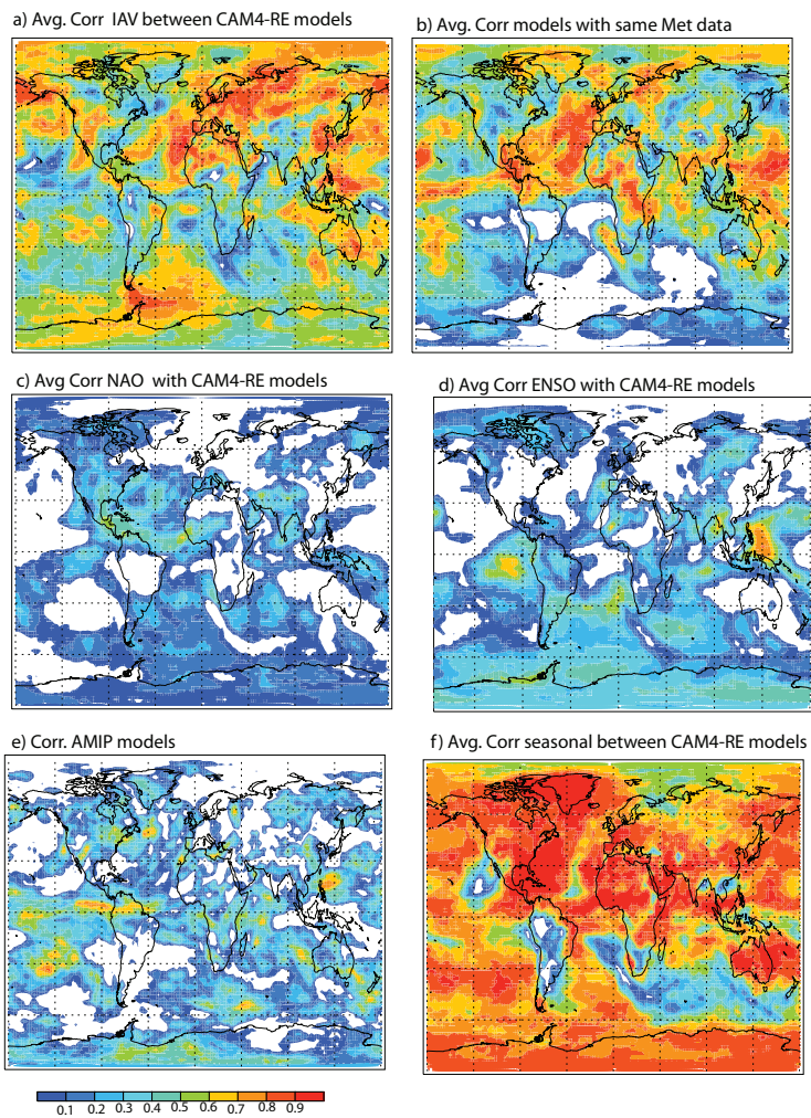
Figure 8: Spatial plot of the average temporal rank correlation of the annual mean modelled values. The correlation is calculated between the CAM4-Reanalysis models (CAM4 (MERRA));
