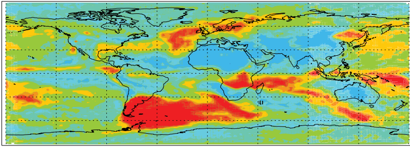
Figure 11: Monte Carlo-based estimation of the number of monthly mean observations required to obtain a 95% chance of obtaining a mean and standard deviation consistent with the true model mean between 1990-2005 at each gridbox, based on model simulations using the CAM4 (MERRA) model. More details on methods in Section 2.3.
