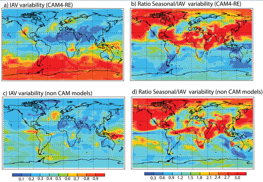
Figure 6: Spatial plot of the modelled IAV variability in the model simulations at each grid box (CAM4-RE is the mean of CAM4 (MERRA), CAM4 (NCEP) and CAM4 (ERA-Interim)), where variability is unitless and is the standard deviation divided by the mean of the annual mean between 1990 and 2005 for a) surface concentration. The ratio of the seasonal variability over the IAV variability (calculated using the 12 climatological monthly means) is shown in the right hand panel for b) surface concentration. Similar diagnostics for the non-CAM models (GCHEM(MERRA) and MATCH (NCEP)) are shown in the bottom panel for a) IAV in variability and b) ratio of seasonal over IAV variability for concentration.
