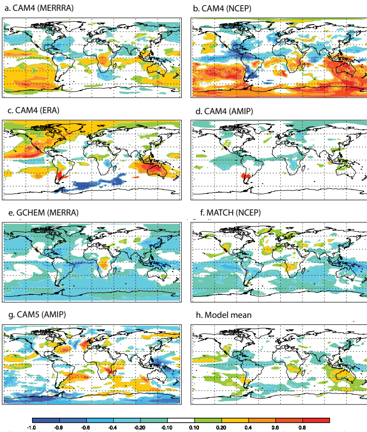
Figure 4: Slope of the trend in the relative concentrations (linear regression of concentration onto time) of the modelled annual mean surface concentrations (normalized by the mean) in units of fraction change per decade for a) CAM4 (MERRA), b. CAM4 (NCEP), c. CAM4 (ERA), d. CAM4 (AMIP), e. GCHEM (MERRA), f. MATCH (NCEP), g. CAM5 (AMIP) and the mean slope across the models (h). Only slopes that are larger in magnitude than one sigma from the regression are plotted. Positive slopes imply increasing concentrations.
