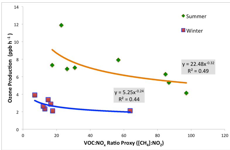
Figure 10: Plot of measured ozone production from the DISCOVER-AQ campaign near Fresno during winter (maroon squares) and from the ArvinO3 study during the summer (green diamonds) versus a proxy of VOC:NO x ratio estimated by the measured CH 4 enhancement over global background divided by the NO x measured during the flights from the CARB air quality monitoring network nearby.
