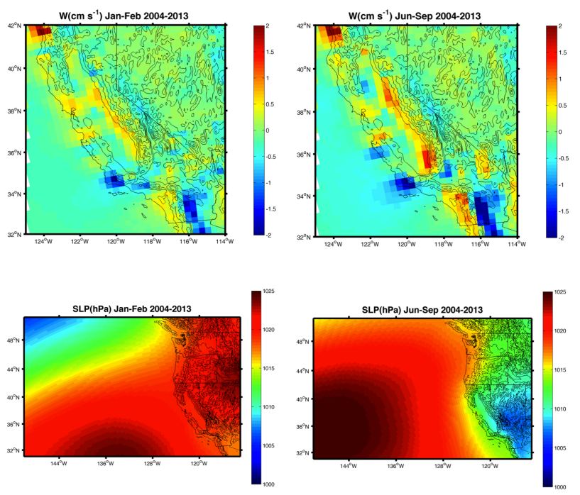
Figure 1: W (vertical velocity), converted from omega (pressure velocity), at the 900 hPa level and mean sea level surface pressure. Plotted for two intervals Jan–Feb and June–Sept. for 10 years from 2004–2013. The months chosen for the two separate plots represent the time frame of the flights.
