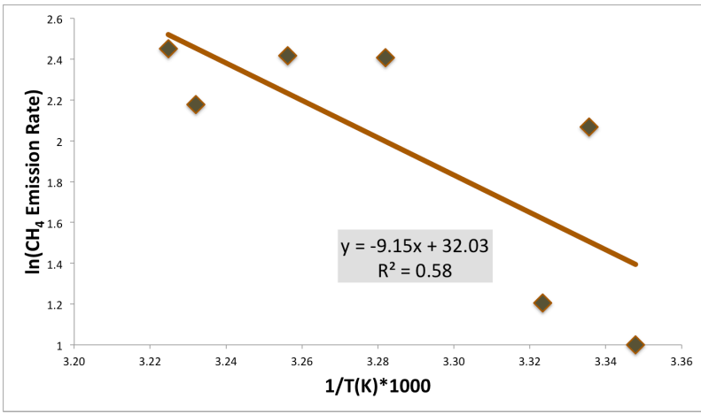
Figure 11: Arrhenius plot of the estimated methane emission rate from each flight and the average ABL temperature from the ArvinO3 study where methane emissions are believed to be dominated by agricultural sources.
