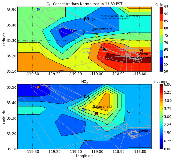
Figure 9: Horizontal patterns of O 3 (top) and NO 2 (bottom) during an ozone exceedance episode near Bakersfield on 14 August 2013. The grey lines represent the flight tracks, and the coloured circles represent the surface network observations. Because of the continual trend in ozone throughout the flight, the values in the top figure are all corrected to a reference time of 13:30 PST. The black arrow in the top figure represents the vector average wind observed in the ABL during that sortie showing a strong negative advection of ozone and a large positive advection of NO 2 into the Arvin region to the south. BFL is the Meadows Field Airport on the north end of urban Bakersfield. The coloured circles represent the 13:00-14:00 surface site measurements from the ARB surface network.
