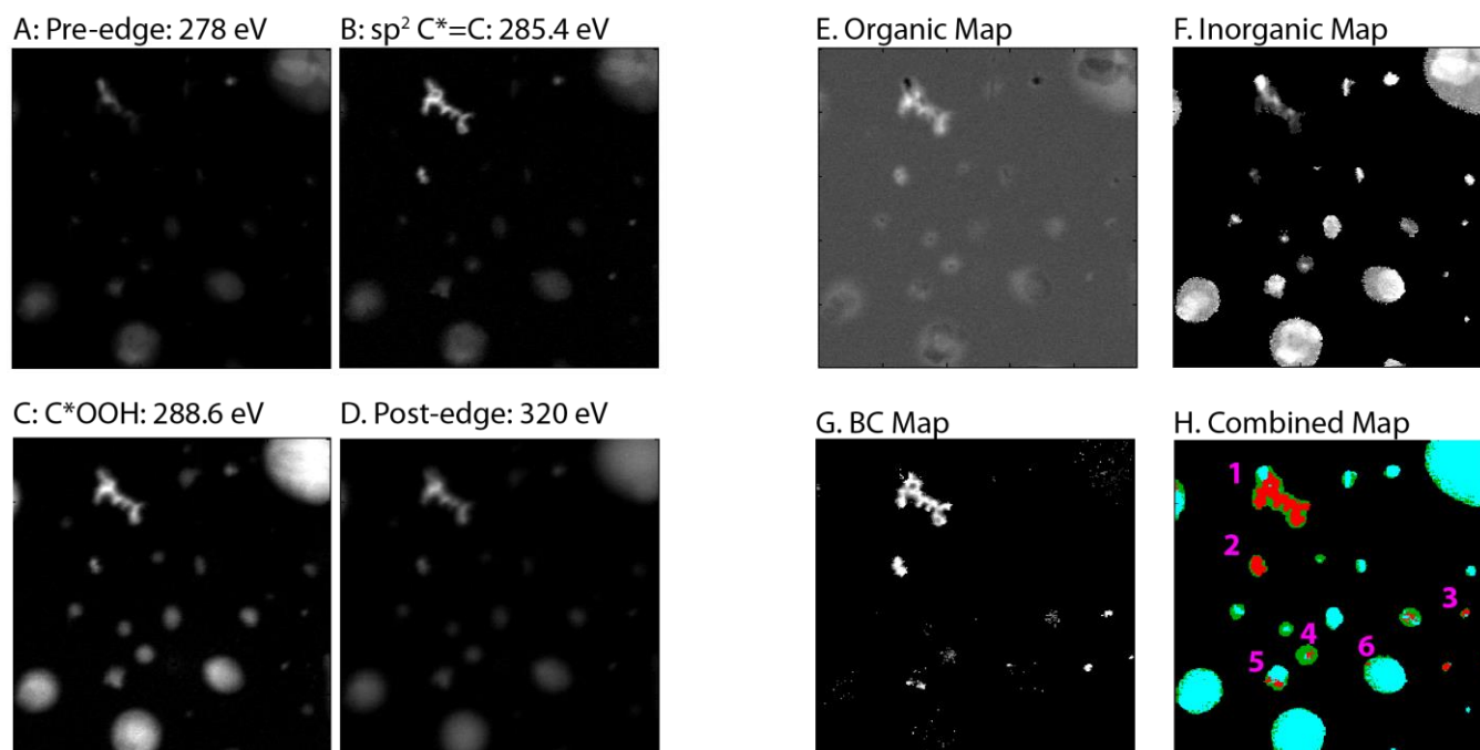
Figure 1. (A-D): Single energy images at 278, 285.4, 288.6, and 320 eV representing the pre-edge, C*=C sp 2 carbon, C*OOH, and total carbon. E) Organic map produced by subtracting the image at 278 eV from the image at 288.6 eV. F) Inorganic map produced by taking the ratio of the image at 278 eV to the image at 320 eV (Pre edge: total carbon) G) sp 2 carbon map derived by multiplying the ratio of 285.4 eV to 320 eV by a constant to give the percentage of sp 2 bonds as described in Hopkins et al. (2007) (Hopkins et al., 2007) H) Combined maps derived from thresholding of maps E-G; red areas contain %sp 2 >35%, green areas are organic dominant and blue areas are non-carbonaceous inorganic dominant .
