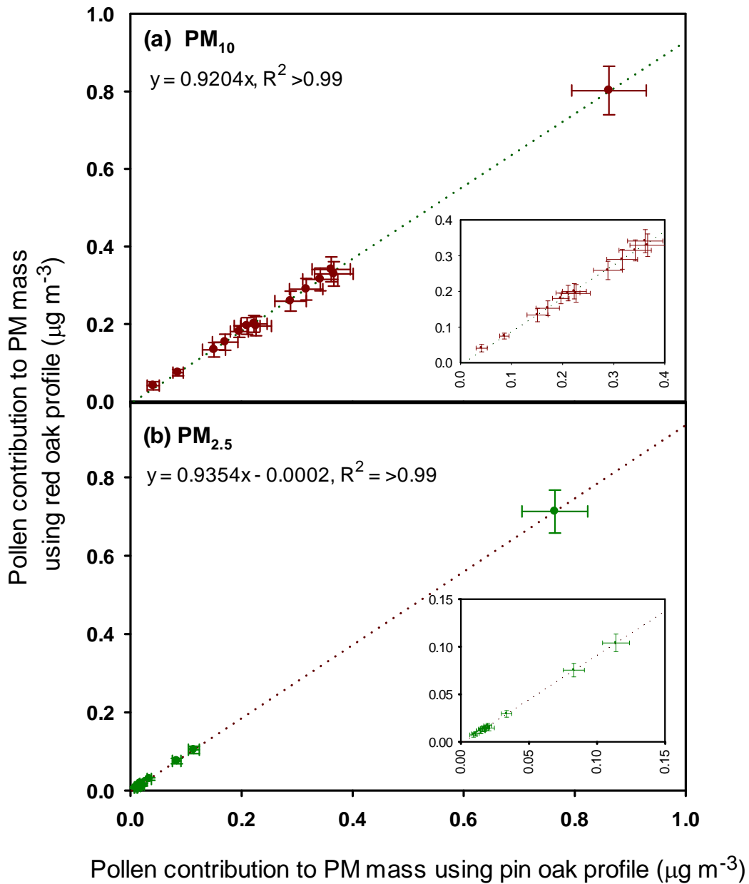
Figure S2: Comparison of pollen contributions to PM 10 (a) and PM 2.5 (b) mass, estimated by the CMB model using pin oak and red oak pollen profiles. The comparison is limited to 26 April – 9 May, after the onset of the pollen season. The strong correlation ( R^2 > 0.99 ) and numerical agreement (slopes close to 1) demonstrate the consistency in model results for when either profile is used. Consequently, source contributions from these two types were averaged to obtain the best estimate of pollen contributions to PM mass.
