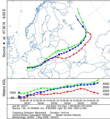
NOAA HYSPLIT MODEL Backward trajectories ending at 1500 UTC 07 May 08 GDAS Meteorological Data
