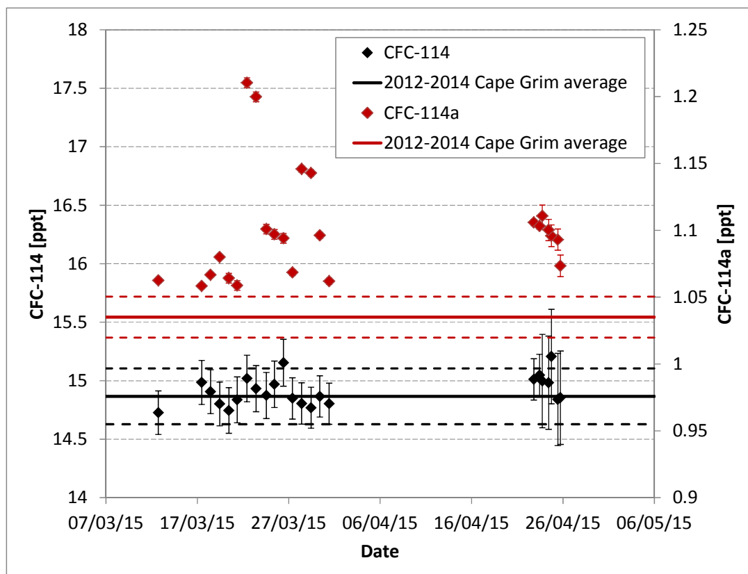
Figure 6: Mixing ratios of CFC-114 and CFC-114a from samples collected during a ground-based campaign near Hengchun, Taiwan in early 2015 (diamonds) compared to mixing ratios observed at Cape Grim averaged from 2012 to 2014 (lines). Uncertainties (error bars and dashed lines) are 1\sigma standard deviations.
