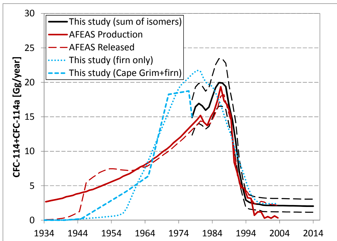
Figure 4: Atmospheric observation-based emissions of the sum of CFC-114 and CFC-114a (black line with black dashed lines representing uncertainty ranges) in comparison with “bottom-up” emissions from the AFEAS inventory. The dotted blue line are emissions purely derived from firn air observations while the dashed blue line results from matching the firn-based emissions to the Cape Grim-based emission record in 1978 while not leaving the uncertainty range of the firn-based mixing ratios from Figure 1.
