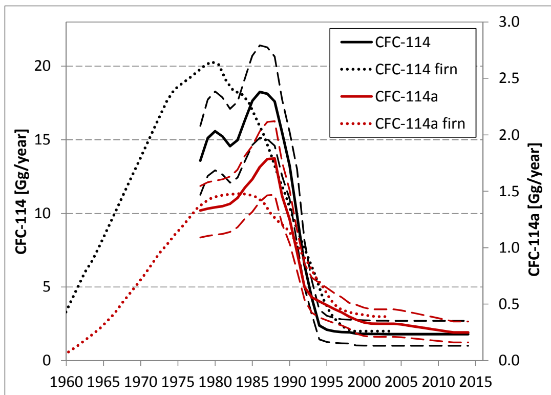
Figure 3: Global emissions of CFC-114 and CFC-114a derived from the Cape Grim observations. The dotted black lines are emissions purely derived from firn air observations with dashed lines representing uncertainty ranges.
