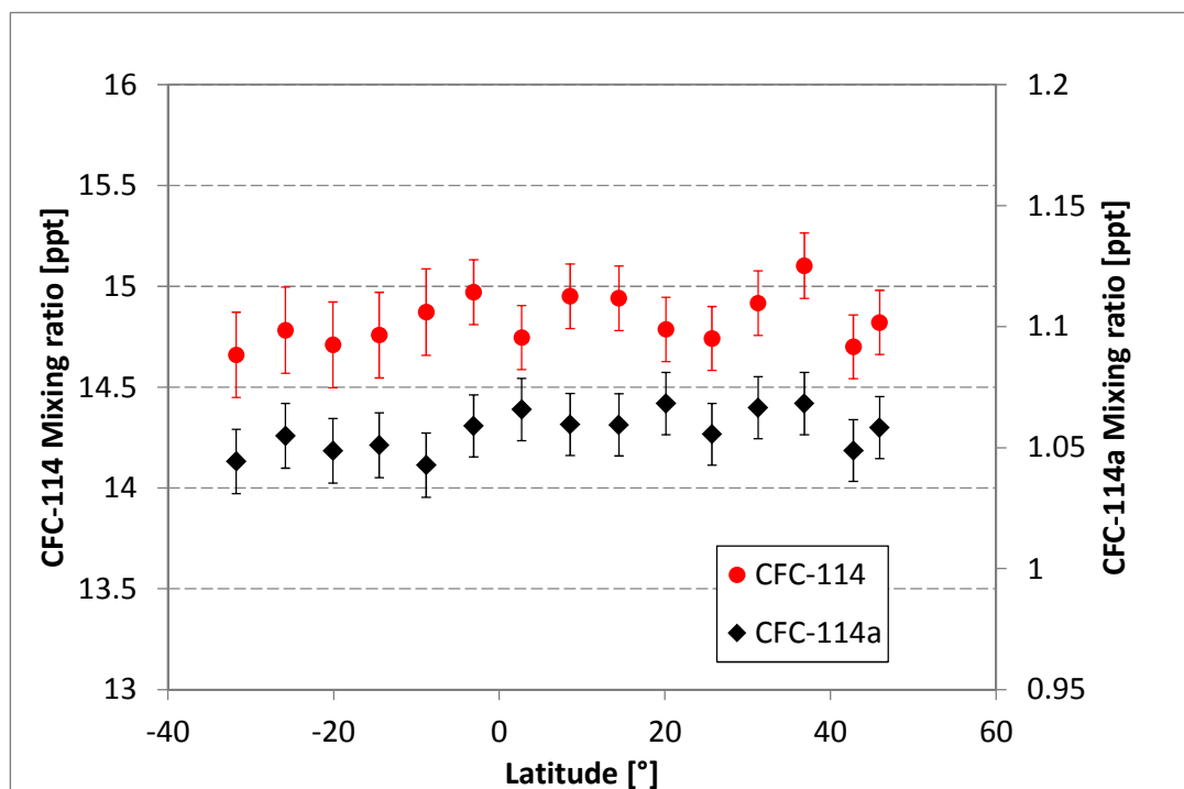
Figure 5: CFC-114 and CFC-114a observations from air samples collected during two interhemispheric aircraft flights from Germany to South Africa and back on 10-11th February 2015. Samples were collected between 8.3 and 11.6 km altitude and between 45.9°N (positive values) and 31.8 °S (negative).
