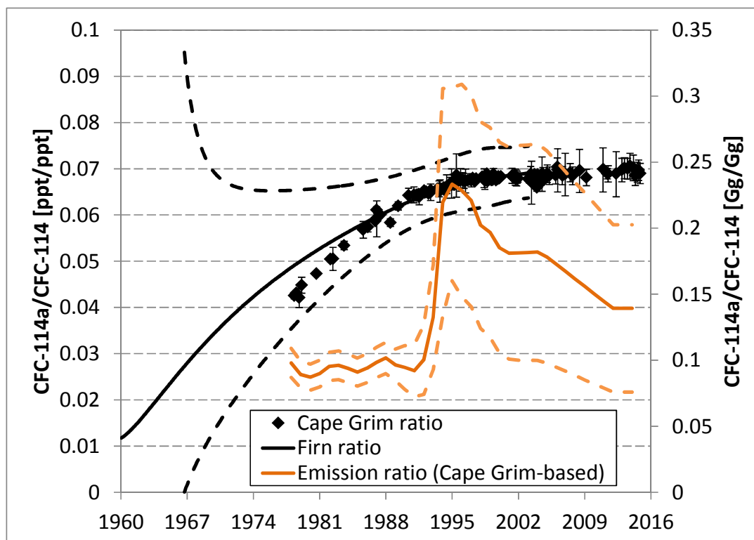
Figure 2: CFC-114a/CFC-114 ratio of mixing ratios at Cape Grim (left axis, black diamonds) and derived from Antarctic firn (left axis, black line), as well as the ratio of their emissions derived from these observations (right axis, orange line). Uncertainties of those ratios are calculated from the uncertainties of mixing ratios (Figure 1) and emissions (Figure 3) and using the equation for combining errors in quotients.
