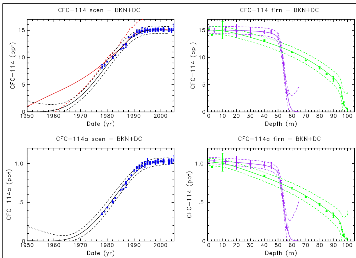
Figure S1: Mixing ratios of CFC-114 and CFC-114a measured in firn air collected at the Berkner (BKN, purple dots) and Dome C (DC, green dots) Antarctic sites, the modelled firn profiles (green and purple lines) and resulting atmospheric time series (black lines) compared to Cape Grim air archive data (blue dots). For CFC-114, the atmospheric trends from Sturrock et al. (2002) (firn air based, red dashed line) and Martinerie et al. (2009) (AFEAS emissions based, red continuous line) are also shown.
