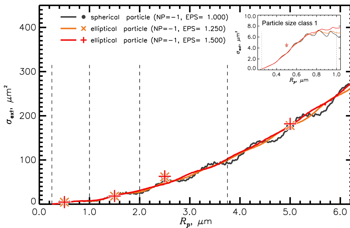
Figure 10. The same as Fig. 8 but for two oblate ellipsoids (orange and red lines).
