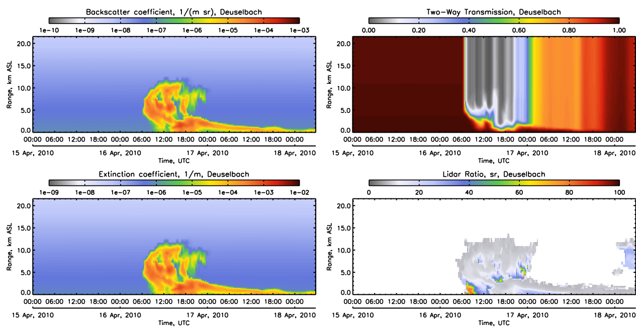
Figure 17. Time-height cross section of backscatter coefficient, two-way transmission, total extinction coefficient and lidar ratio, calculated by the forward model based on COSMO-ART output at the station Deuselbach (West Germany). The forward model represents clean air molecules and volcanic ash particles (no clouds, rain, fog, background aerosol or other scattering objects).
