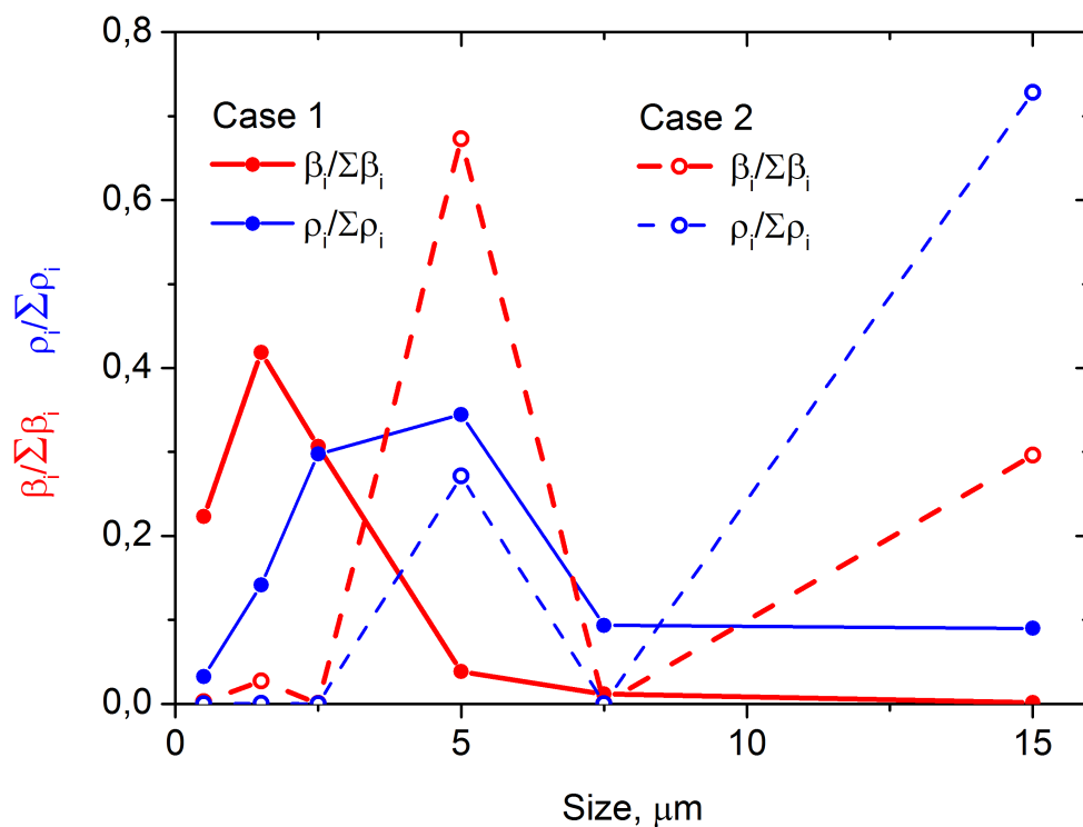
Figure 16. Relative contribution of the 6 volcanic ash size classes to the total backscatter coefficient (red) and to the total mass density (blue) for case 1 (solid) and case 2 (dashed lines). The data are based upon data in Table 4 and Table 5.
