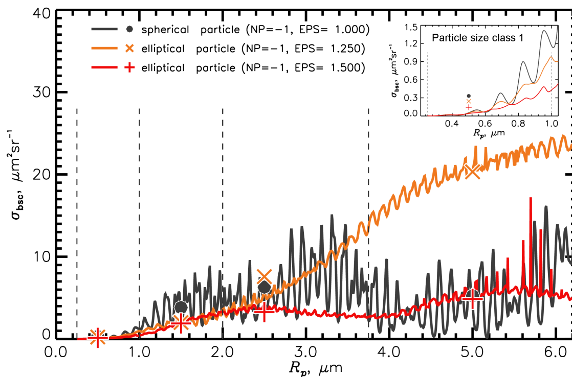
Figure 11. The same as Fig. 10 but for the backscatter cross sections.
