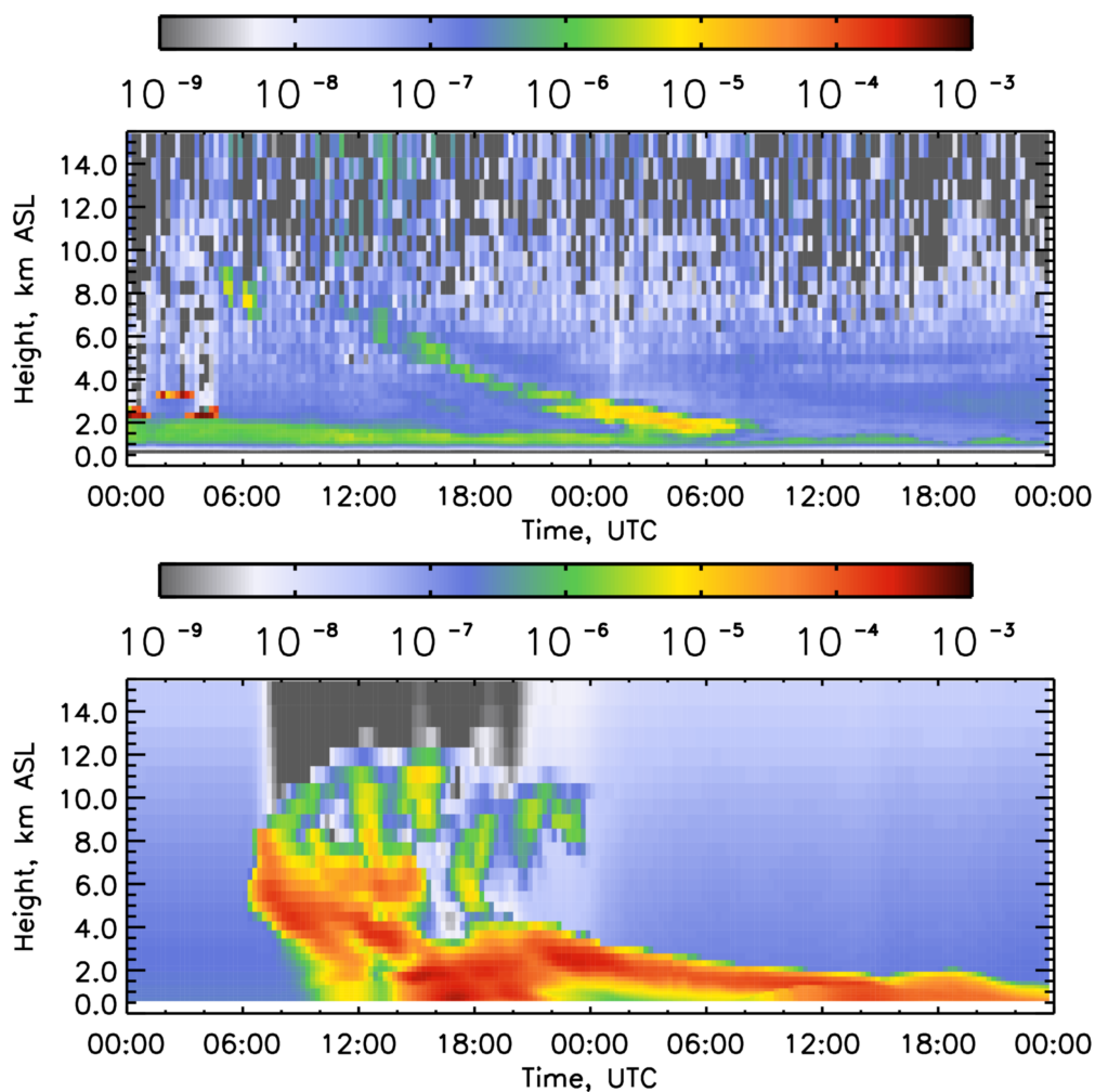
Figure 18. Attenuated backscatter coefficient of ceilometer (top) and forward model (bottom) at the station Deuselbach in Germany from the 16th of April 2010, 00:00 UTC to the 17th of April 2010, 24:00 UTC. The ceilometer data is calculated according to Eq. (27) and averaged according to the model resolution.
