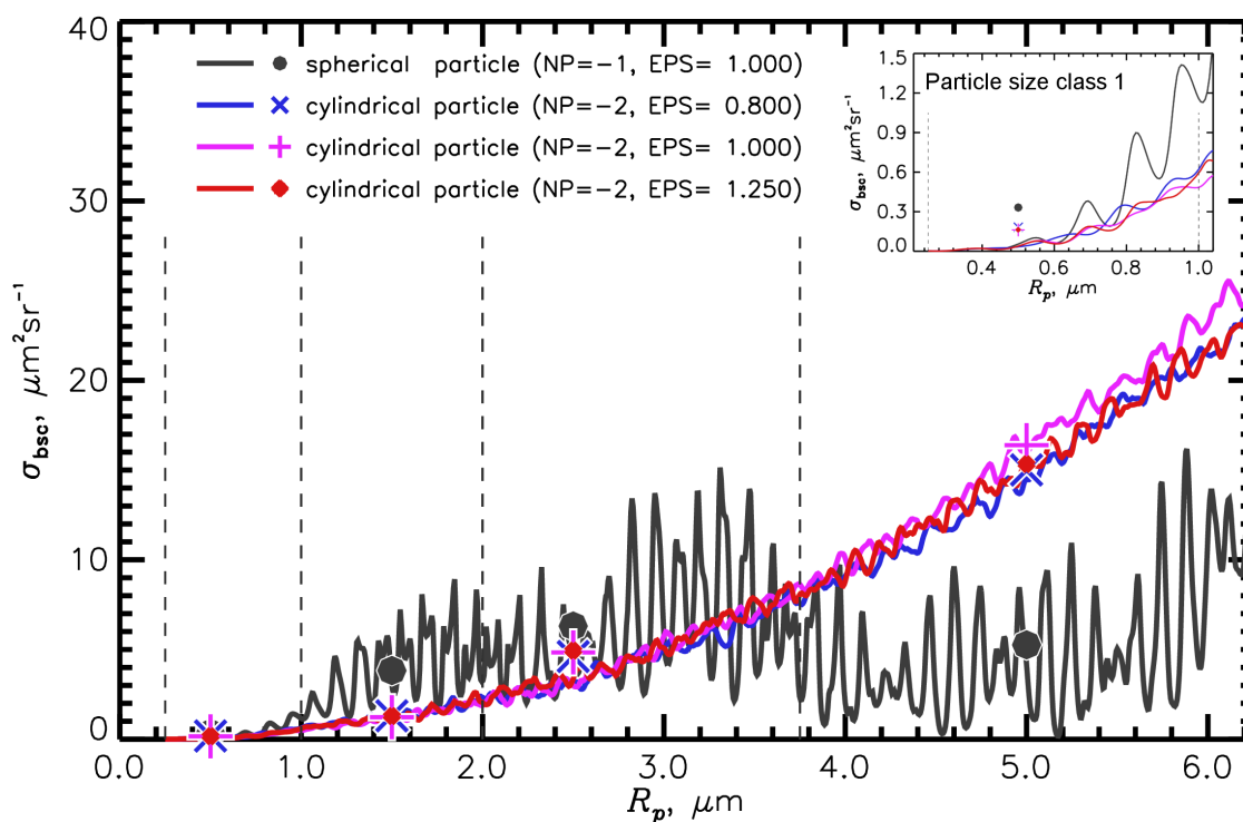
Figure 13. The same as Fig. 12 but for the backscatter cross sections.
