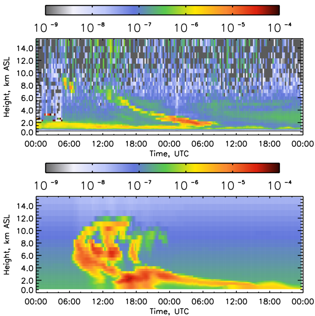
Figure 19. The same as Fig. 18 with a decreased volcanic ash number density. For this purpose, the ash number density predicted by COSMO-ART was reduced by factor 20 before applying the forward operator.
