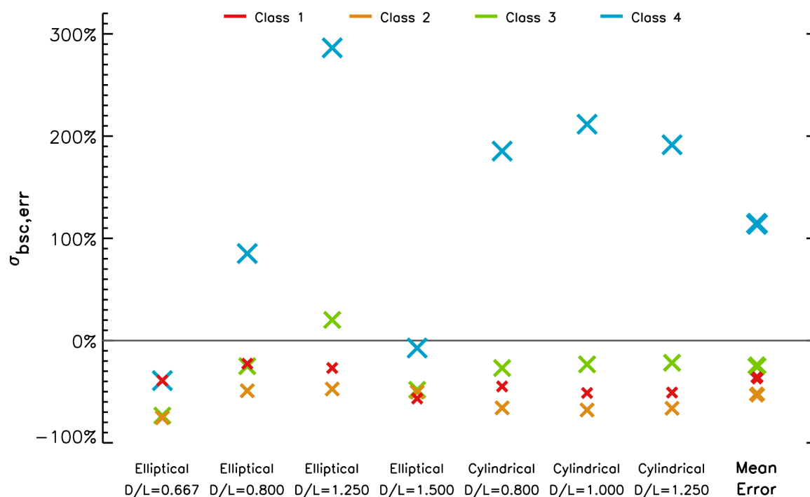
Figure 15. The same as Fig. 14 but for the backscatter cross sections. The mean error is the average relative error of all considered shapes on this plot.
