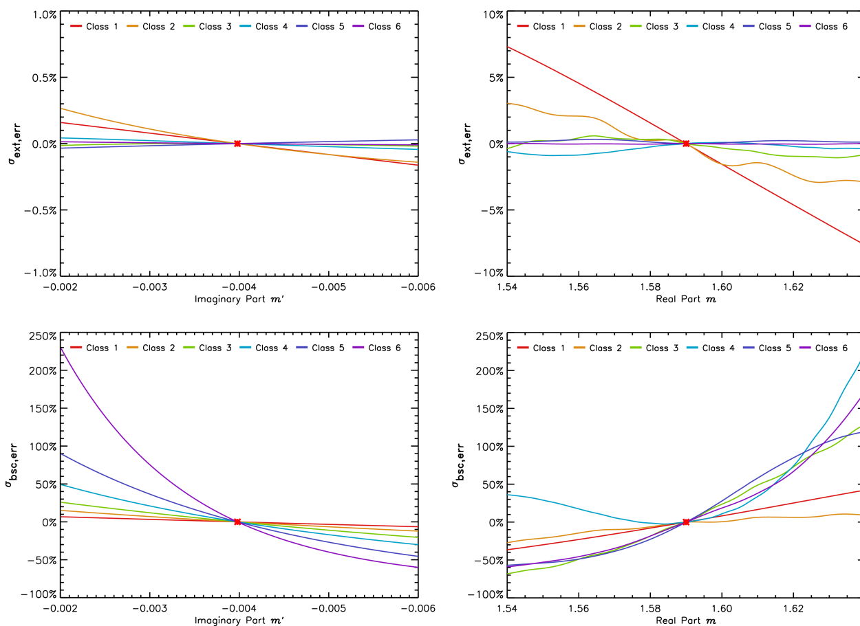
Figure 7. Relative errors of the effective extinction cross section (top row) and of the effective backscatter cross section (bottom row) if the assumed reference refractive index (red dot) is not equal to the true refractive index. Plots in the left row show the error for variable imaginary parts; plots in the right row for variable real parts of the refractive index. Uncertainties of the imaginary part may lead to a maximum error of 0.5% for the effective extinction cross section and of 230% for the backscatter cross section. Uncertain real parts also may lead to errors of 7% for the extinction cross section as well as of 225% for the backscatter cross section in the worst case.
