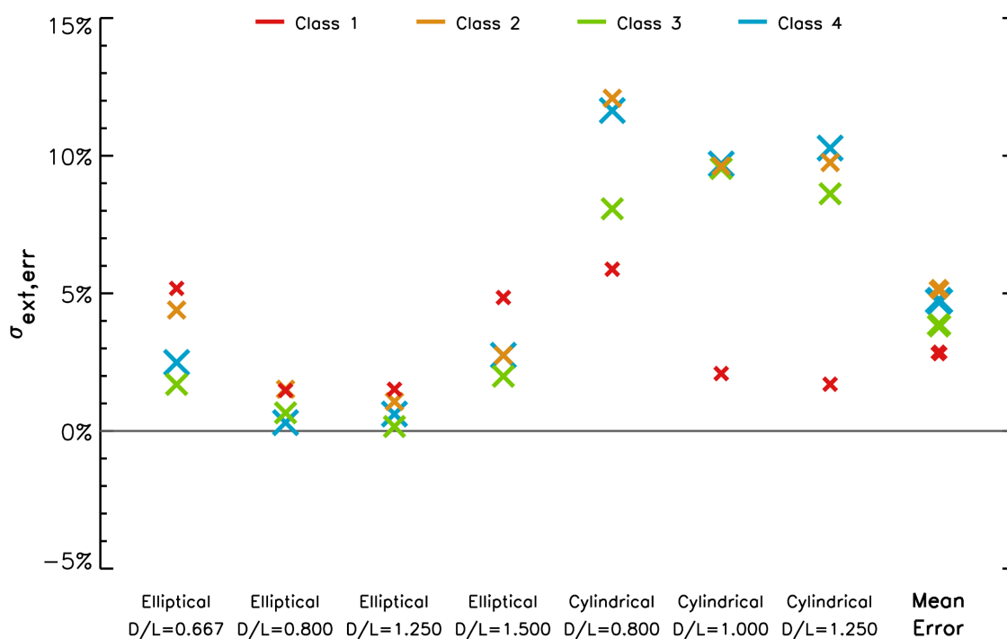
Figure 14. Relative errors of the effective extinction cross section if spherical particles are assumed but the real particles are of elliptical, cylindrical, or of mixed shape. The mean relative error of the analyzed particle shapes does not exceed 6% for the effective extinction cross section.
