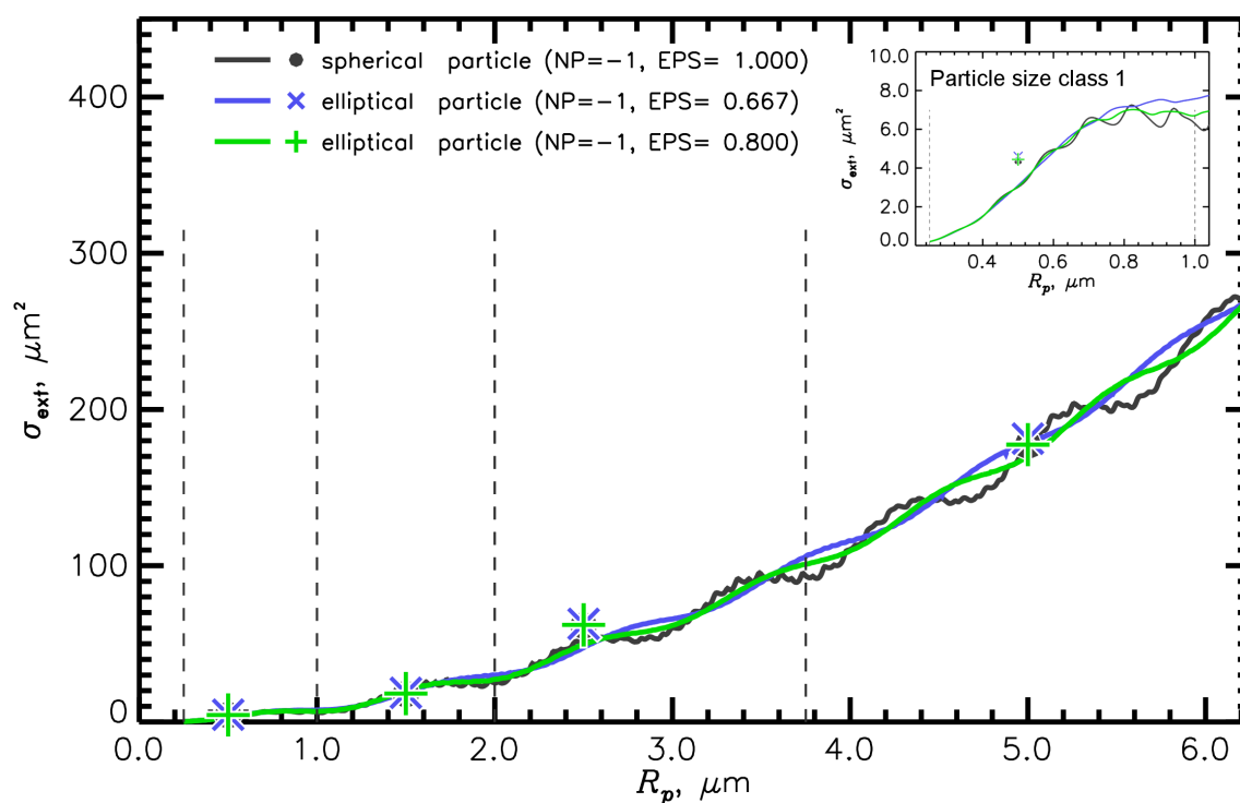
Figure 8. Extinction cross section spectrum for spheres (black line, EPS=1) and two prolate ellipsoids (blue and green line) given as equal-volume radius R_p . The dashed lines indicate the size-margins of each class and the symbols are the effective values of each size class.
