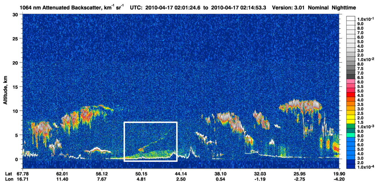
Figure 3. Attenuated backscatter coefficient measurement from CALIOP which was used to calibrate the ACL measurement during the Eyjafjallajökull eruption phase. The volcanic ash cloud is visible around 50.15° lat and 4.81° lon. Image obtained from http://www-calipso.larc.nasa.gov/
