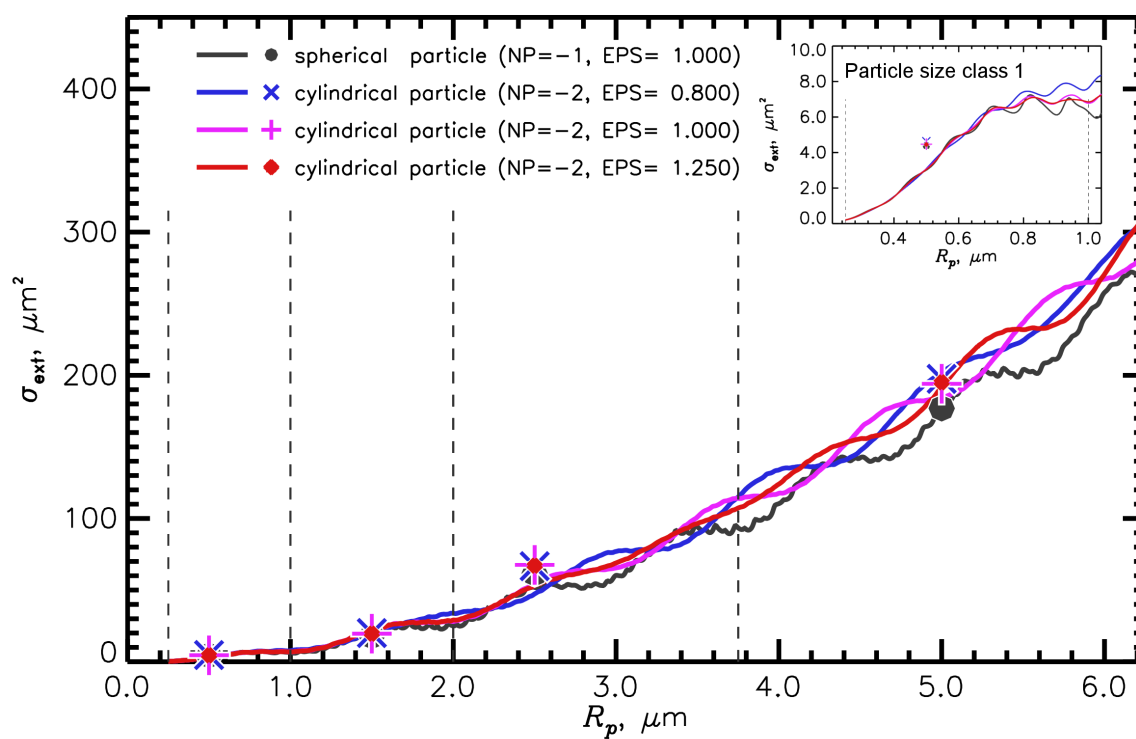
Figure 12. The same as Fig. 8 and Fig. 10 but for three types of cylindrical particles (blue, purple and red line).
