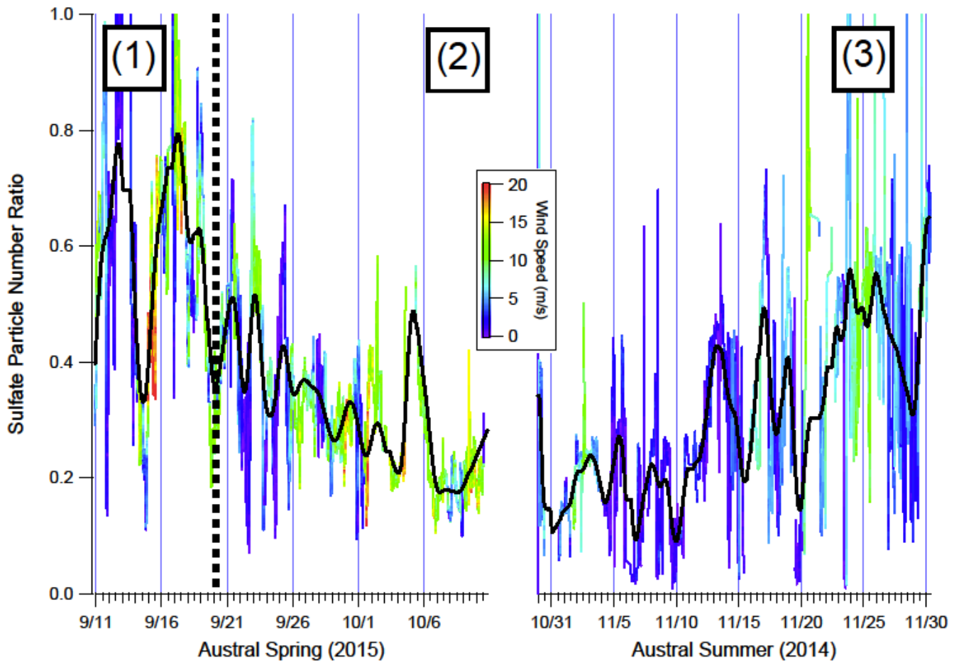
Figure 4: Sulfate number ratio as calculated from the AMS PToF mode divided by the total number concentration from the EPC over both 2014 (right) and 2015 (left). Both field seasons data are colored by recorded wind speeds. A smoothed trace of only wind speeds < 8m/s is overlaid in black. Rough timing for the phases discussed in section 3.2 are noted.
