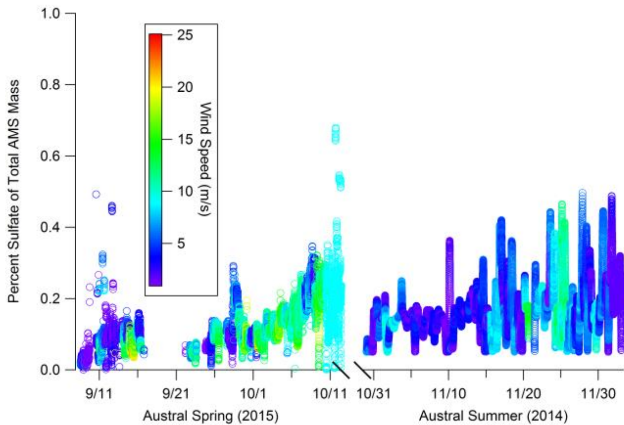
Figure A1: Mass of sulfate as a percent of total non-refractory mass measured in the AMS, colored as a function of wind speed, for both field seasons.
