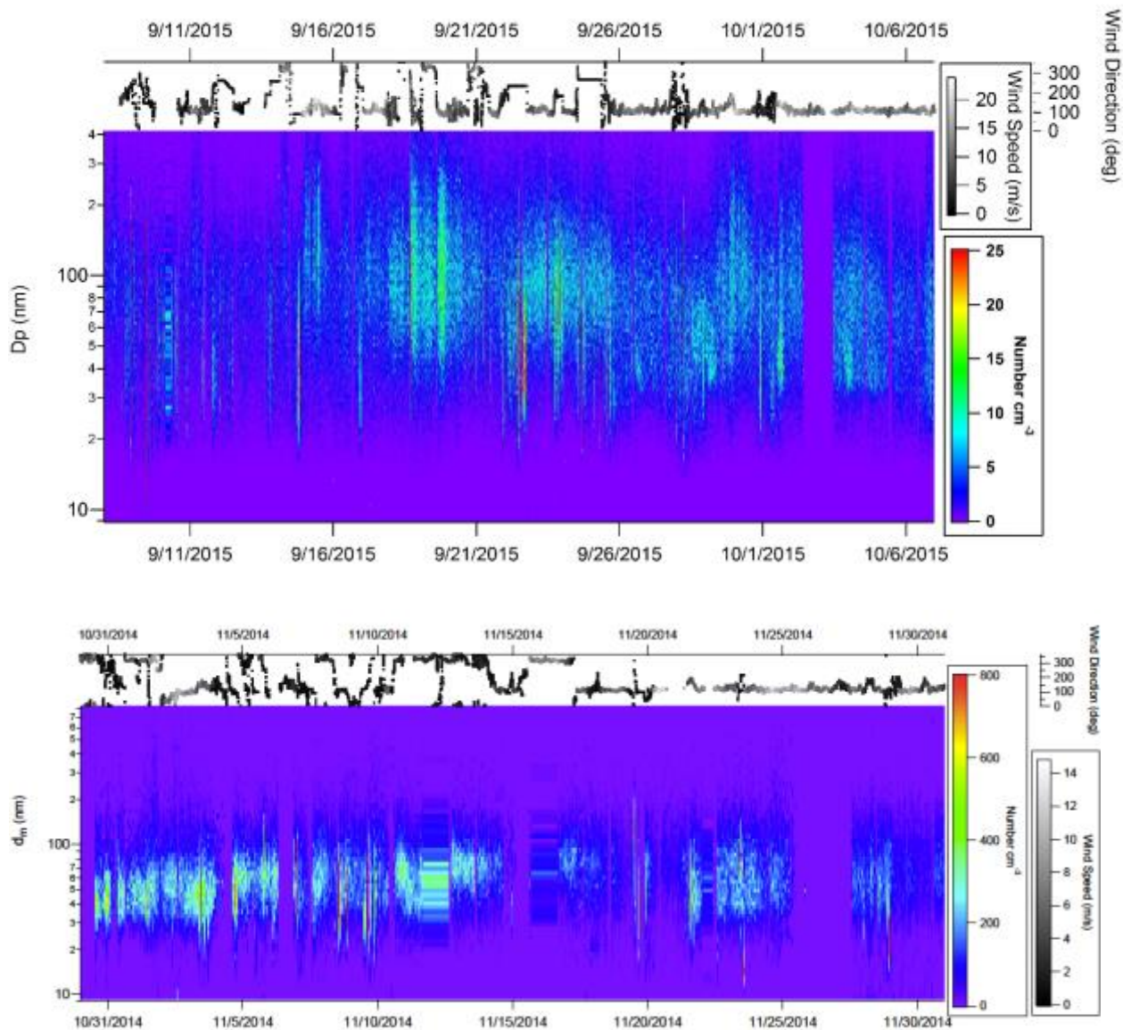
5 Figure A3: dN/d\log D_p image plots from the particle sizing instruments for the 2015 (a, SMPS) and 2014 (b, SEMS) field seasons. Included are the wind speed and direction records. Note that small (20-30nm) particle enhancements only happen during calm wind periods that coincide with elevated m/z 55 concentrations in the AMS (not shown) indicating generator contamination.
