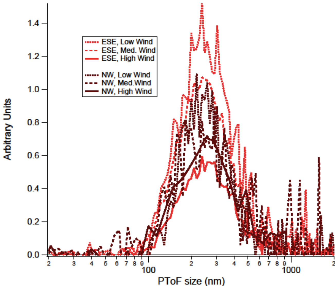
Figure 2: AMS PToF results of AMS sulfate for 2014 as functions of wind speed (solid lines [ > 8\text{ms}^{-1} ] vs dotted lines [ 2\text{-}8\text{ms}^{-1} and <2\text{ms}^{-1} ]) and wind direction (black [Northwest] vs red [East Southeast]). The PToF mass has been arbitrarily scaled to enhance readability of the figure. The PToF results for 2015 are identical in both distribution shape and peak location for all wind regimes.
