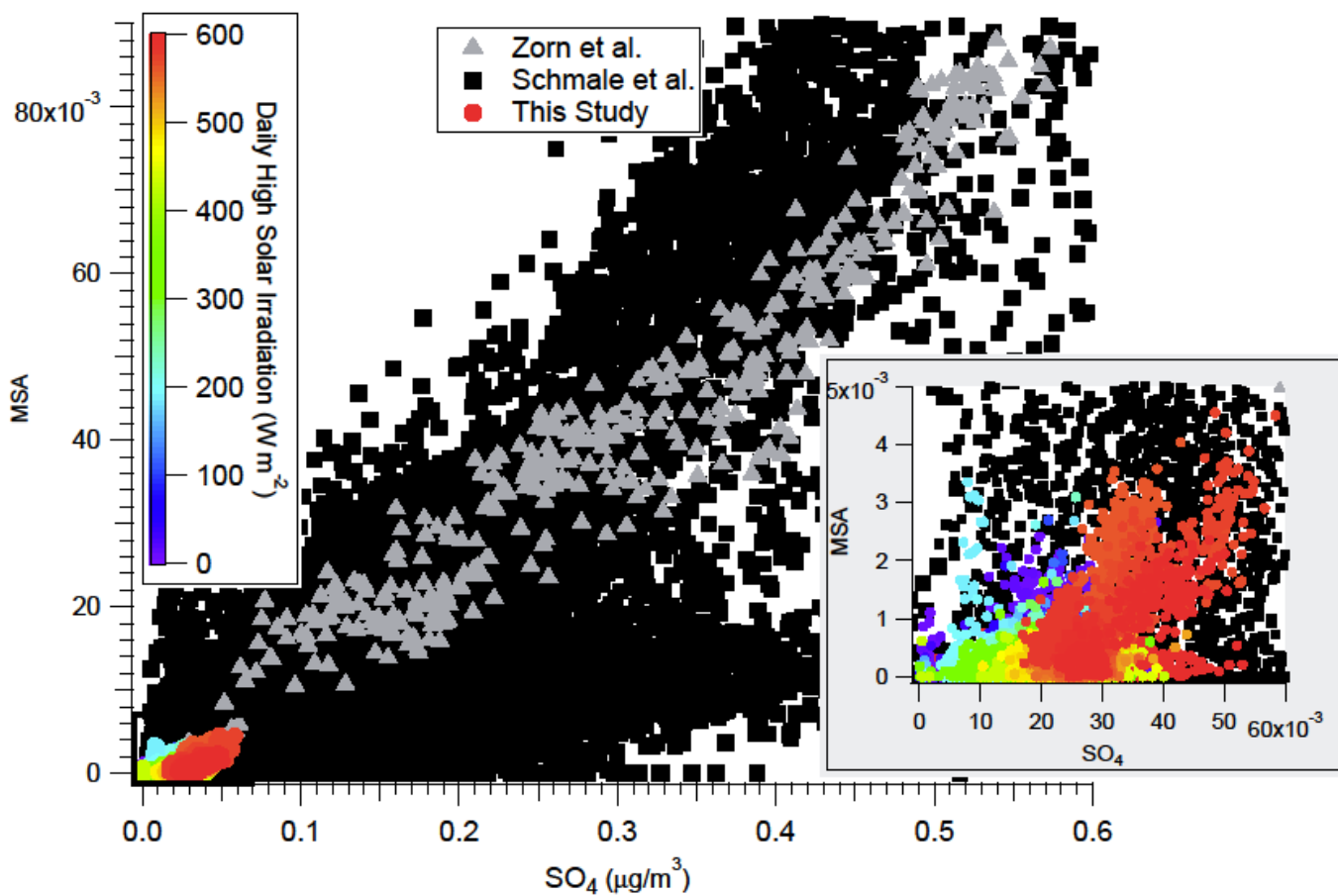
Figure 5: MSA vs sulfate as measured by the AMS for both field seasons, colored by the daily high solar irradiance. 20DIAC data is presented with results from Zorn et al. (2008) and Schmale et al. (2013) for context. Inset is a zoomed in area showing the 20DIAC data in higher detail.
