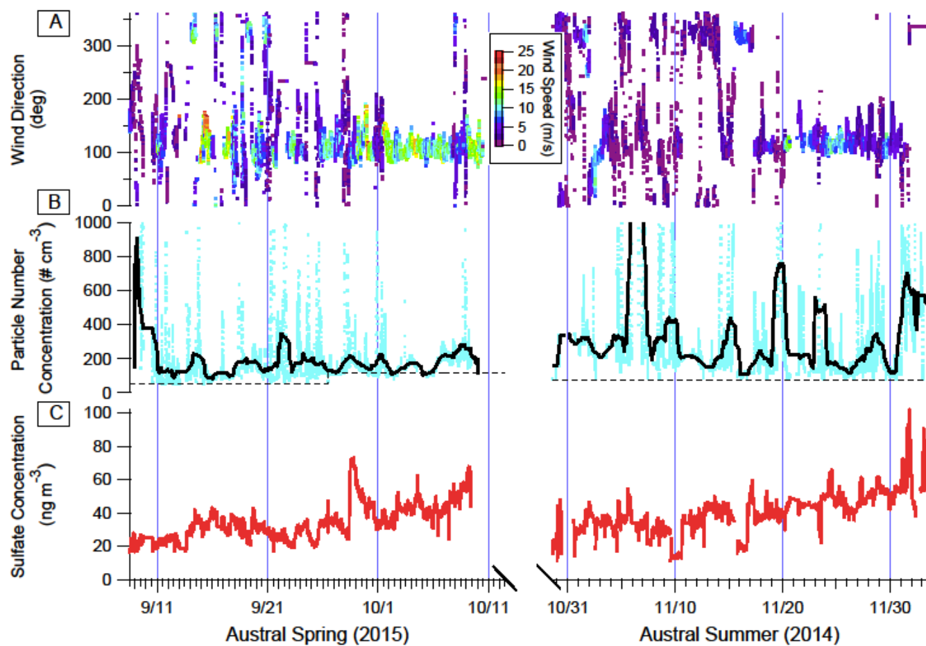
Figure 1: For both the 2014 and 2015 field seasons, with 2015 leftmost: A) Wind direction record colored as a function of wind speed, displayed as a 2-minute average record (standard deviation 0.2 ms -1 and 2 degrees) B) 2-minute (light blue; standard deviation of 11 and 18 # cm -3 for 2015 and 2014, respectively) and 1-hour (black) records of particle number concentration from the EPC, C) 2-minute records of sulfate concentration from the aerosol mass spectrometer. Dotted lines on (B) indicate the minimums in particle number concentrations (99 th percentile) measured over the field seasons.
