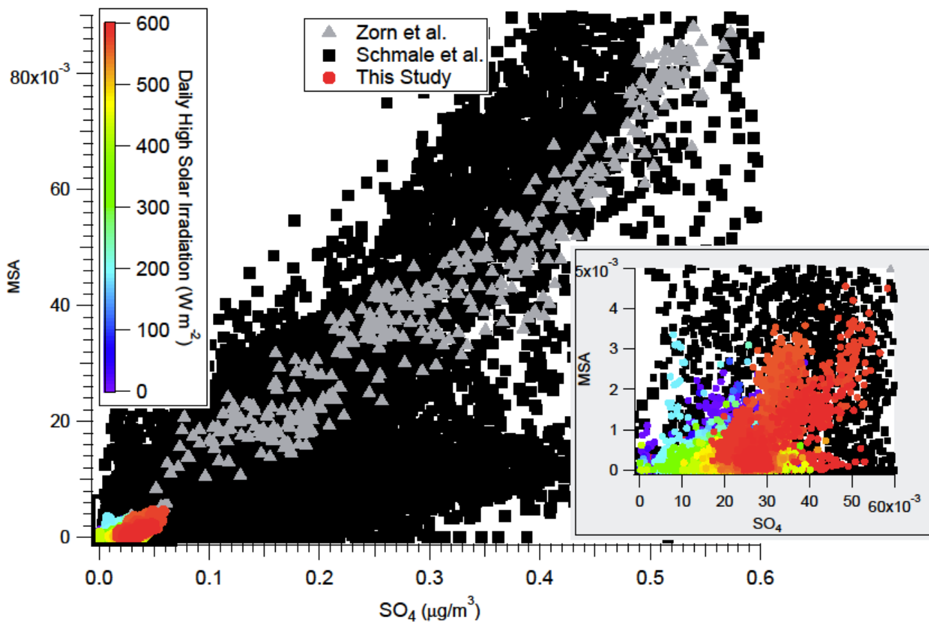
5 Figure 5: MSA vs sulfate as measured by the AMS for both field seasons, colored by the daily high solar irradiance. 2ODIAC data is presented with results from Zorn et al. (2008) and Schmale et al. (2013) for context. Inset is a zoomed in area showing the 2ODIAC data in higher detail.
