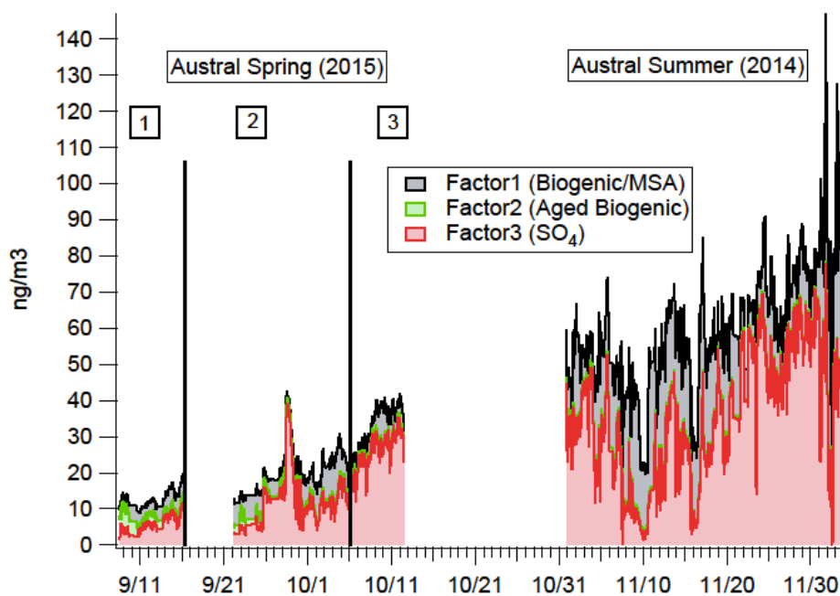
Figure 6: PMF results for the sulfur containing species observed over both field seasons. A) Mass concentration reconstructions in ng/m 3 for each factor and B) the mass spectral fingerprints for each of the 3 factors.
