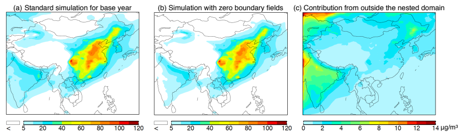
Figure 1 Contributions from outside the nested domain
