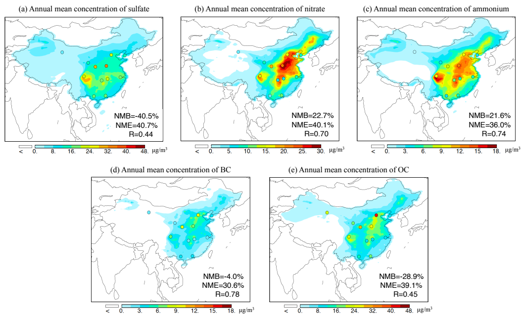
Figure 2 Comparisons of simulated \text{PM}_{2.5} composition with observation averaged during 2012-2013
