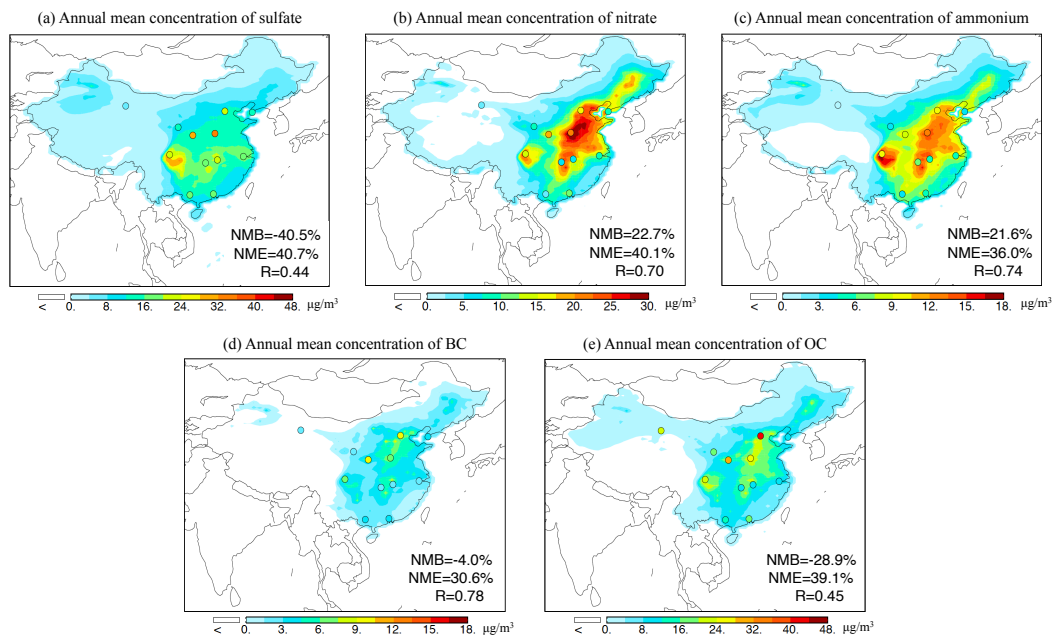
Figure 1 Comparisons of simulated PM_{2.5} composition with observation averaged during 2012-2013
