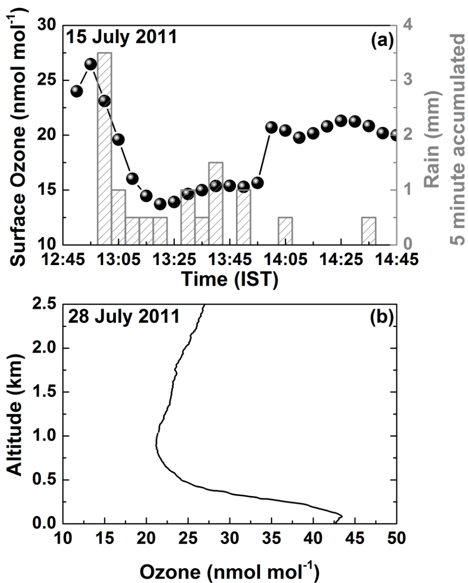
805 Figure 9. (a) Temporal variation in surface O 3 mixing ratio (black dots) along with 5-minute accumulated rainfall (grey vertical bars) over Thumba, Thiruvananthapuram (location of the site shown in Fig. 1 and 2) on 15 July 2011. (b) Vertical profile of O 3 mixing ratio over Thumba, Thiruvananthapuram as measured on 28 July 2011.
