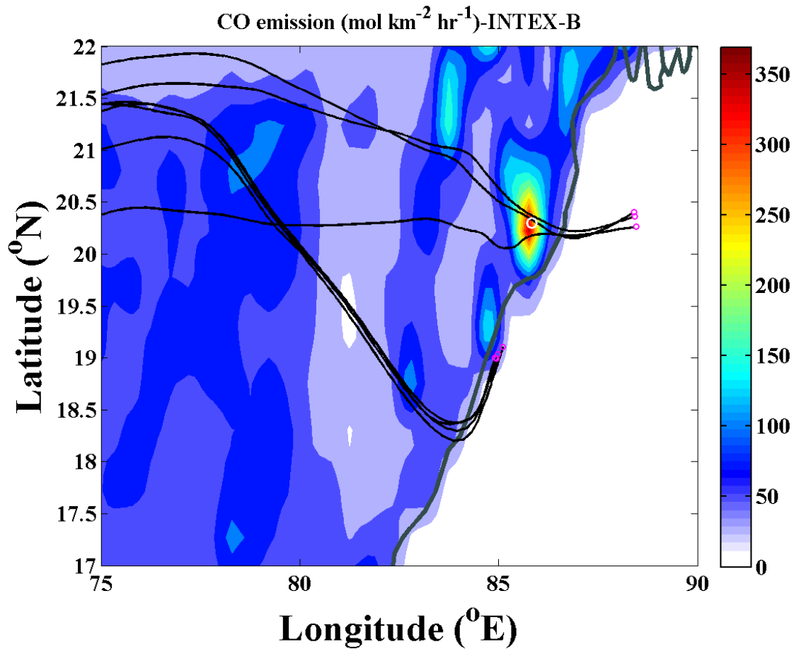
780 Figure 5. Backward air mass trajectories (black curves) 500 m above the location of higher CO observations as marked by red arrows in Fig. 5b during August 7 and 11, 2009. The background colour map shows the spatial distribution of anthropogenic CO emissions over the Indian region for the year 2006 from INTEX-B inventory. The small circles in magenta represent the points where observations were made, as well as the end-point of trajectories. The white circle over the hot-spot region denotes an observational site, Bhubaneswar.
