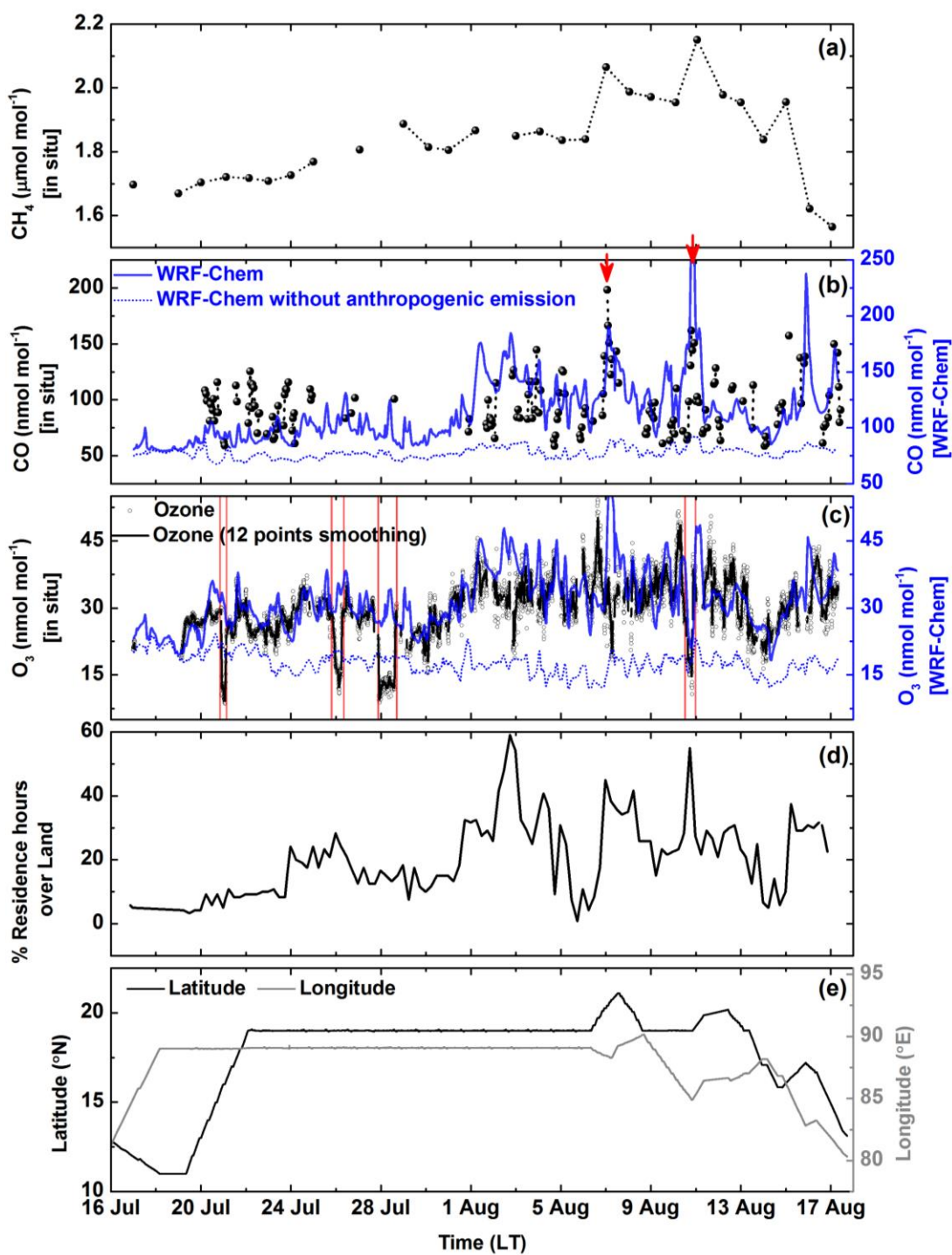
775 Figure 4. Variations in observed CH 4 (a), CO (b), O 3 (c), and percentage residence time over land (d) along with WRF-chem simulated O 3 and CO (blue line) during the campaign. Events of sharp decrease in O 3 during rainfall are marked by vertical red lines (Fig. 8). (e) Variations in measurement locations.
