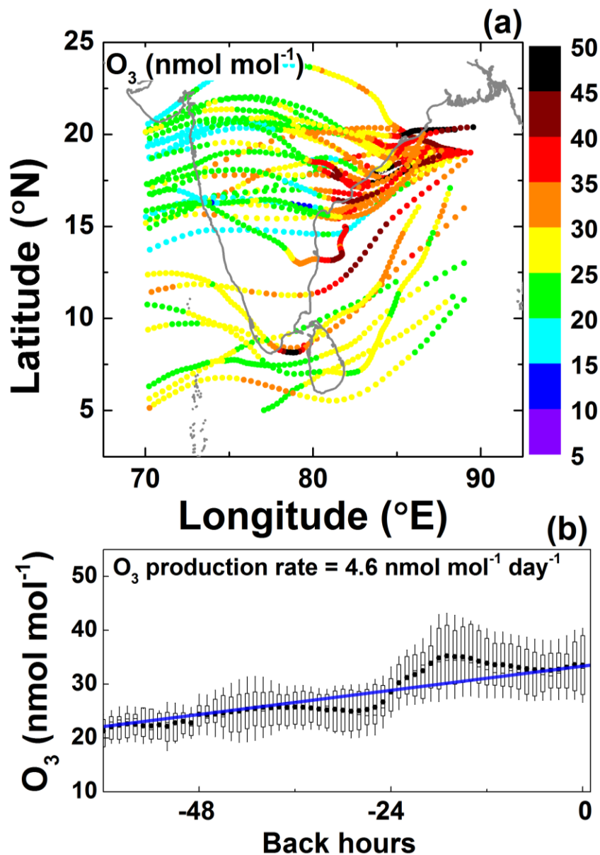
795 Figure 7. (a) WRF-Chem simulated O_3 along the air mass trajectories ending over a few representative locations over the BoB. (b) Variation of O_3 mixing ratios with time along the trajectories as shown in 7a. In box plot, the black dots and lines inside the box represent the mean and median of the data respectively. While the lower and upper edges of boxes represent the 25 th and 75 th percentiles respectively, the whiskers represent standard deviations.
