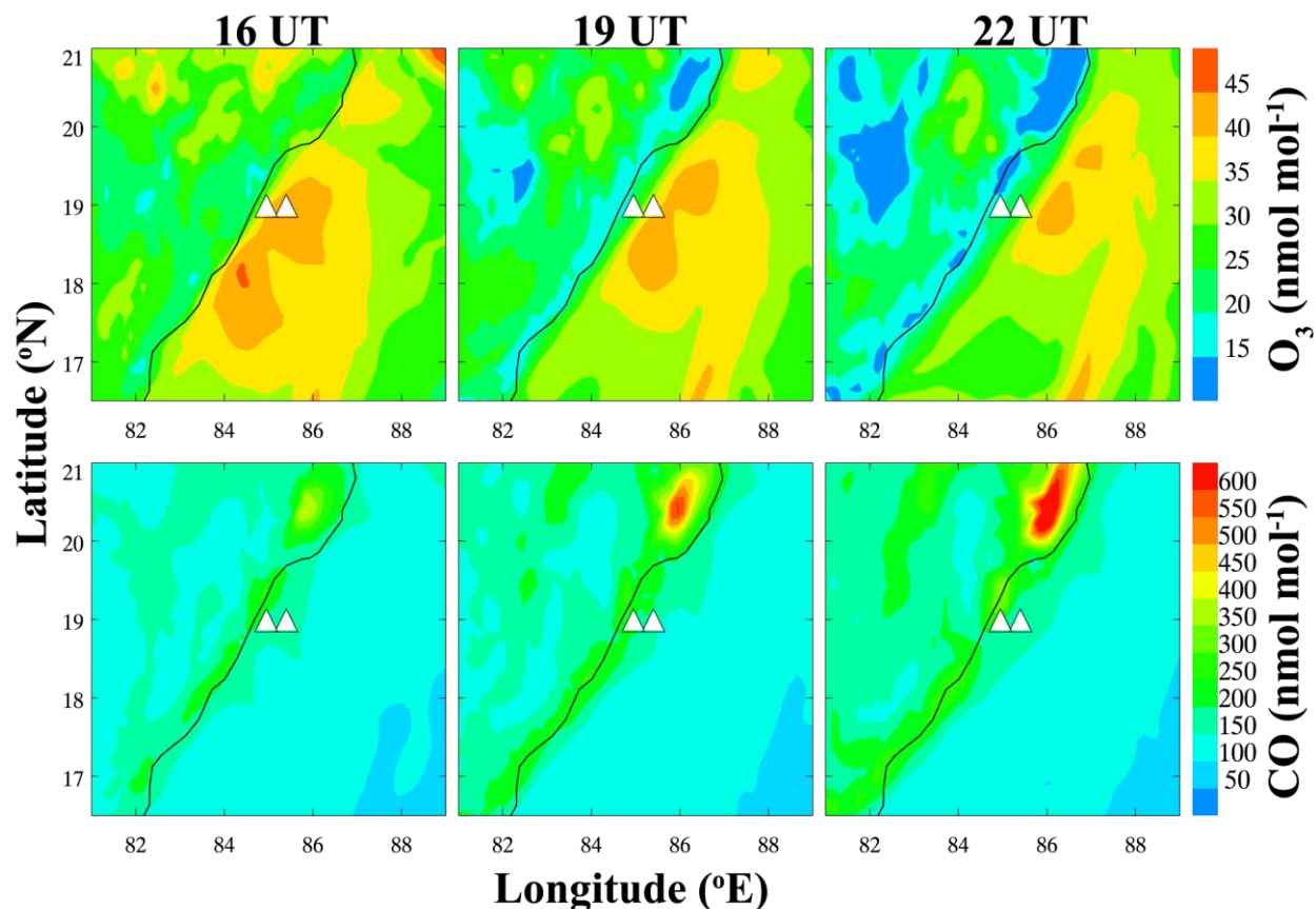
820 Figure 11. Spatial distribution of surface O_3 (top panel) and CO (bottom panel) at 16:00 UT and 19:00 UT on August 10, 2009, both prior to and during the fourth event, which took place 22:00 UT on August 10, 2009. White triangles show two locations ( 85.40^{\circ} E, 19.00^{\circ} N; 84.95^{\circ} E, 19.00^{\circ} N) corresponding to the event.
