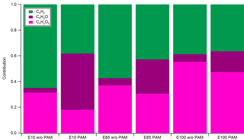
Figure 5. Contribution of different organic fragments with and without PAM chamber. CH refers to hydrocarbons (C x H y ); CHO to fragments with one oxygen atom (C x H y O z + ) and CHO x to compounds containing several oxygen atoms (C x H y O z , z>1).
