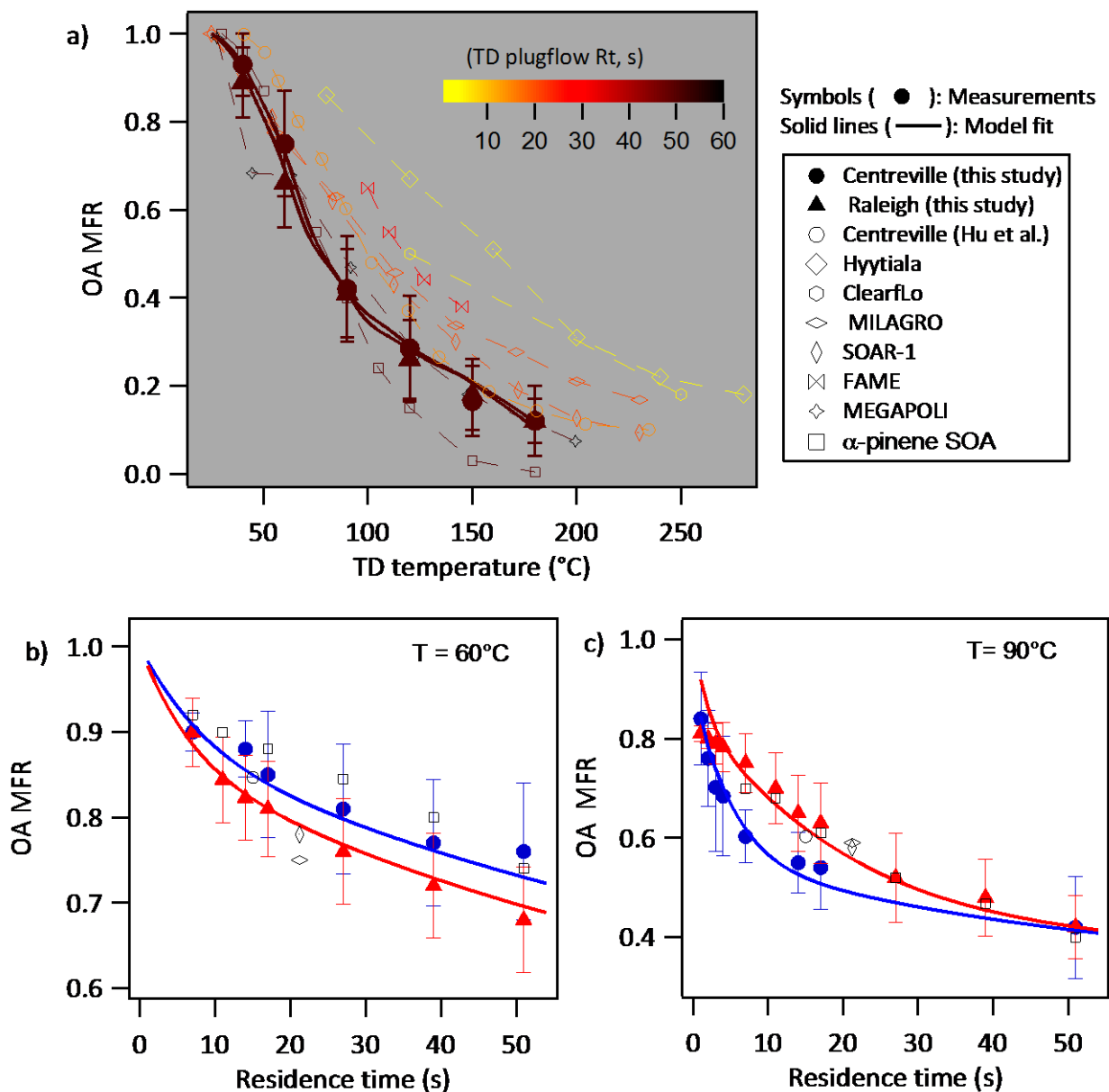
Figure 2: Measured (solid symbols) and modeled (solid thick lines) campaign average organic aerosol (OA) mass fraction remaining (MFR) as a function of TD temperatures ( T ) and residence times ( Rt ). The solid symbol shows mean value and error bar is \pm one standard deviation of all campaign data at each ( T , Rt ) condition. Raw data at each ( T , Rt ) condition are averaged over 20-30 minutes. Model lines are shown using the 'best fit' volatility parameter values from campaign average TD data fit (parameter values listed in Table 1). TD measurement data from the Centreville site collected by the University of Colorado group at SOAS-2013 (Hu et al., 2016) are also shown. Measurements from several previous field studies are shown with various open symbols: Hyytiälä/2008-2010, Finland (Häkkinen et al., 2012); ClearLo/2012, London (Xu et al., 2016); MILAGRO/2006, Mexico City (Huffman et al., 2009); SOAR-1/2005, Riverside, California (Huffman et al., 2009); FAME/2008, Finokalia, Greece (Lee et al., 2010); MEGAPOLI/2009-10, Paris, France (Paciga et al., 2015). Chamber alpha-pinene SOA (dark ozonolysis, COA \sim 5 \mu\text{g m}^{-3} , VMD \sim 140 \text{ nm} ) evaporation data are shown from Saha and Grieshop (2016). In panel-a, data are
