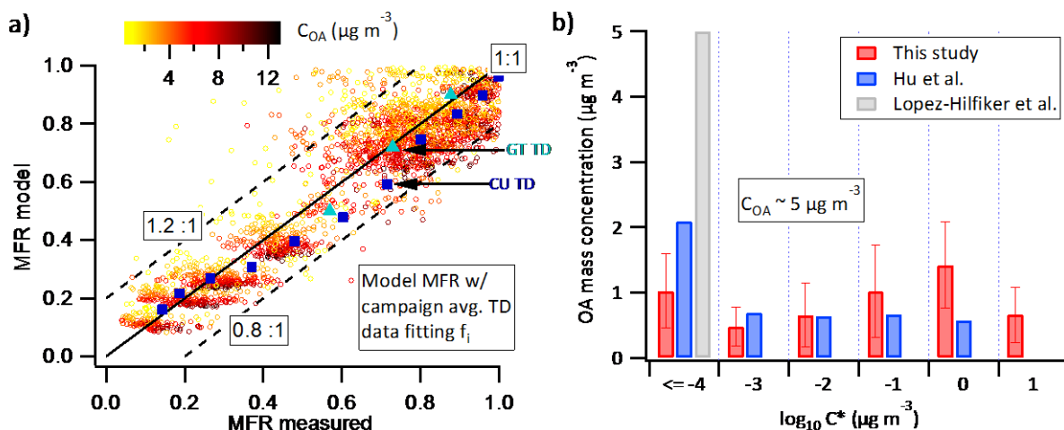
Figure 4: (a) Comparison of individual observations from the Centreville campaign and corresponding modeled MFRs applying the extracted f_i distribution from the campaign-average fit. MFR data collected by other groups during the Centreville campaign are also shown: University of Colorado TD (CU TD; blue squares)(Hu et al., 2016) and Georgia-Tech TD (GT TD; cyan triangles) (Cerully et al., 2015) along with corresponding MFRs modeled applying volatility parameterizations from this study with the campaign average C_{OA} and d_p . Fig. S9 shows an extended data figure of panel a, including similar plot using the f_i distribution from the unified fit and analysis results for the Raleigh data set. (b) Comparison of the SOAS campaign-average OA volatility distribution (showing only condensed phase) derived from this study (dual-TDs; kinetic evaporation model fits), Hu et al.(2016) (TD; method of Faulhaber et al.(2009)), and Lopez-Hilfiker et al.(2016) (FIGAERO-CIMS). Error bars on data from this study are \pm one standard deviation of distributions extracted over the campaign period (Fig.6).
