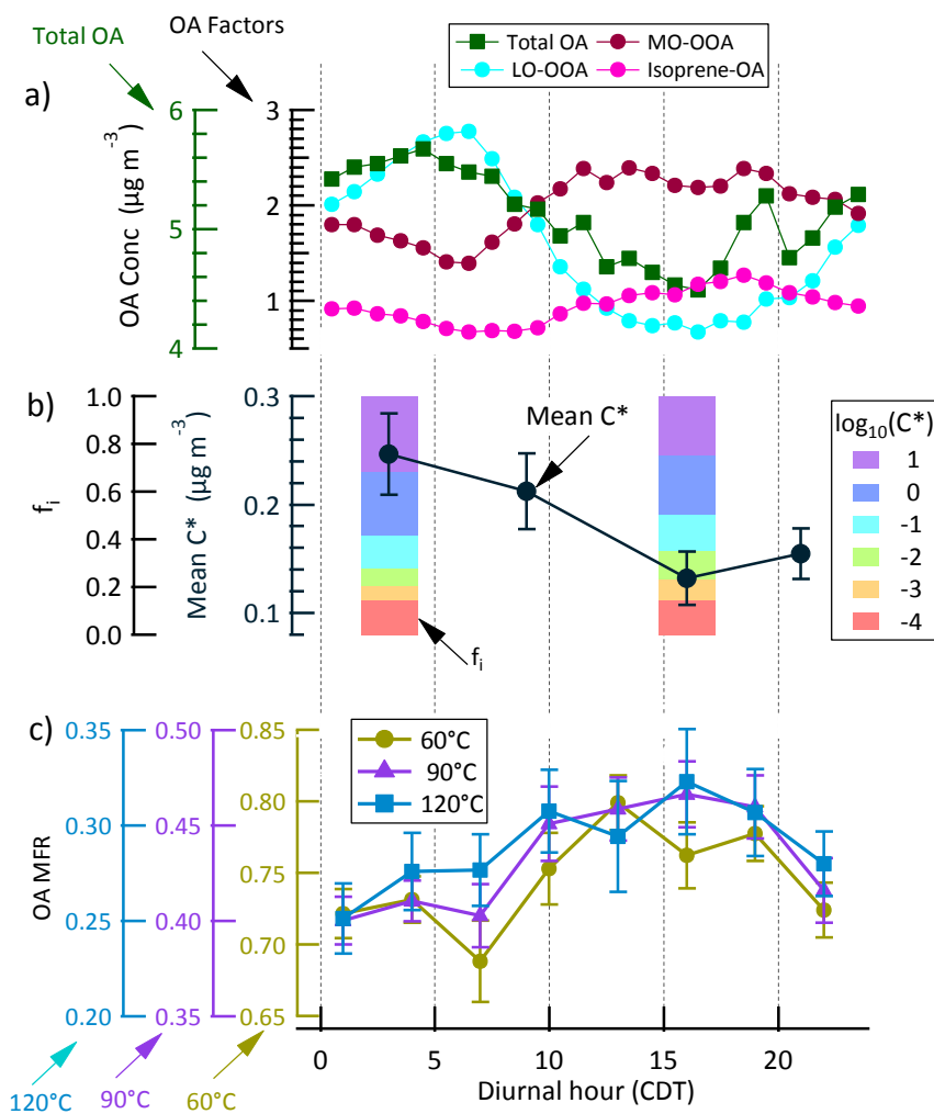
Figure 7: Campaign average diurnal trends for the Centreville measurements of: (a) concentrations of total OA and OA factors, (b) OA volatility ( f_i and \bar{C}^* ), (c) OA MFR after heating at 60, 90 and 120 °C with a TD residence time of 50 s. Fig. S11 shows similar analysis results for the Raleigh data set. PMF factors in panel-a are LO-OOA: less-oxidized oxygenated OA; MO-OOA: more-oxidized oxygenated OA; Isoprene-OA: isoprene-derived OA (for details on OA factors analysis see Xu et al., 2015a, 2015b).
