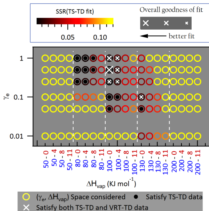
5 Figure 3: Extraction of OA gas-particle partitioning parameter ( \Delta H_{vap} , \gamma_e and f_i ) values via evaporation kinetic model fits to campaign-average dual-TD observations during the Centreville campaign. A relationship of \Delta H_{vap} = \text{intercept} - \text{slope} (\log_{10} C^*) was assumed (e.g., 50-0 on x-axis represents intercept = 50 and slope = 0). Symbols and colors represent the goodness of fit. Points with filled inner circles recreate TS-TD observations and points with a white cross (x) recreate both TD data sets to within observational variability. Crosses represent the overall goodness of fit including both TS-TD and VRT-TD observations, with larger size corresponding to a better fit.
