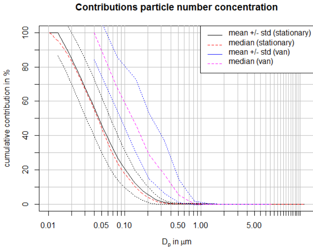
Fig. 1. Cumulative contribution to total particle number concentration above 10 nm in particle diameter starting at the largest size of 20 micron. Displayed are two datasets, i.e. (a) based on the stationary
