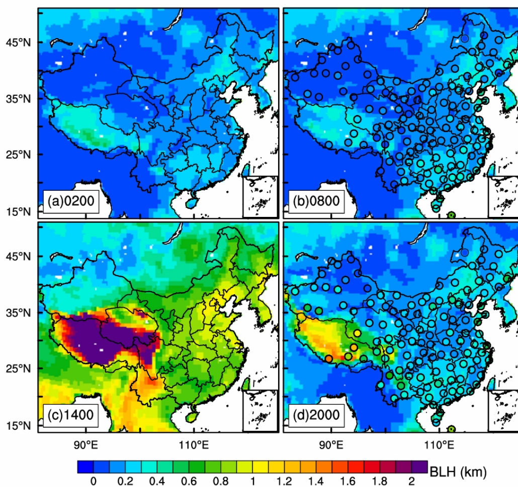
Figure S3. Similar as Figure S5, but for spatial distributions of BLHs in winter.
