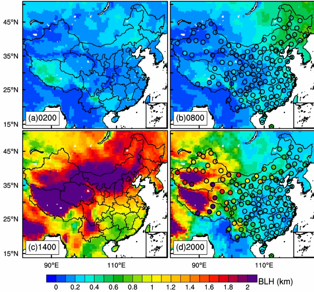
Figure S1. Spatial distributions of seasonally averaged ERA-BLH (color shaded) and CMA-BLH (color dots) at (a) 0200 BJT, (b) 0800 BJT, (c) 1400 BJT, and (d) 2000 BJT in spring.
