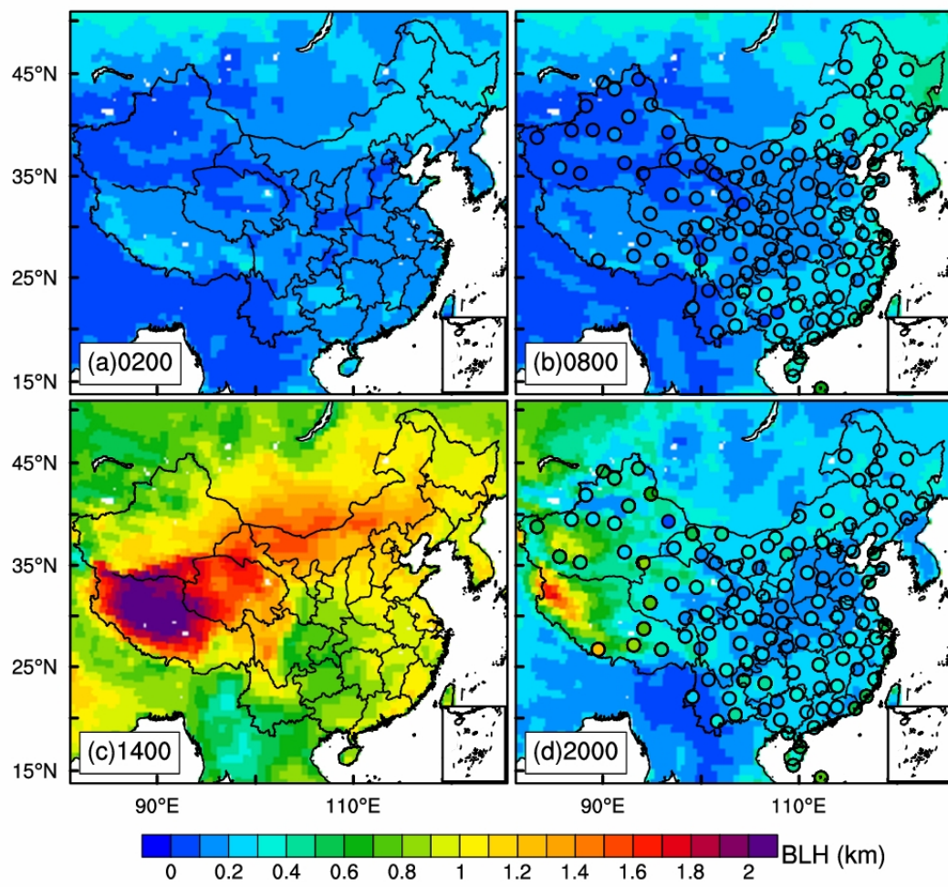
Figure S2. Similar as Figure S5, but for spatial distributions of BLHs in fall.
