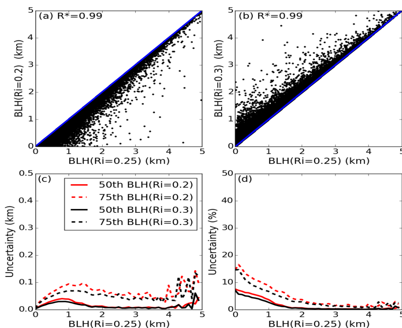
Figure 3. Scatter plots showing (a) CMA-BLHs computed using 0.2 and 0.25 as critical R_i , and (b) CMA-BLHs computed using 0.25 and 0.3 as critical R_i , both of which are based on 391552 soundings across China from January 2011 to July 2015. The 50th and 75th percentile values of (c) absolute uncertainty and (d) relative uncertainty using 0.2 and 0.3 as critical R_i are shown as well. The correlation coefficients ( R ) are given in the top panels, where the star superscripts indicate that values are statically significantly ( p < 0.05 ).
