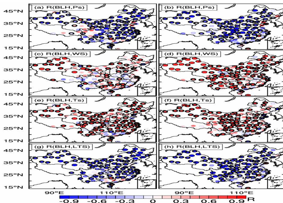
Figure 13. Correlations ( R ) between mean annual cycles (12 monthly values) of CMA-BLH and (a, b) surface pressure (Ps), (c, d) 10-m wind speed, (e, f) near-surface temperature (Ts), (g, h) Lower Tropospheric Stability (LTS), at (left) 0800 and (right) 2000 BJT. Symbols outlined in black indicate values that are statistically significant ( p < 0.05 )
