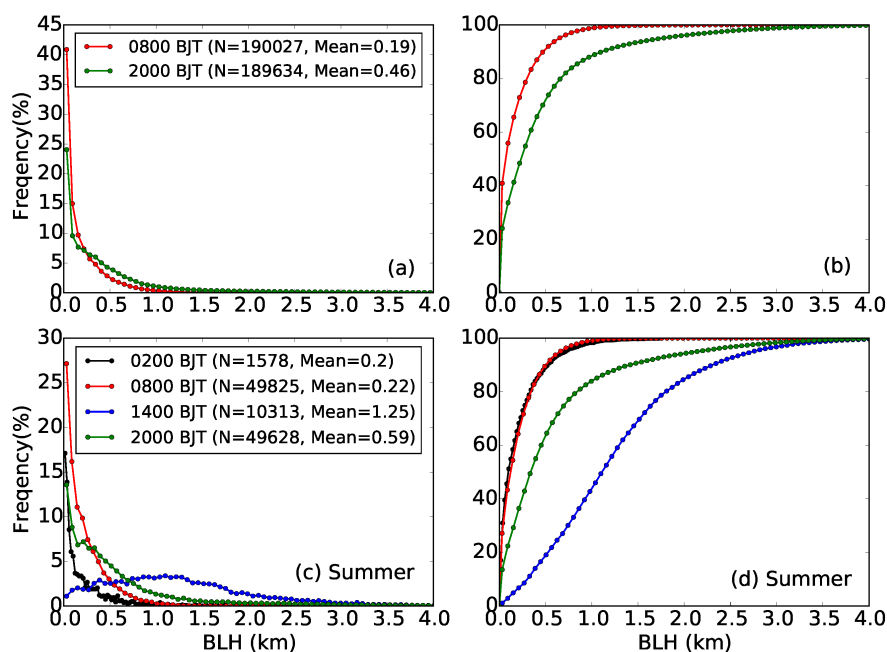
Figure 4. Frequency distribution (left) and cumulative frequency distribution (right) of CMA-BLH at 0200 (in black), 0800 (in red), 1400 (in blue) and 2000 BJT (in green) during (a, b) the whole period and (c, d) the summertime from January 2011 to July 2015. The number of soundings (N) and mean value at each observed time are also given. Noted that the soundings at 0200 and 1400 BJT are occasionally launched during certain intensive observation periods in summer.
