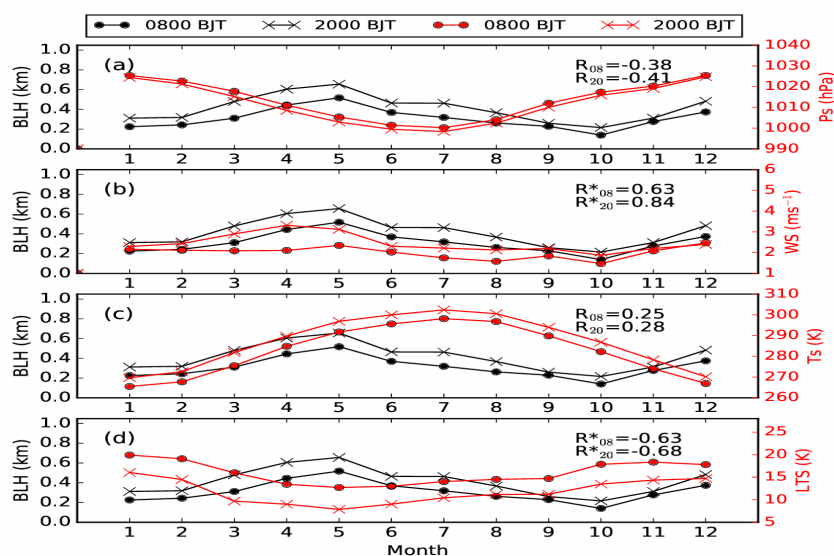
Figure 12. Climatological mean annual cycle of CMA-BLH at Beijing (39.8°N, 116.47°E) at 0800 BJT (dot symbols) and 2000 BJT (x symbols), respectively, as superimposed by the counterparts of meteorological parameters, including (a) surface pressure (Ps), (b) 10-m wind speed (WS), (c) near-surface temperature (Ts), and (d) Lower Tropospheric Stability (LTS). The correlation coefficients at 0800 ( R_{08} ) and 2000 BJT ( R_{20} ) between of CMA-BLH and meteorological parameters are given in each panel as well, and the star superscripts indicate the values that are statistically significant ( p < 0.05 ).
