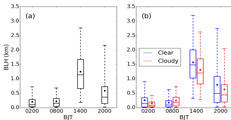
Figure 11. (a) Box-and-whiskers plots showing the 5th, 25th, 50th, 75th, and 95th percentile values of CMA-BLH at 0200, 0800, 1400, and 2000 BJT in summer based on all the summertime soundings in China. (b) Box-and-whiskers plots showing CMA-BLH in summer under clear (total cloud cover \leq 20\% , in blue) and cloudy (total cloud cover \geq 80\% , in red) conditions. Note that the rainy days are not considered in (b).
