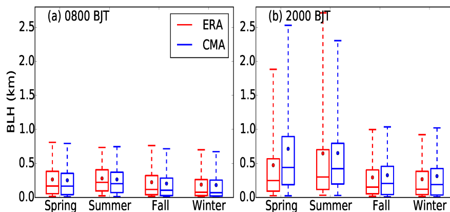
Figure 5. Box-and-whiskers plots showing the 5th, 25th, 50th, 75th, and 95th percentile values of ERA-BLH (in red) and CMA-BLH (in blue) during each season at (a) 0800 BJT and (b) 2000 BJT during the period from January 2011 to July 2015. The dot in the each box indicates the mean value of BLHs. Note that there exists larger uncertainty for the evening BLH climatologies in (b).
