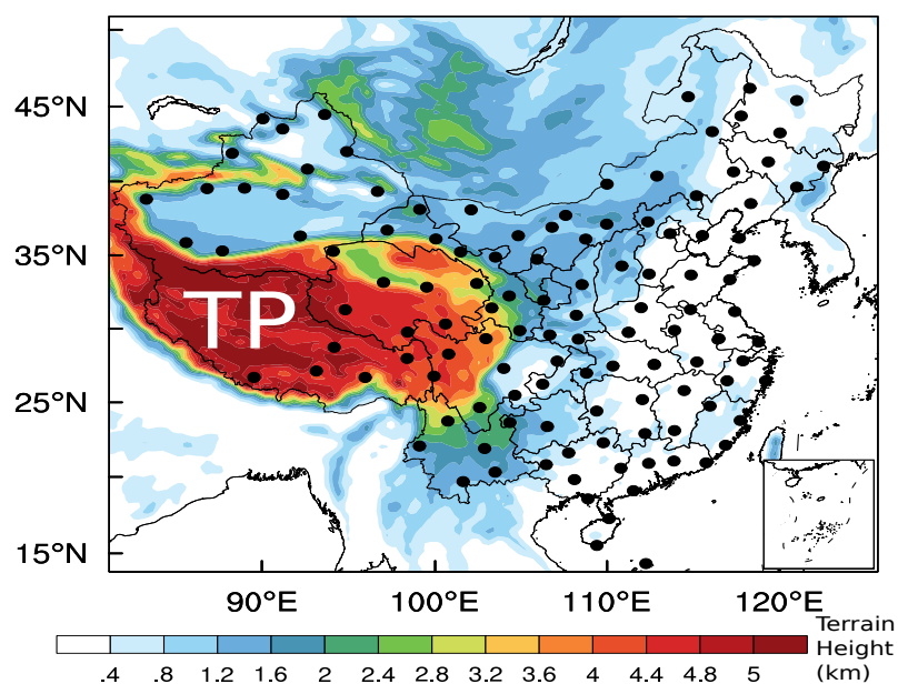
Figure 1. Spatial distribution of CMA sounding sites (black dots), overlaid over the terrain height (color shaded) of China. The white “TP” indicates the location of Tibet Plateau.
