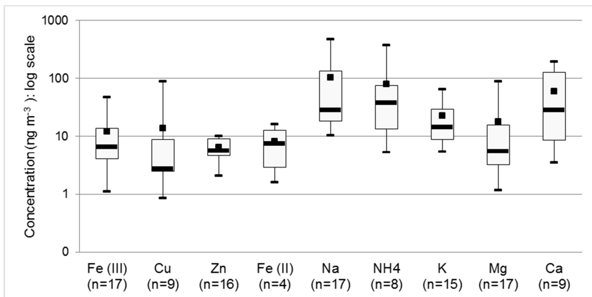
830 Figure 7. Boxplot for the soluble ion and other species concentrations in the total particulate matter samples at 60 m height from 30 March to 25 April 2015. Upper and lower whiskers represent 1.5 interquartile ranges for the period, upper and lower boundaries are for the third and first quartile. The horizontal bar is the median value and the black square is the average value for each element. In the horizontal axis the number of samples with valid results is shown.
