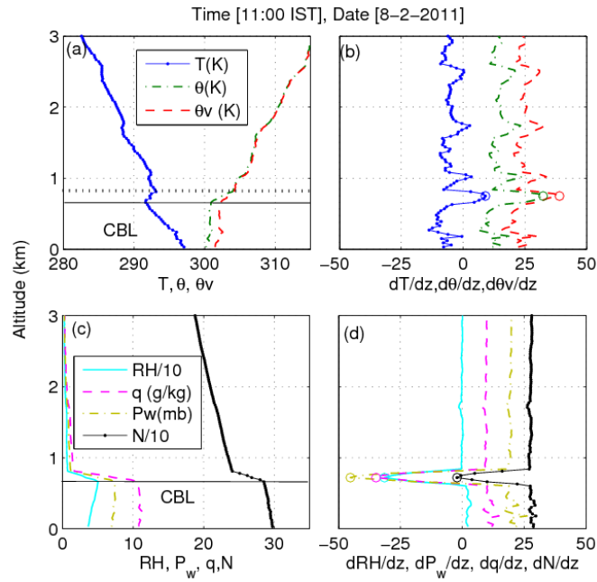
795 Figure 2: Typical profiles of (a) temperature ( T ), potential temperature ( \theta ) and virtual potential temperature ( \theta_v ) and (c) relative humidity (RH), specific humidity ( q ), water vapor pressure ( P_w ), and radio refractivity ( N ) showing convective boundary layer (CBL) using GPS radiosonde observation at 1100 IST on February 8, 2011 over Gadanki (13.45°N, 79.2°E). (b) and (d) show the gradient profiles corresponding to (a) and (c), respectively. Solid horizontal 800 lines in (a) and (c) indicates the base of the inversion layer. Dotted line in (a) indicates the top of the inversion. Open circles in figures (b) and (d) denote the CBL heights above ground level.
