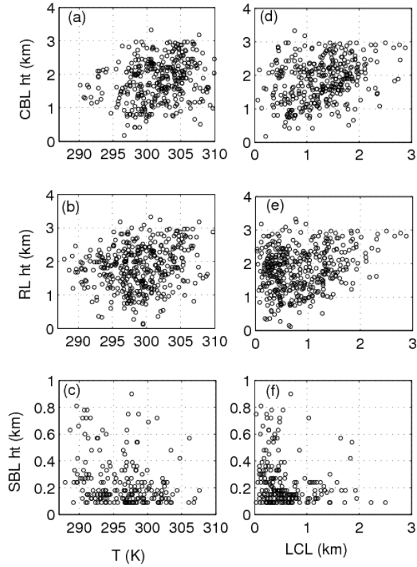
875 Figure 11: Scatter plot between the surface temperature and (a) CBL, (b) RL, and (c) SBL. (d)-(f) are same as (a)-(c) but for the LCL.
