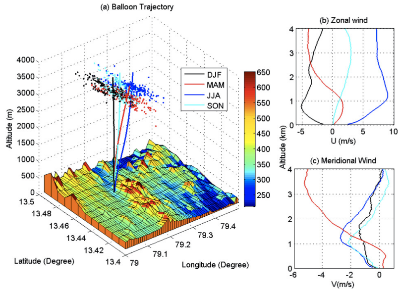
Figure 1: (a) Topographical features surrounding the location of radiosonde launch site, Gadanki ( 13.45^{\circ} N, 79.2^{\circ} E), a tropical station, India, along with profiles of seasonal mean trajectories (thick lines) from the surface to 4 km and the locations of the balloon reaching at altitude 4 km (dots) during different seasons. The mean (b) zonal wind and (c) meridional winds for different seasons observed during the period December 2010-March 2014. Global 30-arc-second gridded topography data is provided by the National Centers for Environmental Information, USA.
