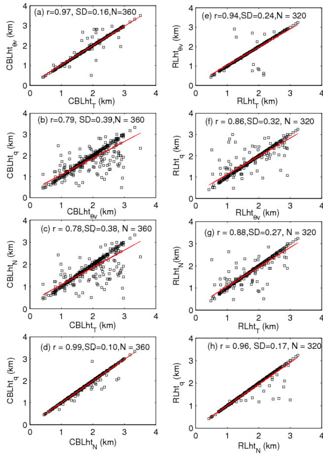
820 Figure 5: (Left panels) Scatter plot between the CBL heights obtained using (a) T and \theta_v , (b) \theta_v and q , (c) T and N , and (d) N and q , (Right Panels) (e)-(h) are same as (a)-(d) but the RL heights.
