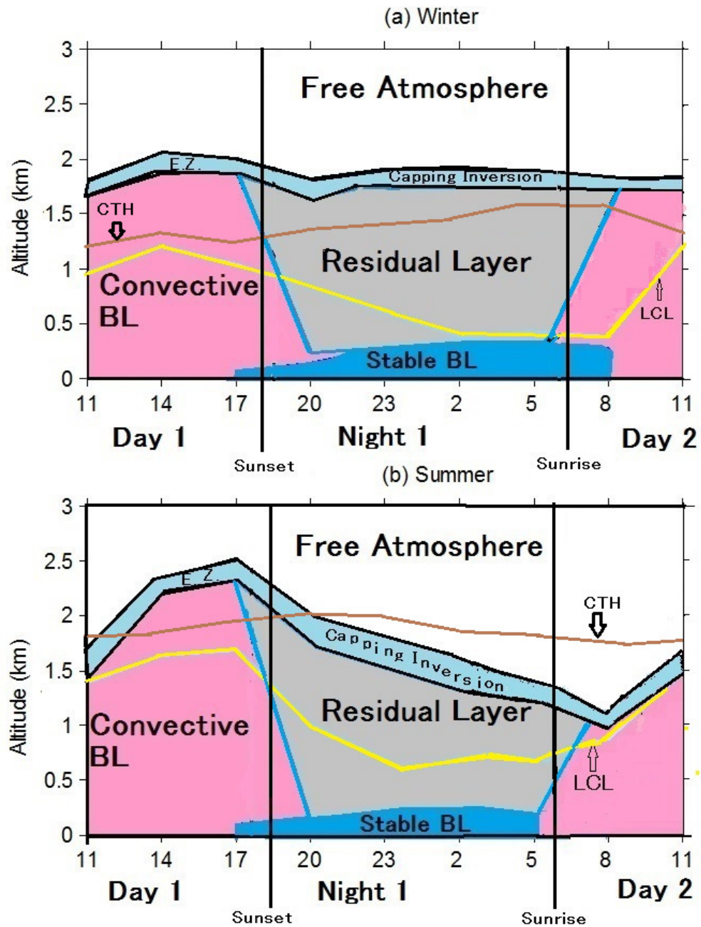
880 Figure 12: Schematic diagram of the vertical cross section of the mean ABL structure along with LCL and CTH during the (a) winter (DJF) and summer monsoon (JJA) seasons over Gadanki. E.Z. indicates entrainment zone.
