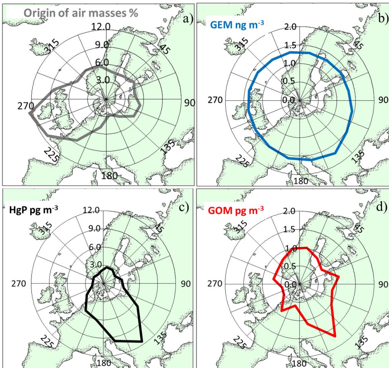
Figure 3. Results of the back trajectory analysis. a) origin of air masses reaching the Rão site presented as relative frequency (%) within each sector. b), c) and d) shows GEM, PBM and GOM concentrations, respectively as function of origin of air masses entering the measurement site.
