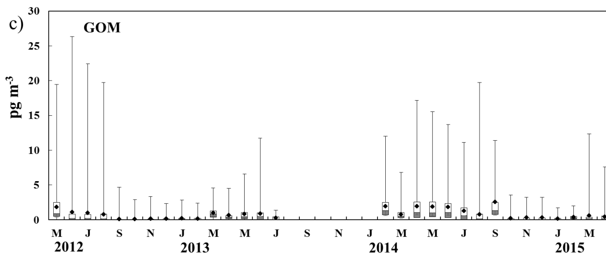
Figure 2. Boxplots of measured a) GEM, b) PBM and c) GOM at Råö/Rörvik from May 2012 to July 2013 and from 5 February 2014 to April 2015. Diamonds show average values. Upper and lower boxes show 75 % and 25 % percentiles, respectively with median values in between. Upper and lower whisker bars shows maximum and minimum values, respectively.
