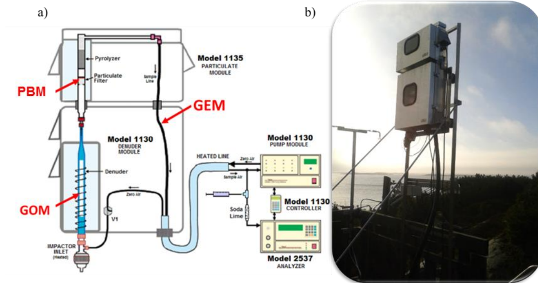
Figure 1. a) a schematic overview of the Tekran mercury speciation system 1130/35 and the 2537 mercury analyser, b) picture of the instrument operating at the Råö station.
