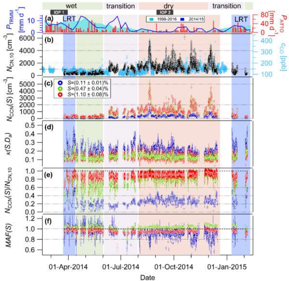
Figure 1. Seasonal trends in time series of precipitation rate P , total aerosol concentration N_{CN,10} , carbon monoxide mole fraction ( c_{CO} ), and CCN key parameters for three selected supersaturations S for entire measurement period (shown in original time resolution). (a) Precipitation rates from tropical rainfall measuring mission (TRMM) P_{TRMM} and in situ measurements at the ATTO site P_{ATTO} . The P_{TRMM} seasonal cycles are derived from an area upwind of the ATTO site (W 59.5°, N 2.4°, W 54.0°, S 3.5°), covering a long-term period from 1 Jan 1998 until 30 June 2016 (aqua shading), and the period of the CCN measurements from 1 Mar 2014 until 28 Feb 2015 (blue line). (b) Time series of pollution tracers N_{CN,10} and c_{CO} . (c) CCN concentrations N_{CCN}(S) , (d) hygroscopicity parameter \kappa(S, D_a) , (e) CCN efficiencies N_{CCN}(S)/N_{CN,10} , and (f) maximum activated fraction MAF(S) . Three different types of shading represent: (i) the seasonality in the Amazon atmosphere according to Andreae et al. (2015) (wet versus dry seasons with transition periods, illustrated in top of graph), (ii) periods of IOP1 and IOP2 during GoAmazon2014/5, (iii) seasonal periods of interest in context of the present study as defined in Sect. 3.3 (shading in background of time series).
