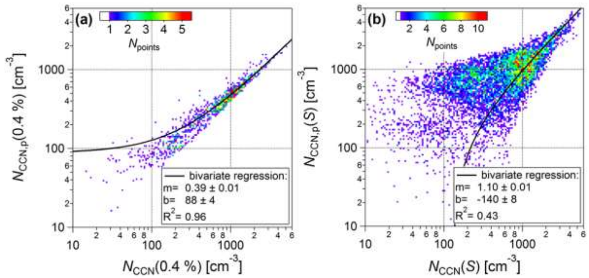
Figure 9. Predicted versus measured CCN number concentrations calculated from (a) observed ratio N_{\text{CCN}(0.4\%)} / N_{\text{CN}} = 0.36 in Andreae et al. (2009) and (b) observed (biomass burning-related) excess CCN to excess CO ratios in M. L. Pöhlker et al. (2016b). The color code shows the number of data points falling into the pixel area, following Jurányi et al. (2011). The black line represents a bivariate regression fit of the data.
