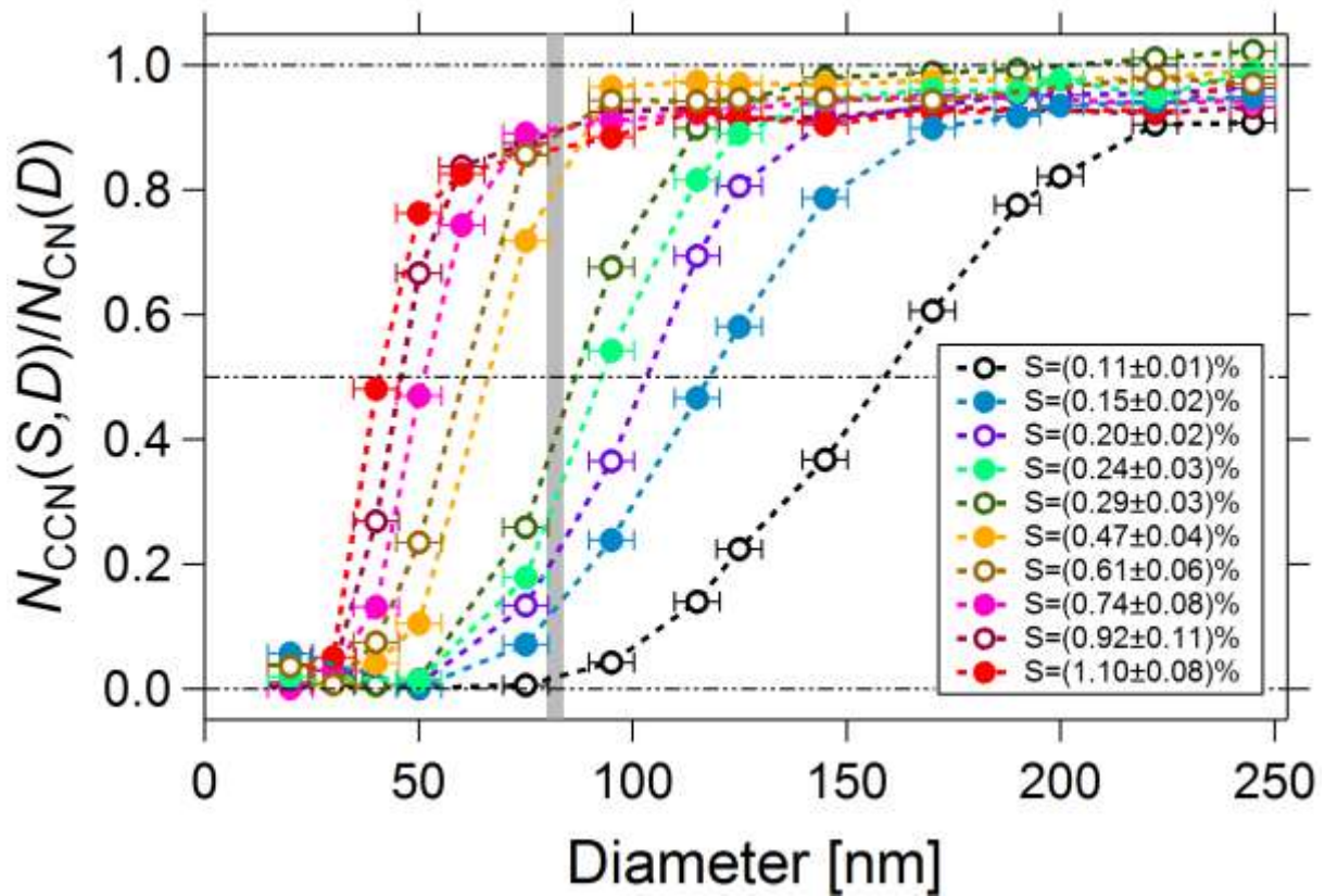
Figure 2. CCN activation curves for all measured S levels ( S = 0.11 - 1.10 %), averaged over the entire measurement period. Data points represent arithmetic mean values. For N_{CCN}(S,D)/N_{CCN}(D) the standard error is plotted, which is very small (due to the large number of scans with comparatively small variability) and, therefore, not perceptible in this representation. For the diameter, D , the error bars represent the experimental error as specified in Sect. 2.3. The grey vertical band represents the position of the Hoppel minimum (including error range) for the annual mean number size distribution (compare Fig. 3). Dashed lines provide visual orientation and indicate 0, 50, and 100 % activation. The value at 50 % activation is used for calculation of the hygroscopicity parameter \kappa(S,D_a) . The lines connecting the data points merely serve as visual orientation.
