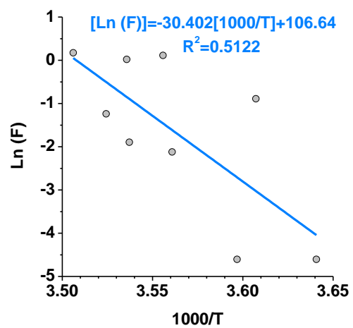
Figure S3. Arrhenius relationships between Hg(0) flux and soil temperature during May–June 2015 campaign.
