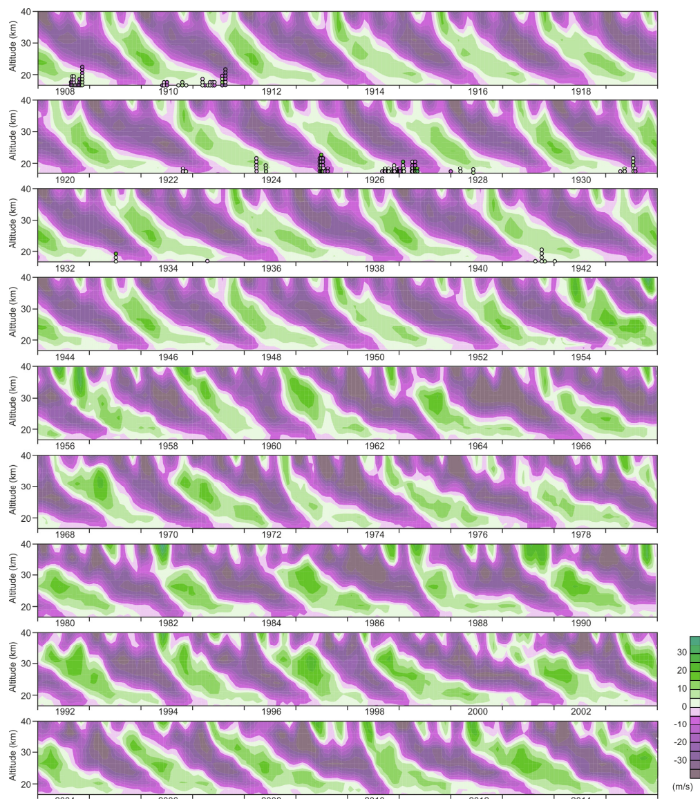
Figure 1: Hovmöller diagram (time–height cross section) of zonal-mean zonal wind at the equator from 1908 to 2015 (from Brönnimann et al., 2007). The dots indicate the additional wind data rescued within the ERA-CLIM project.
