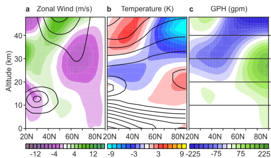
Figure 2: Composite fields (shading) and climatologies (contours) of ERA-Interim for boreal winter for easterly minus westerly QBO phases for zonal averages of (a) zonal wind (contours: 20 to 60 m/s in steps of 10 m/s), (b) temperature 5 (contours: 200 to 300 K in steps of 10 K) and (c) GPH in Jan.-Mar. using the 50 hPa QBO early winter.
