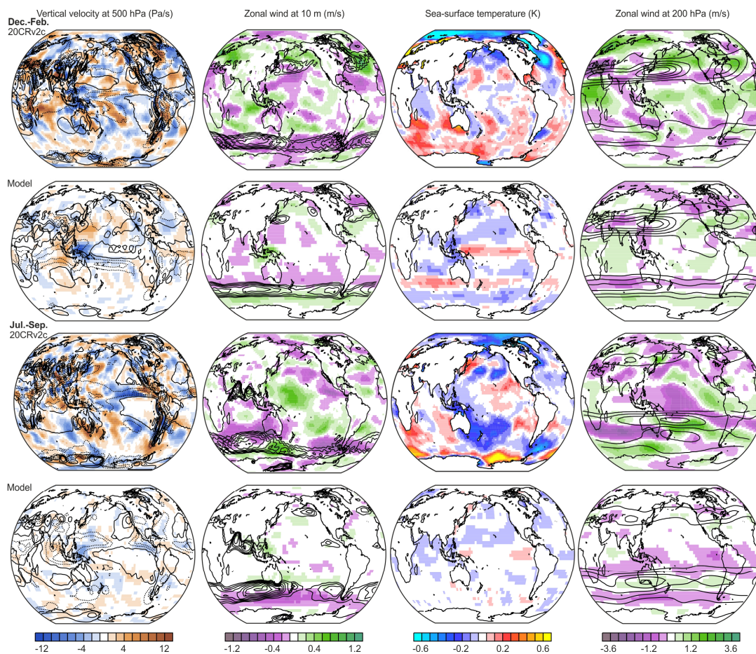
Figure 6: Composite fields for easterly minus westerly QBO phases for (left) 500 hPa vertical velocity (shading, contours indicate climatology, spacing is 40 Pa/s symmetric around zero, dashed are negative), 10 m zonal wind (shading, contours indicate climatology from 4 m/s in steps of 1 m/s), SST, and 200 hPa zonal wind (shading, contours indicate climatology from 20 m/s in steps of 10 m/s) for boreal summer and winter in 20CRv2c and in the model simulations. See Fig. S10 for significance.
