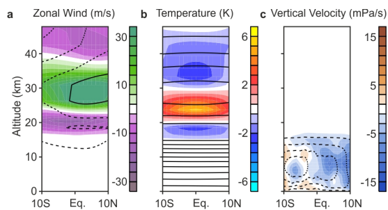
Figure 5: Composite fields (shading) and climatologies (contours) of ERA-Interim for boreal winter for easterly minus 5 westerly QBO phases for zonal averages within 120–160° E for (a) zonal wind contours: (-50 to 50 m/s in steps of 20 m/s), (b) temperature (contours: 200 to 300 K in steps of 10 K) and (c) omega (-70 to 70 Pa/s in steps of 20 Pa/s) in Dec.-Feb. using the 70 hPa QBO definition.
