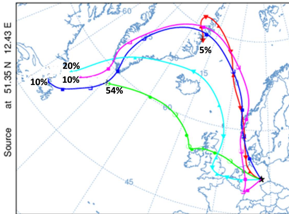
5 Figure 8. Cluster analysis of the HYSPLIT back trajectories that arrive every hour (from 23 September 12:00 UTC up to 24 September 18:00 UTC) at 2.5-3.5 km height over Leipzig. A 54% cluster percentage means that there is 54% chance that the SO 2 arriving anywhere between 2.5-3.5 km over Leipzig originates from the specific direction.
