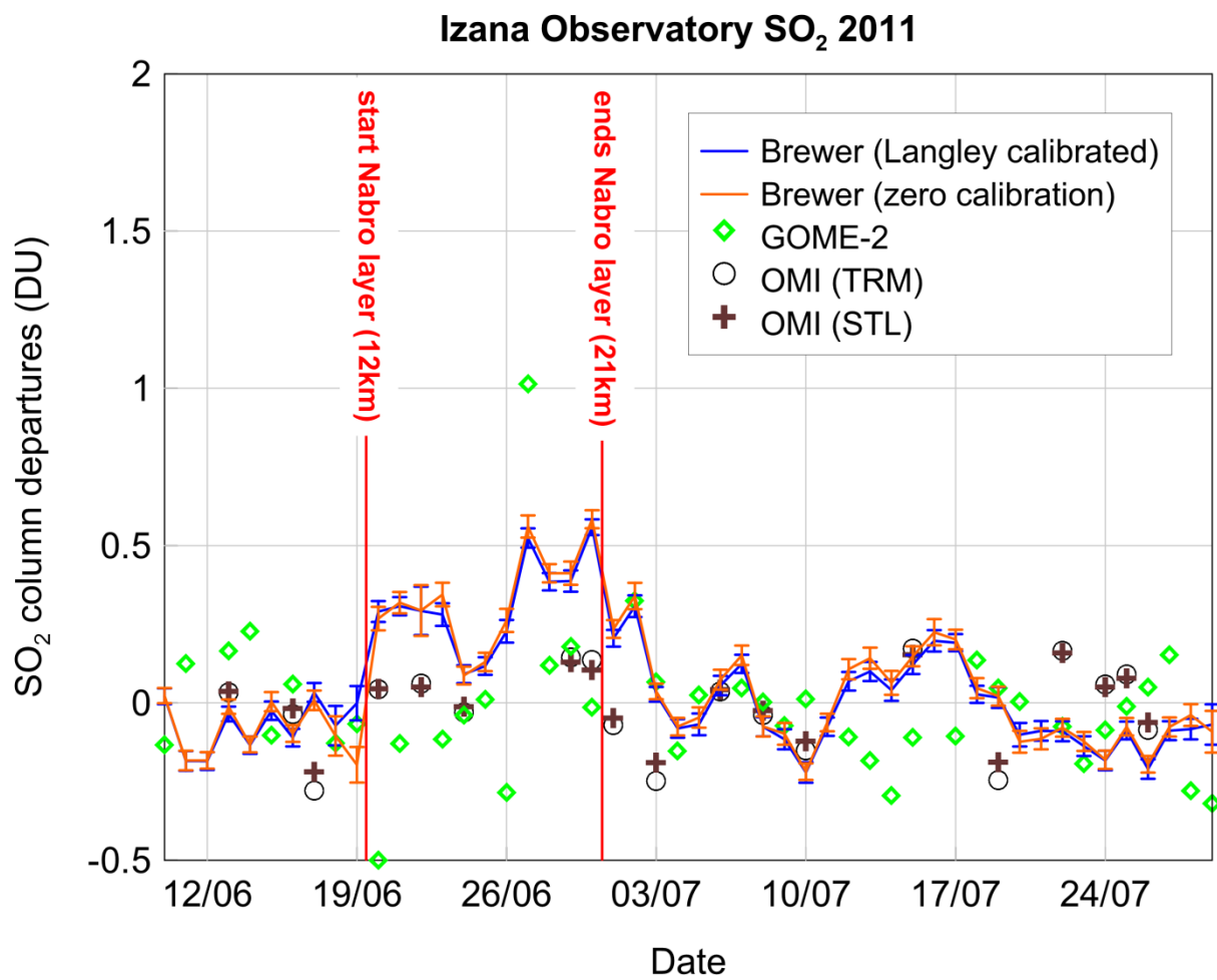
5 Figure 11. SO 2 column departures from the unperturbed 10 day pre-volcanic baseline measured by the Brewer, OMI (TRM, STL) and GOME-2 over Izaña, Tenerife, during June-July 2011 following the 2011 Nabro volcanic eruption. SO 2 calculations by the Brewer were performed using the Langley calibration and the zero calibration at Izaña (assuming SO 2 =0 during the days 06 and 07 of June 2011).
