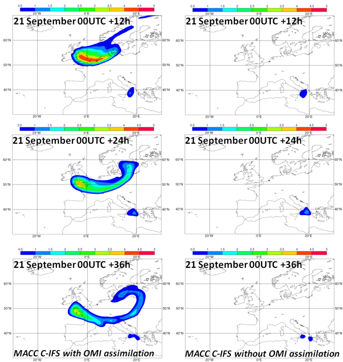
5 Figure 6. Charts of forecasted total column SO 2 produced within the MACC system for 21 September 2014 with OMI data assimilation (left) and without OMI data assimilation (right).
