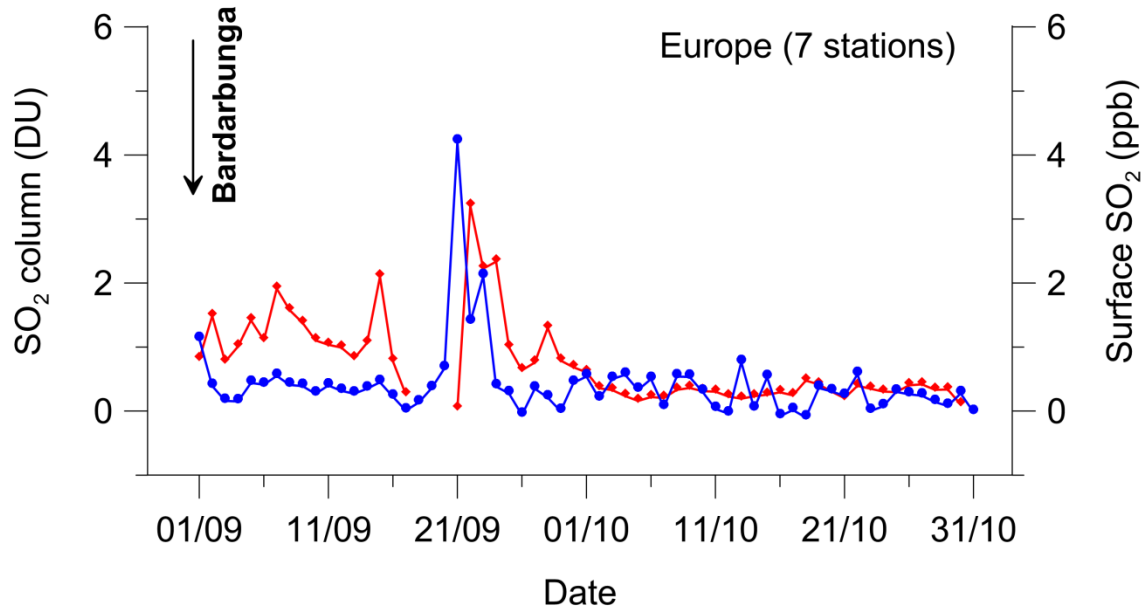
Figure 5. Mean surface SO 2 measured by Airbase class 1-2 stations located within 150 km from 7 nearest Brewer stations in Europe as listed in Table 3. The arrow marks the starting date of the eruption (beginning on 31 August 2014 which continued to be active throughout the whole bimonthly period and beyond).
