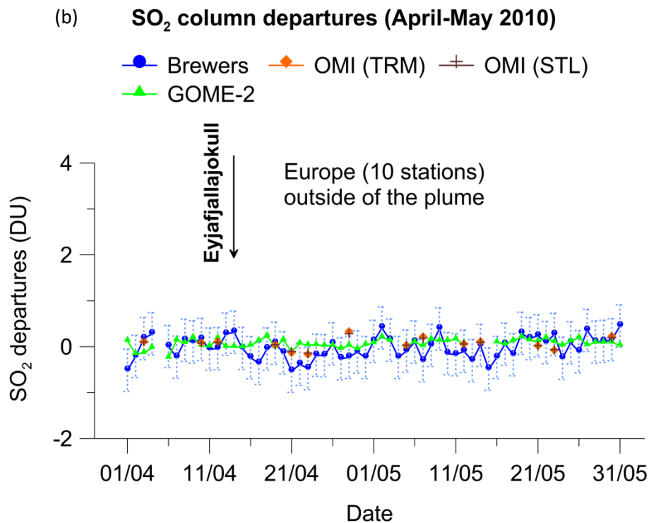
Figure 12. Mean SO 2 column departures from the unperturbed 10 day pre-volcanic baseline measured by Brewers, OMI (TRM, STL) and GOME-2 during April-May 2010 over Europe following the 2010 Eyjafjallajökull volcanic eruption for: (a) stations under the volcanic SO 2 plume, and (b) stations outside of the plume. The error bars for the Brewer observations show the standard deviation of all daily values during the unperturbed 10 day period prior to the volcanic eruption. Brewer stations under the plume are: Sodankylä, Obninsk, Manchester, De Bilt, Uccle, Belsk, Reading, Hohenpeissenberg, Davos and Arosa. Stations outside of the plume are: Vindeln, Oslo, Norrkoeping, Copenhagen, Hradec Kralove, Aosta, Kislovodsk, Rome, Thessaloniki and Athens. Each daily average from either OMI or GOME-2 was calculated if and only if more than half of the individual overpasses had data at a given day. The arrow marks the starting date of the eruption (beginning on 14 April until 24 May 2010).
