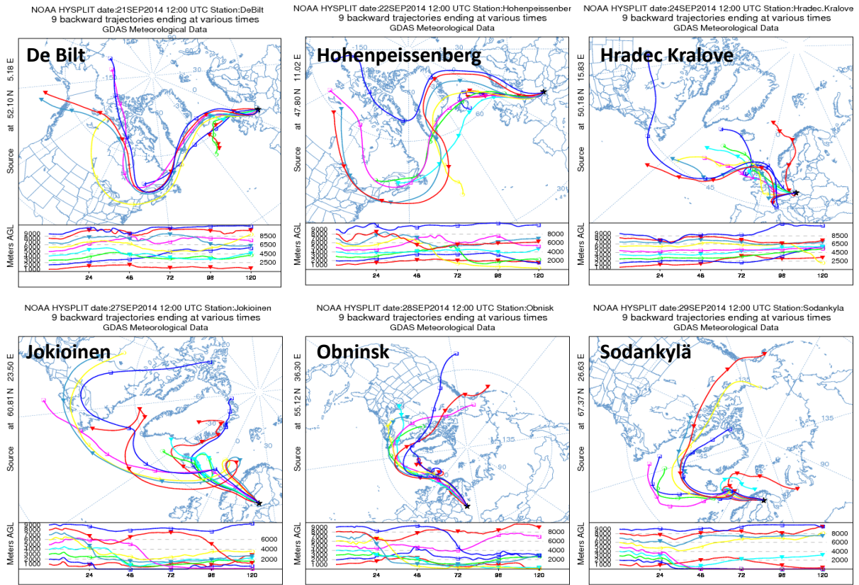
5 Figure 3. HYSPLIT 120 hours back trajectories of air masses arriving on the day of maximum SO 2 records for each one of the Brewer stations at De Bilt, Hohenpeissenberg, Hradec Kralove, Jokioinen, Obninsk and Sodankylä.
