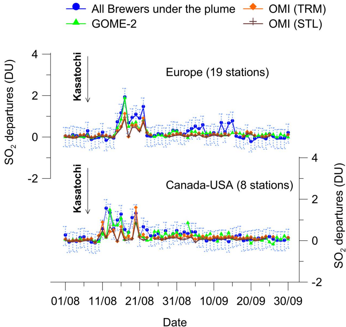
5 Figure 14. Mean SO 2 column departures from the unperturbed 10 day pre-volcanic baseline measured by Brewers, OMI (TRM, STL) and GOME-2 during August-September 2008 over Europe and Canada/USA following the 2008 Kasatochi volcanic eruption. The error bars for the Brewer observations show the standard deviation of all daily values during the unperturbed 10 day period prior to the volcanic eruption. Stations in Europe include: Sodankylä, Vindeln, Jokioinen, Norrkoeeping, Copenhagen, Manchester, De Bilt, Belsk, Reading, Uccle, Hradec Kralove, Hohenpeissenberg, Davos, Arosa, Aosta, Kislovodsk, Rome, Thessaloniki and Athens. Stations in Canada/USA 10 include: Churchill, Edmonton, Goose Bay, Regina, Saturna Island, Toronto, Boulder and Mauna Loa. Each daily average from either OMI or GOME-2 was calculated if and only if more than half of the individual overpasses had data at a given day. The arrow marks the date of the eruption (7 August 2008).
