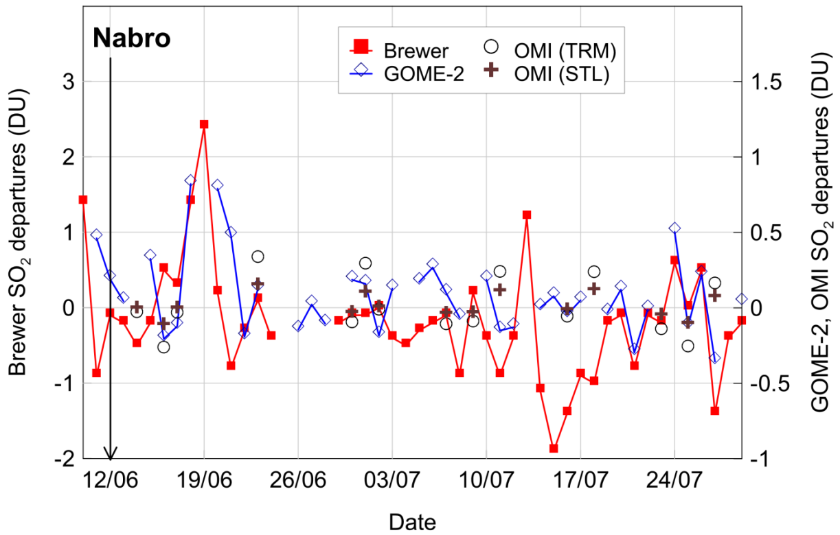
Figure 9. SO 2 column departures from the unperturbed 10 day pre-volcanic baseline measured by Brewer, OMI (TRM, STL) and GOME-2 over Taipei, Taiwan, during June-July 2011 following the 2011 Nabro volcanic eruption (on 12 June 2011).
