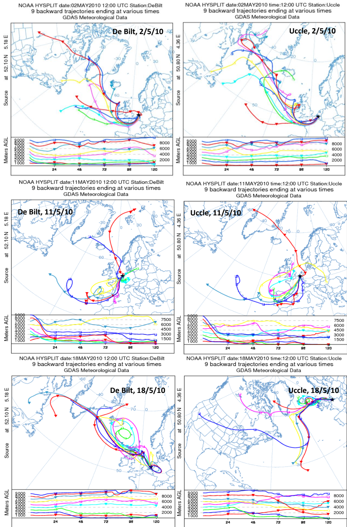
5 Figure 13. HYSPLIT 120 hours back trajectories of air masses arriving at De Bilt (left column) and Uccle (right column) on 2 May 2010 (1 st row), 11 May 2010 (2 nd row), 18 May 2010 (3 rd row).
