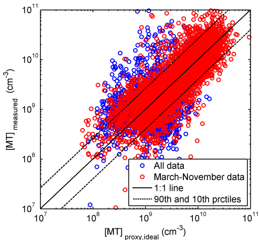
5 Figure 2. A correlation between the measured monoterpane concentration and concentration predicted by MT_{\text{proxy,ideal}} , which is calculated by using the measured monoterpane concentration for determining the concentration of \text{NO}_3 . The blue circles show all data and the red circles show data for March–November. The solid black line shows 1:1 line and the dotted black lines show 90th and 10th percentiles of the ratio between the measurements and proxy. The variability V_{90/10} is calculated as the ratio of the 90th and 10th percentiles.
