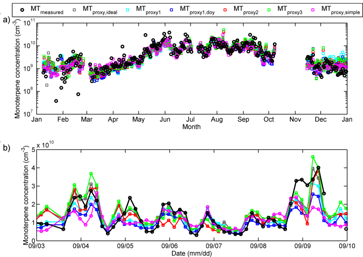
5 Figure 4. Time series of the measured monoterpene concentration and the concentrations predicted by different proxies (a) for the whole year 2013, (b) for one week in September. The black circles show the measured concentration, the grey squares show \text{MT}_{\text{proxy,ideal}} , the light blue squares \text{MT}_{\text{proxy1}} , the dark blue squares \text{MT}_{\text{proxy1,doy}} , the red squares \text{MT}_{\text{proxy2}} , the green squares \text{MT}_{\text{proxy3}} , and the magenta squares \text{MT}_{\text{proxy,simple}} .
