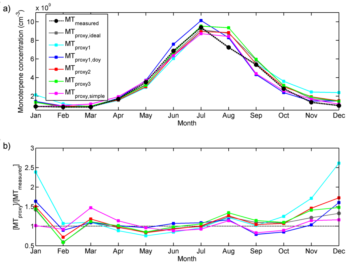
Figure 6. Monthly medians of (a) the concentrations of the measured monoterpenes and different proxies and (b) the ratios of different proxies to measured monoterpene concentration. The black circles show the measured concentration, the grey squares show \text{MT}_{\text{proxy,ideal}} , the light blue squares \text{MT}_{\text{proxy1}} , the dark blue squares \text{MT}_{\text{proxy1,doy}} , the red squares \text{MT}_{\text{proxy2}} , the green squares \text{MT}_{\text{proxy3}} , and the magenta squares \text{MT}_{\text{proxy,simple}} .
