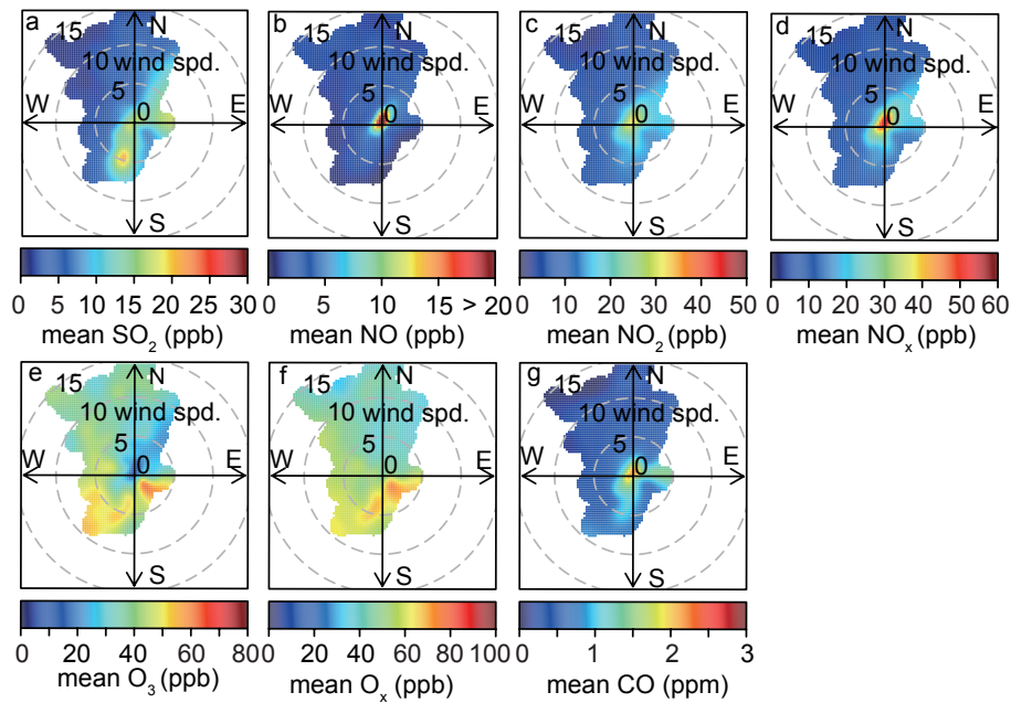
871 Figure 5. Bivariate polar plots for SO 2 (a), NO (b), NO 2 (c), NO x (d), O 3 (e), O x (f) and CO 872 (g) concentrations based on hourly average data at the Yufa site from 1 September 873 2006 to 31 August 2008. The colour scale shows the concentrations of pollutants in 874 ppb (or ppm specially for CO) and the radial scale shows the wind speed ( \text{m s}^{-1} ), 875 which increases from the centre of the plot radially outwards.
