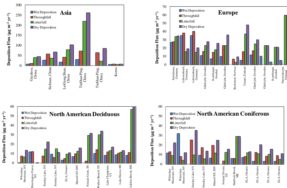
Figure 1: Contributions to the mercury deposition flux ( \mu\text{g m}^{-2} \text{yr}^{-1} ) from wet deposition, throughfall Hg, litterfall Hg, and dry deposition in: (a.) Asia, (b.) Europe, (c.) North American deciduous forests, and (d.) North American coniferous forests. (References in order of appearance: Fu et al., 2010a, b; Wang et al., 2009; Luo et al., 2015; Schwesig and Matzner, 2000, 2001; Hultberg et al., 1995; Lee et al., 2000; Larssen et al., 2008; orvari and Verta, 2003; Iverfeldt, 1991; Lee et al., 1998; Blackwell and Driscoll, 2015b; Choi et al., 2008; Demers et al., 2007; Kalicin et al., 2007; Graydon et al., 2008; Grigal et al., 2000; Fisher and Wolde, 2012; Lindberg et al., 1996; Rea et al., 1996, 2001; Johnson et al., 2007; St. Louis et al., 2001))
