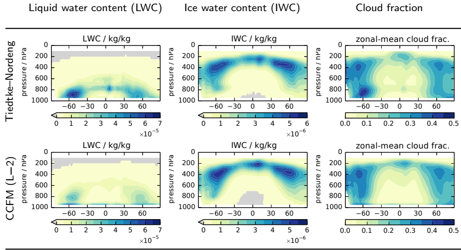
Figure 3. Annual and zonal mean (from left to right) liquid water content (LWC), ice water content (IWC) and cloud fraction from 30-year AMIP-type simulations using ECHAM(-HAM) ECHAM–HAM with Tiedtke–Nordeng and CCFM (L–2) convection. Note that the LWC and IWC scales are different for ECHAM and ECHAM–HAM due to their quite different magnitudes.
