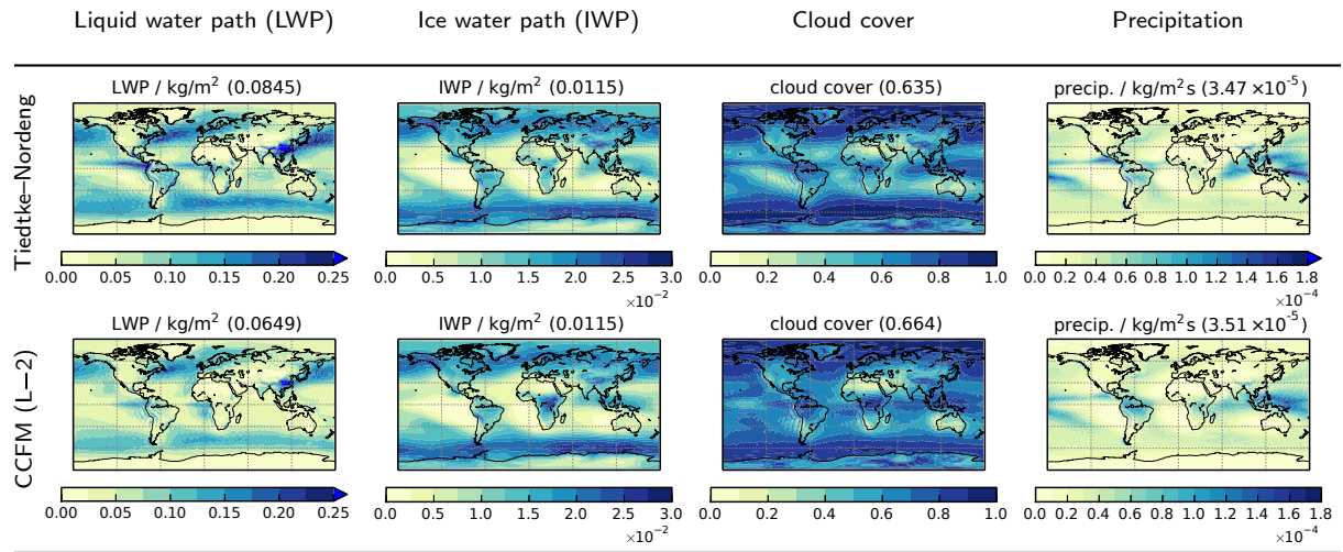
Figure 2. Annual mean (from left to right) liquid water path (LWP), ice water path (IWP), cloud cover and surface precipitation from 30-year AMIP-type simulations using ECHAM(–HAM) ECHAM–HAM with Tiedtke–Nordeng and CCFM (L–2) convection. Note that the LWP and IWP scales are different for ECHAM and ECHAM–HAM due to their quite different magnitudes. (The numbers in parentheses show the annual global mean of each quantity.)
