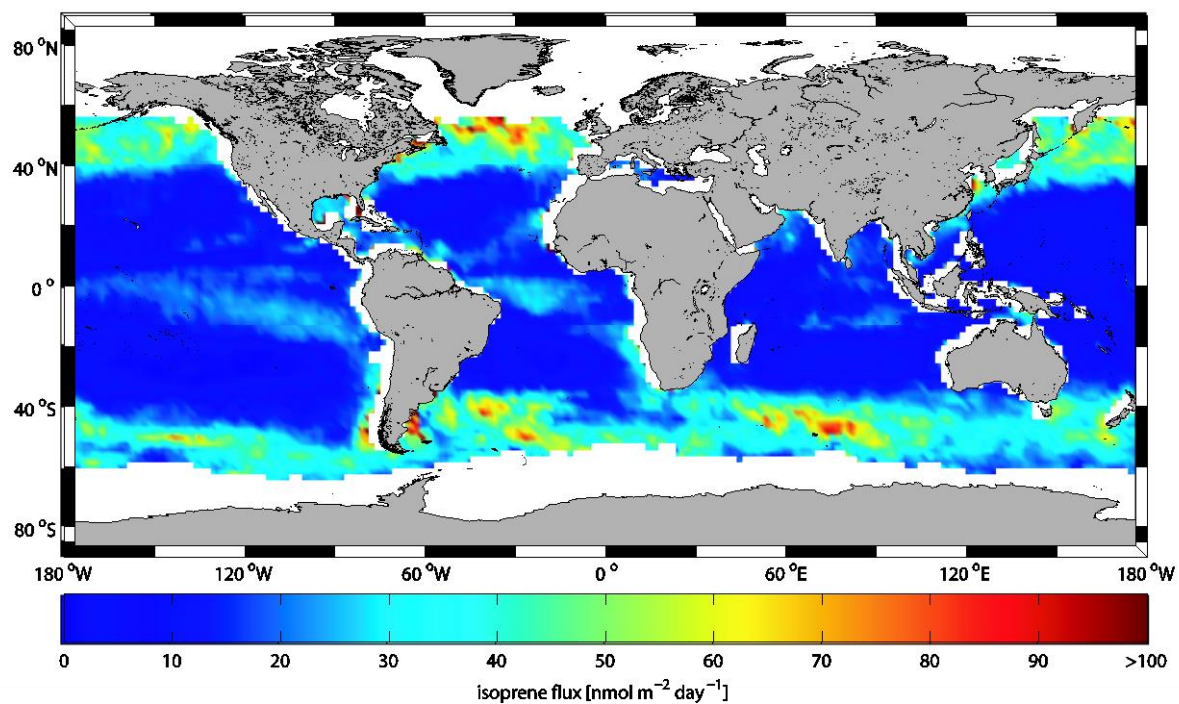
Figure S11: Global monthly mean marine isoprene fluxes in nmol m -2 day -1 for November 2014.
