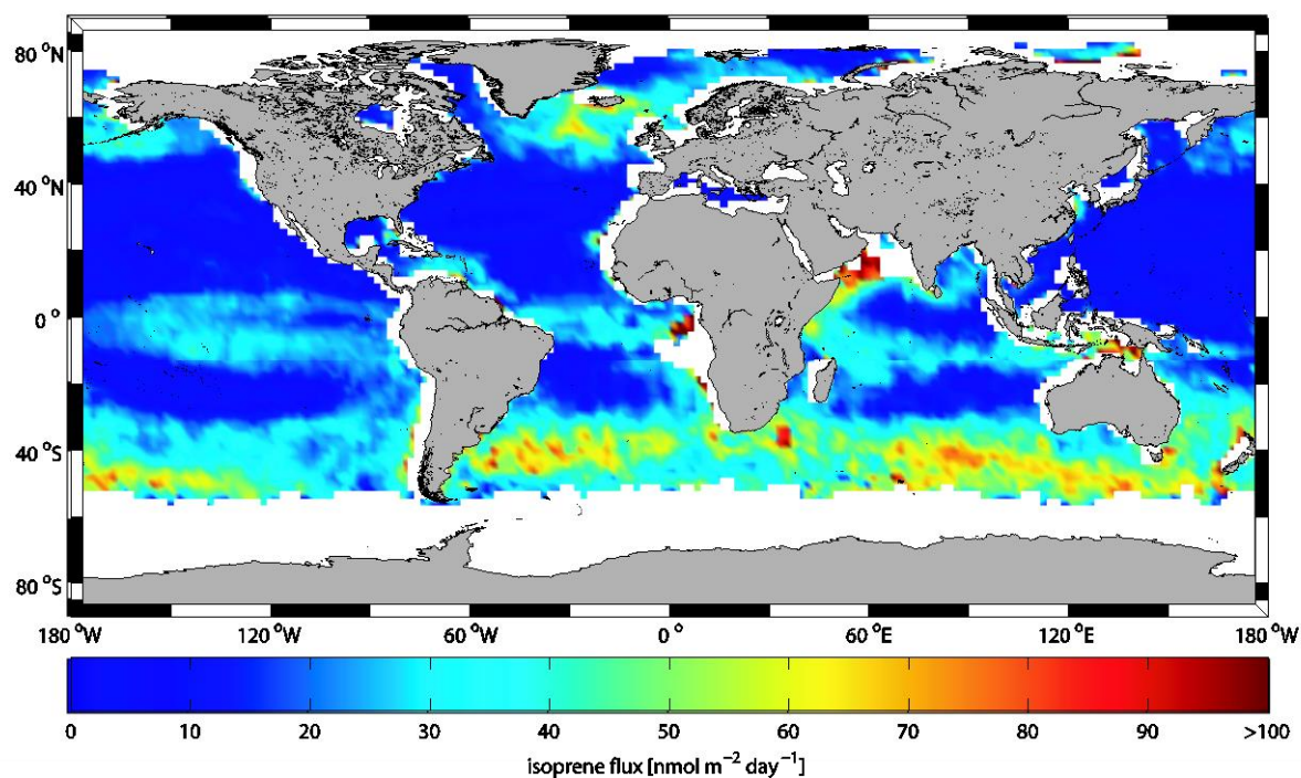
Figure S8: Global monthly mean marine isoprene fluxes in nmol m -2 day -1 for August 2014.
