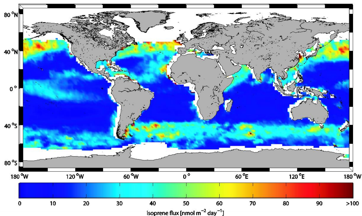
Figure S1: Global monthly mean marine isoprene fluxes in nmol m -2 day -1 for January 2014.
