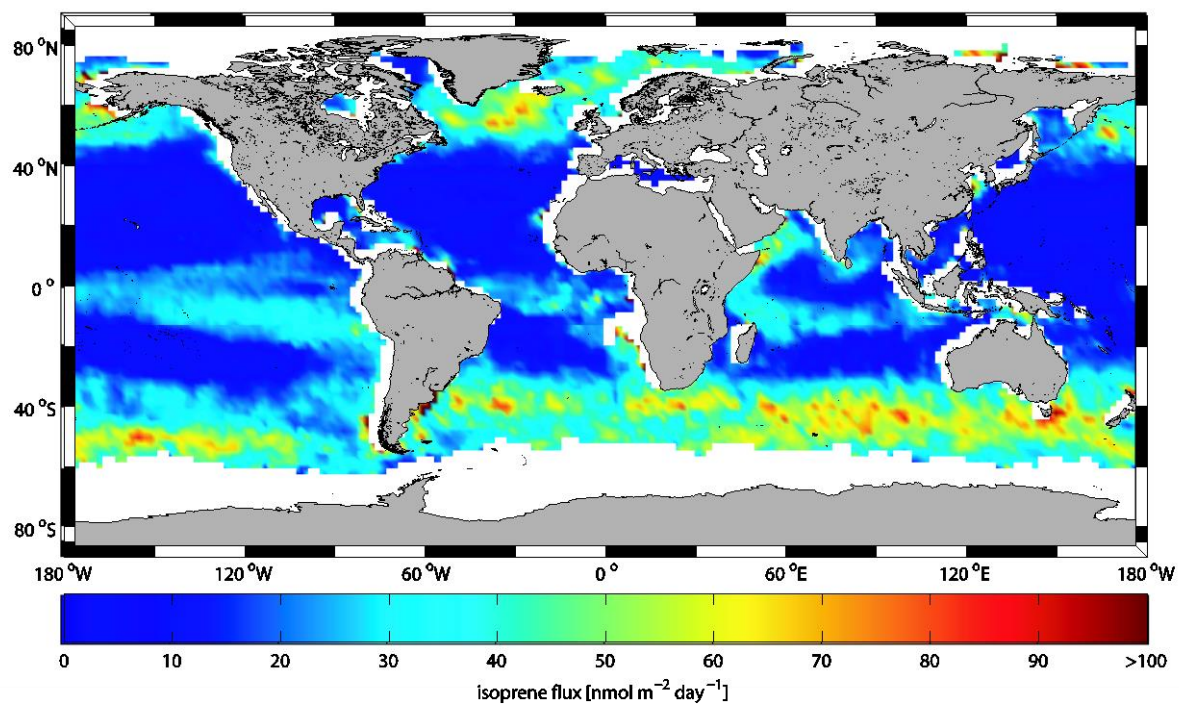
Figure S9: Global monthly mean marine isoprene fluxes in nmol m -2 day -1 for September 2014.
