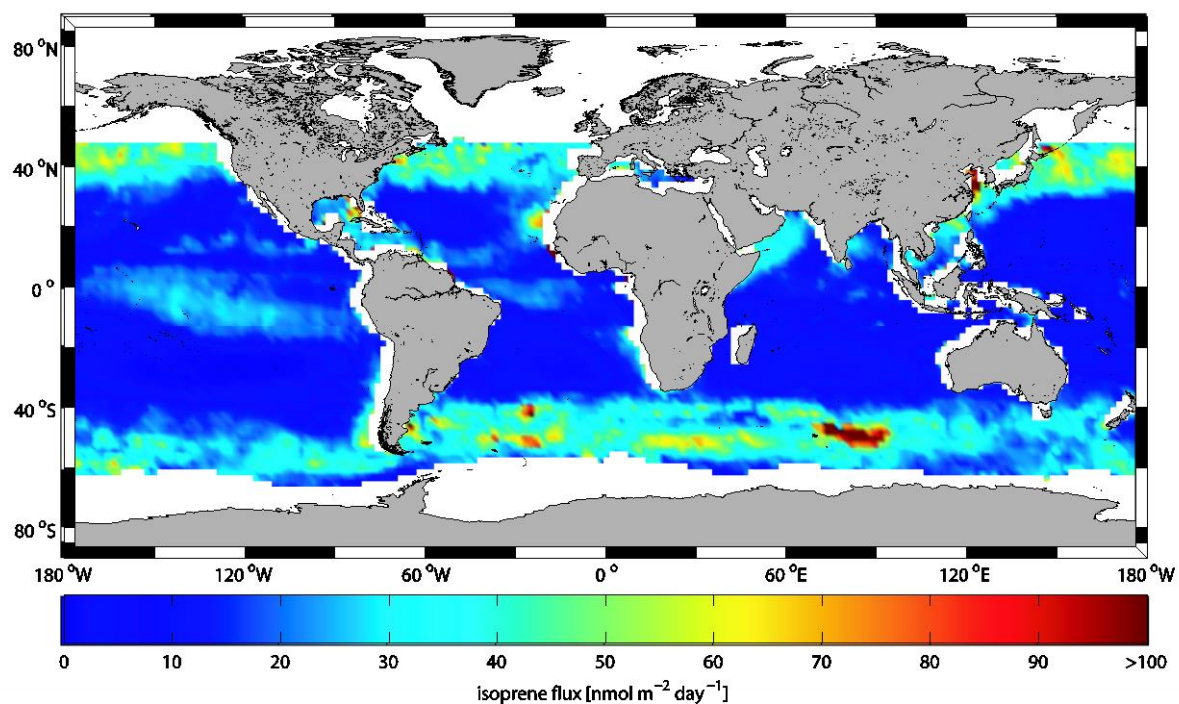
Figure S12: Global monthly mean marine isoprene fluxes in nmol m -2 day -1 for December 2014.
