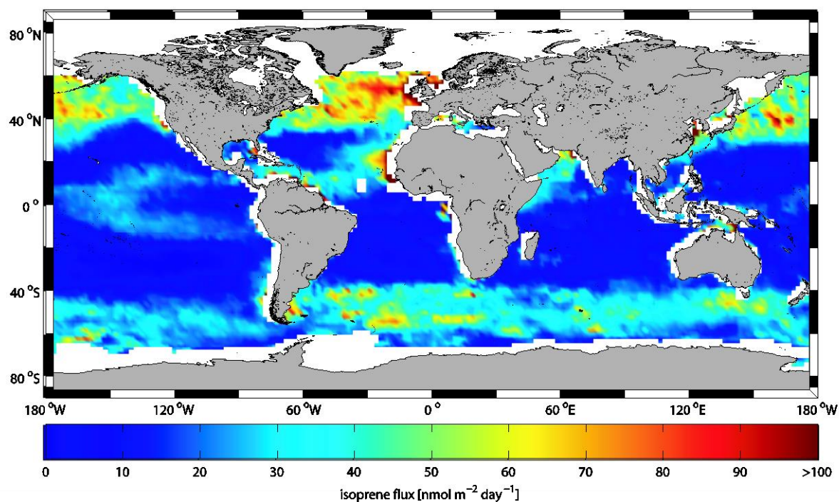
Figure S2: Global monthly mean marine isoprene fluxes in nmol m -2 day -1 for February 2014.
