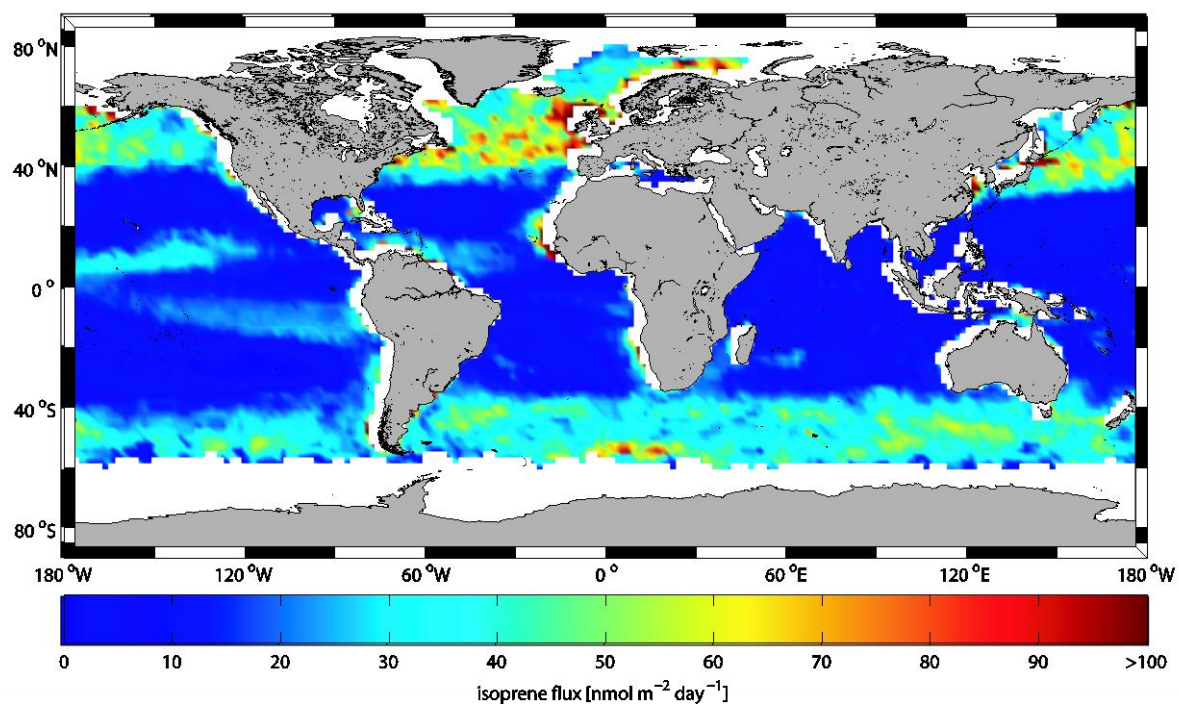
Figure S4: Global monthly mean marine isoprene fluxes in nmol m -2 day -1 for April 2014.
