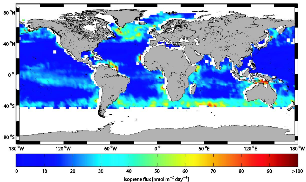
Figure S6: Global monthly mean marine isoprene fluxes in nmol m -2 day -1 for June 2014.
