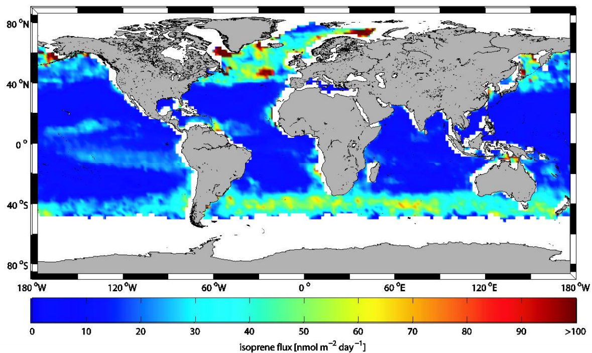
Figure S5: Global monthly mean marine isoprene fluxes in nmol m -2 day -1 for May 2014.
