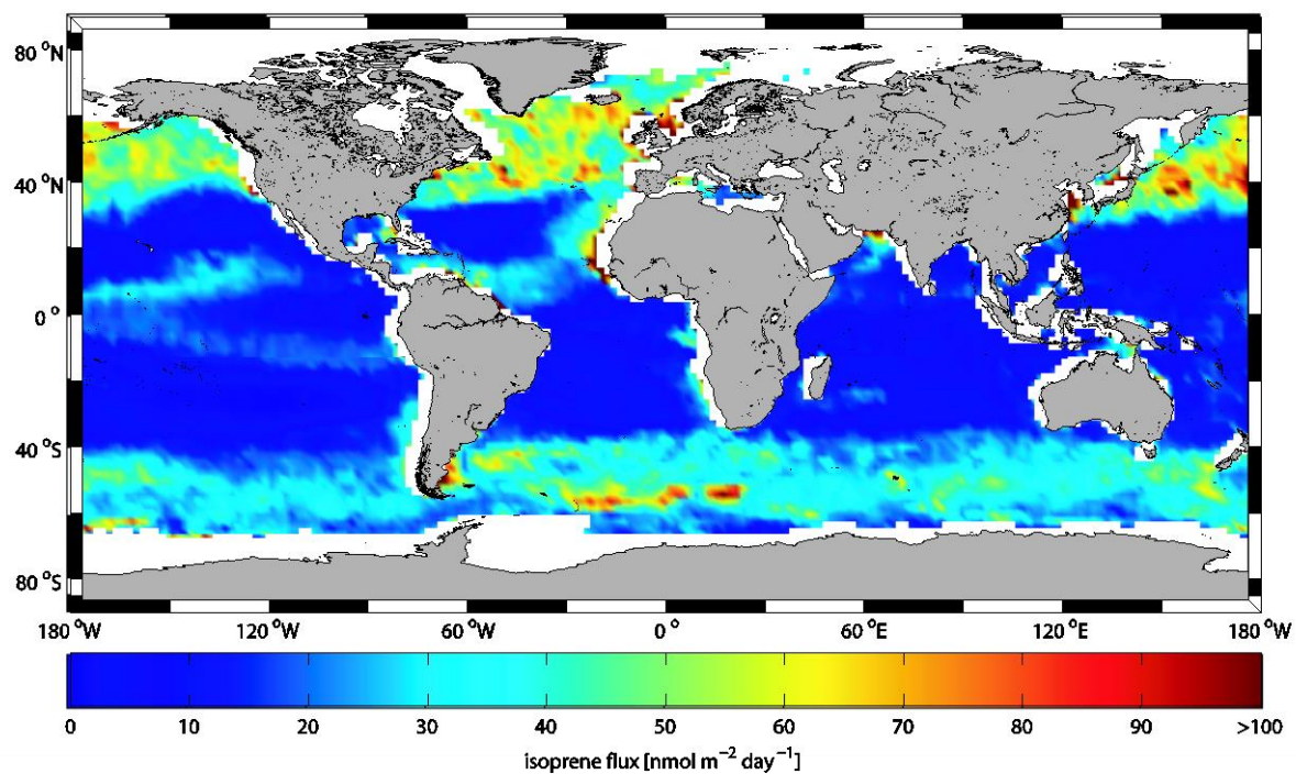
Figure S3: Global monthly mean marine isoprene fluxes in nmol m -2 day -1 for March 2014.
