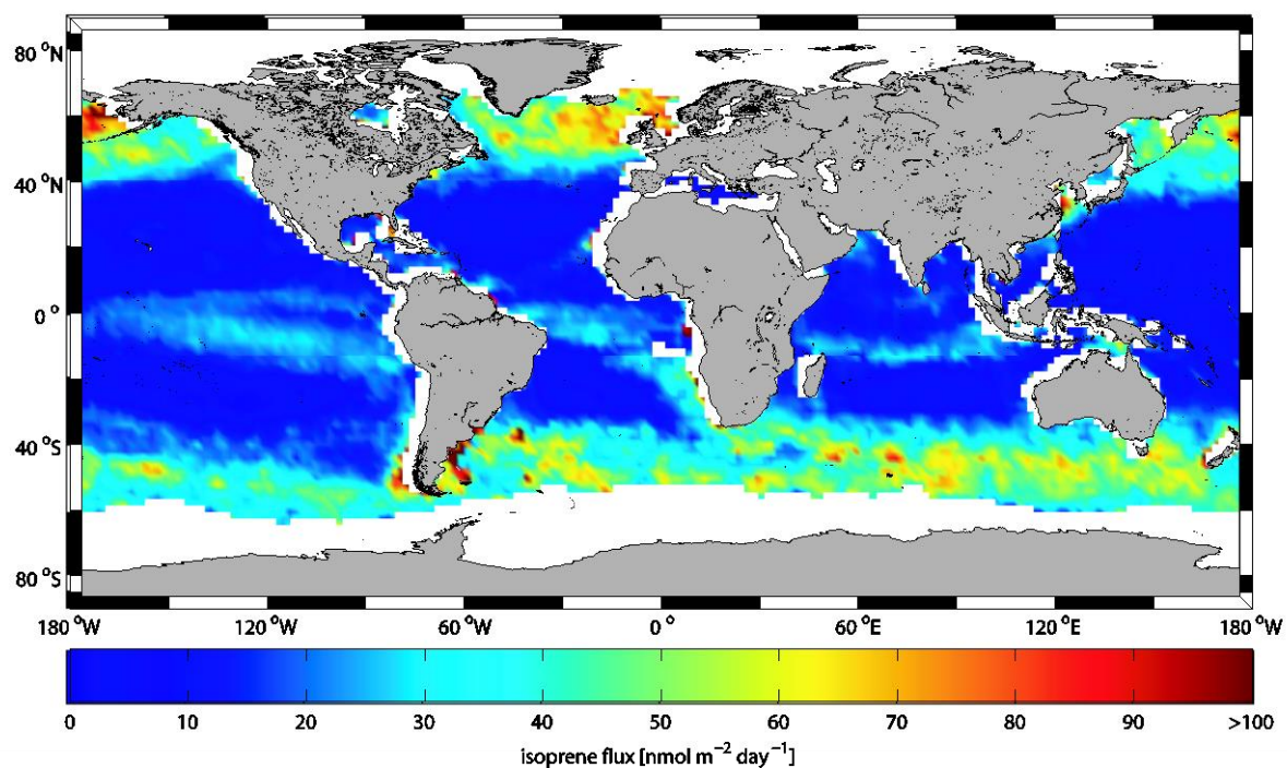
Figure S10: Global monthly mean marine isoprene fluxes in nmol m -2 day -1 for October 2014.
