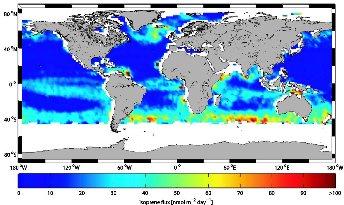
Figure S7: Global monthly mean marine isoprene fluxes in nmol m -2 day -1 for July 2014.
