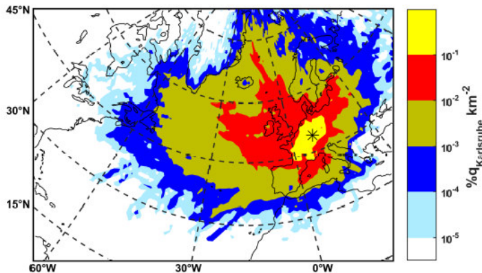
Figure 5. Source regions of moisture ( q ) 30m above ground level in Karlsruhe (black star) based on five-day back trajectories for the time period January 2012 to May 2013. The color code indicates the contribution of different source regions to q in Karlsruhe in % per \text{km}^2 . Integration over the whole map gives the total identified humidity of 47%.
