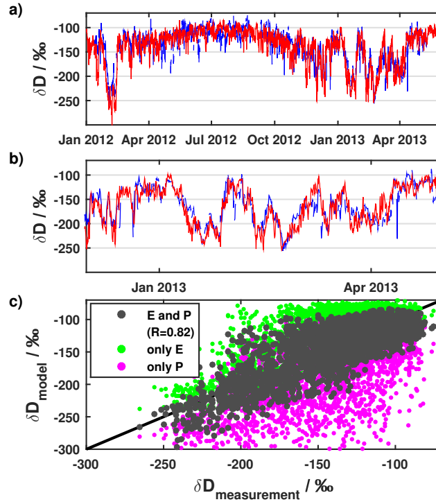
Figure 7. (a) Time series of measured (blue) and modeled (red) \delta D - \delta D of water vapor in Karlsruhe. (b) Enlarged section of (a), which demonstrates the capability of the model of capturing the high variability of \delta D - \delta D in winter. (c) Measured versus modeled \delta D - \delta D . The three-hourly available modeled \delta D - \delta D is compared to the temporally closest ten-minute average of the \delta D - \delta D observations. Gray: reference run, surface evaporation (E) and the formation of precipitation (P) are considered ( R=0.82 , \Delta\delta D \Delta\delta D = +1.0 - 4.1\% ); green: only E is considered, P is ignored ( R=0.81 , \Delta\delta D \Delta\delta D = +29.423.9\% ); magenta: only P is considered, E is ignored ( R=0.62 , \Delta\delta D \Delta\delta D = -35.634.8\% ); black: 1:1 line.
