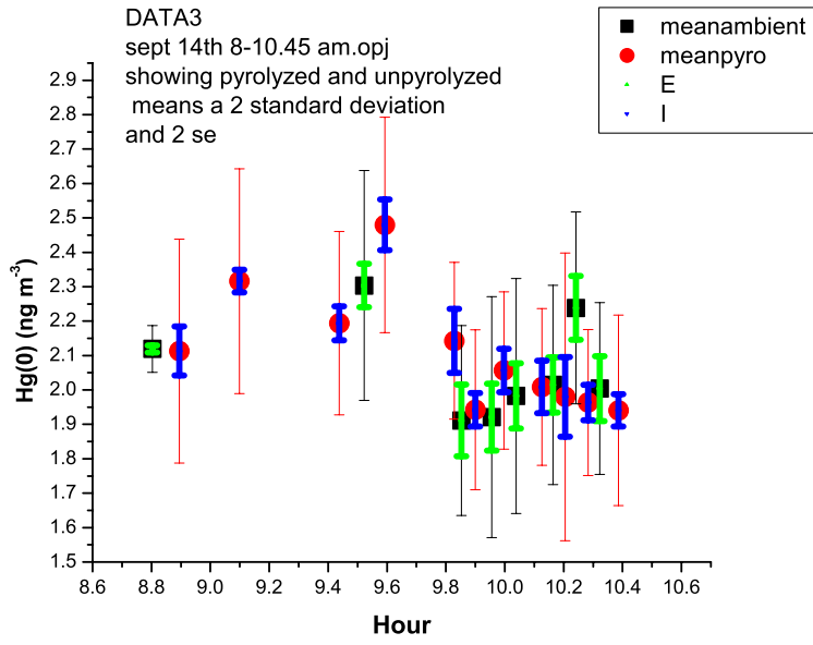
SI Figure 5: September 14 measurements 8-10.45 am. The means of the ambient channel (black) and pyrolyzed channel (red) are shown. The error bars show both 2 standard errors (thicker line) and 2 standard deviations.
