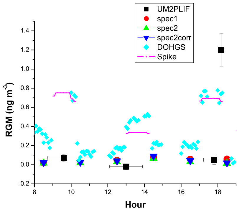
SI Figure 10: September 14 measurements: hour 8-19. The means of the 2P-LIF measurements are shown. The x-axis error bar shows the sample time. The y-error bar is 2SE of the mean. The measurements for the UNR speciation units spec 1 and spec 2 show the sum of gaseous and particle bound oxidized mercury. The values of Spec 2 using the correction suggested by Gustin et al. (2013) are also shown. The spike concentrations were reported by the UW manifold team. The DOHGS concentrations are 5 minute averages.
