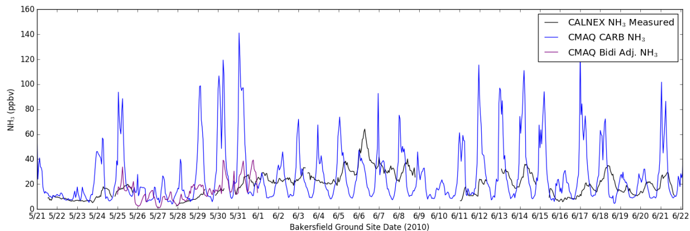
Figure S1. A time series plot of \text{NH}_3 from the Bakersfield ground site measurements (black), the CMAQ hourly output at that location (blue), the CMAQ case study run with the bi-directional ammonia scheme and adjusted emissions (purple).
