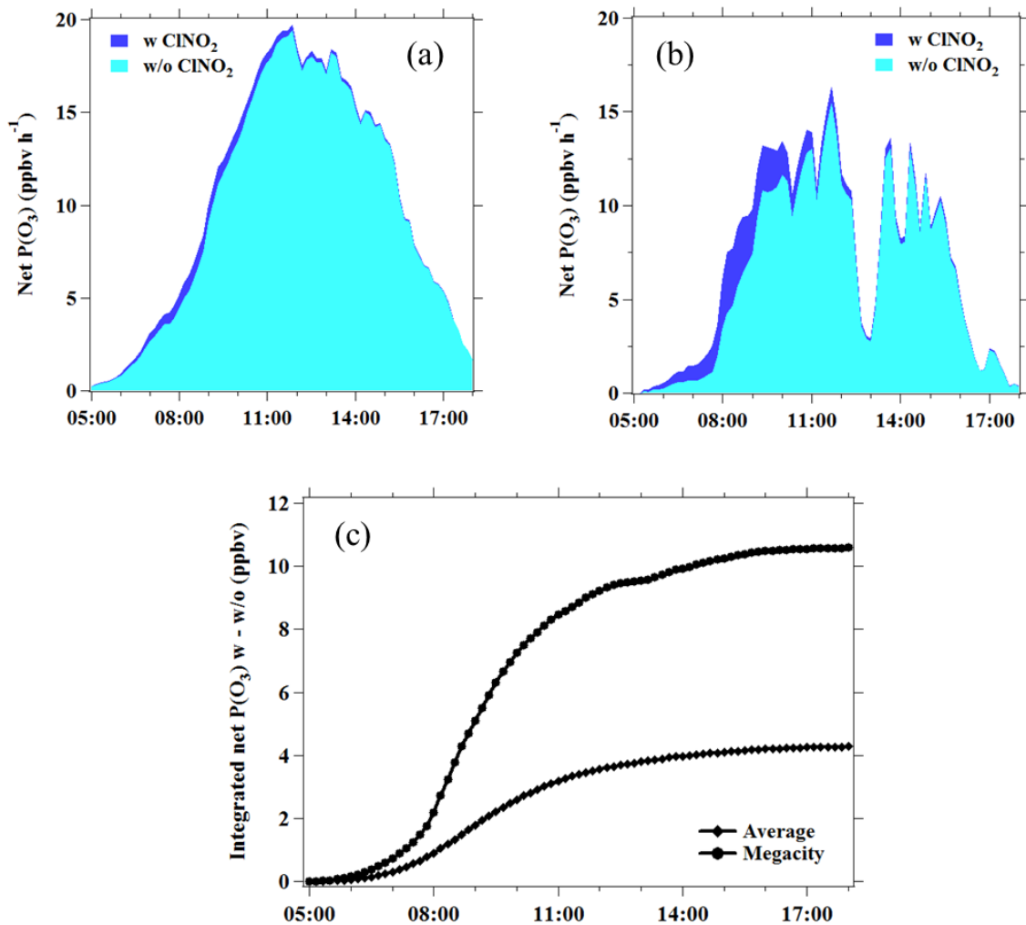
Figure 11. Net ozone production rates for a) average, b) the megacity case and c) the difference in integrated net ozone production rate between the simulation with and without the CINO 2 input.
