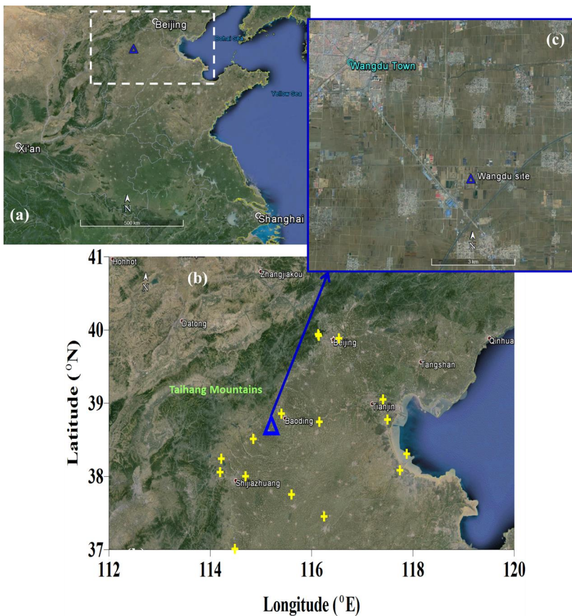
5 Figure 1. Google map showing a) the location of northern China (white dash-box) and Wangdu site (blue triangle), b) an expanded view of northern China plain with the topography, major cities and the locations of major coal-fired power plants (yellow cross) in the region, c) nearby environment of Wangdu site.
