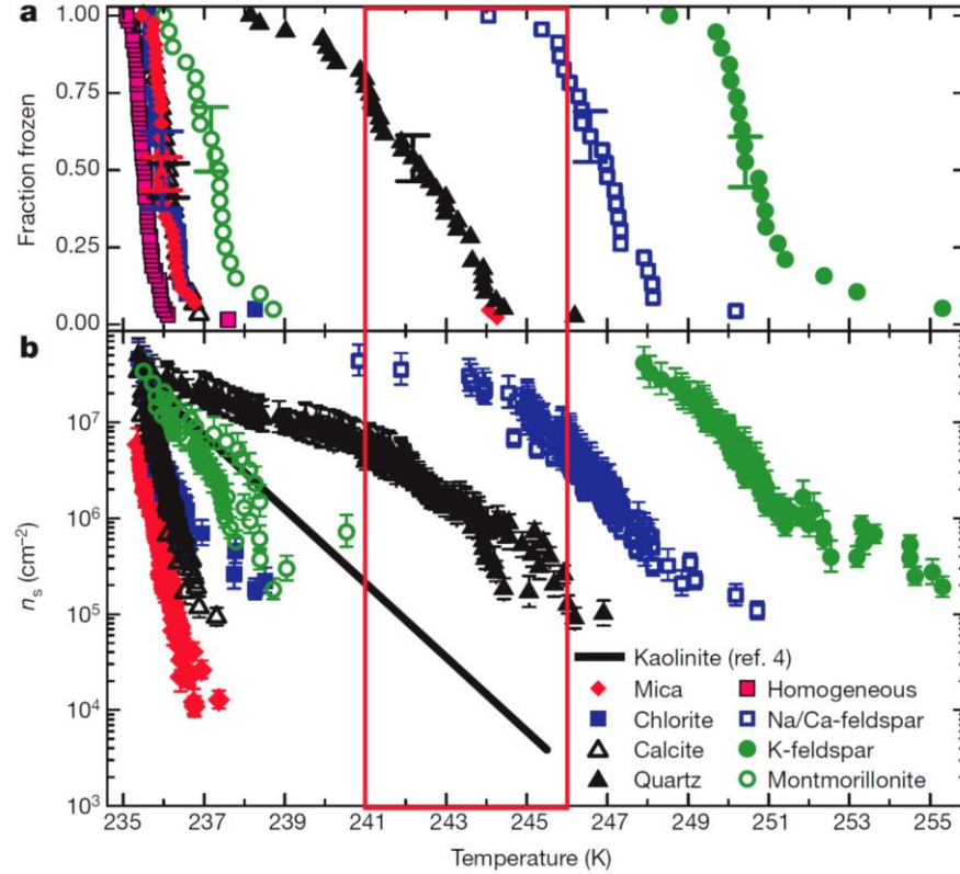
Figure 1: Experimental freezing results for individual minerals (Atkinson et al. 2013).
