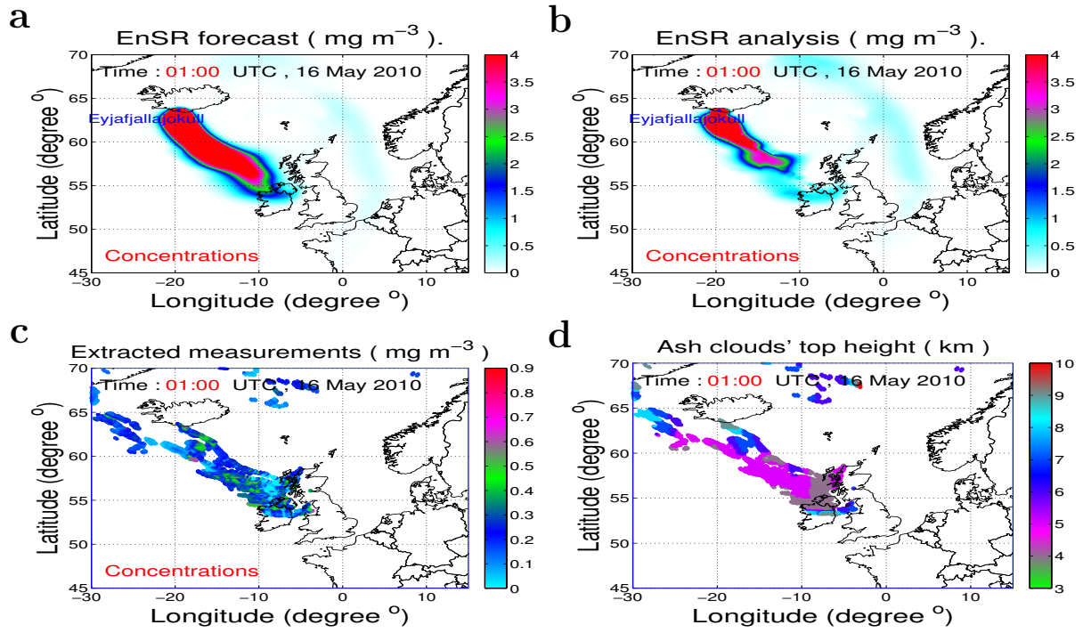
Figure 4. Examination of EnSR effect when assimilating SEVIRI-extracted ash concentrations at 01:00 UTC 16 May 2010. a , EnSR forecast (ensemble mean) of \text{PM}_{10} concentrations. b , EnSR analysis (ensemble mean) of \text{PM}_{10} concentrations. c , Extracted measurements of \text{PM}_{10} concentrations from the satellite observational operator. Ash concentrations shown in a , b , c are at the ash cloud top layer height d .
