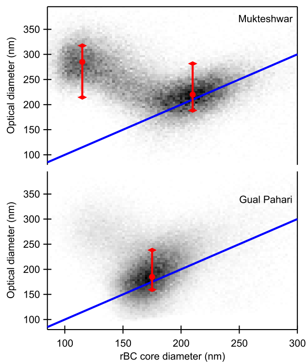
Figure 7. Distributions of single particle optical and rBC core diameters for the 360 nm mobility size and 30–35 °C instrument temperature range (darker color indicates higher probability). The blue lines indicate equal rBC and optical diameters. The red markers represent the mode center points and the error bars are based on calculations using different optical constants (ammonium sulfate and rBC).
