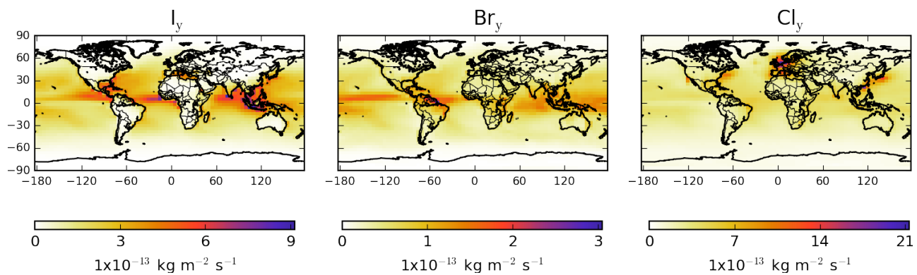
Figure 2. Annual global X_y ( X=\text{Cl}, \text{Br}, \text{I} ) deposition (defined in Footnote 1). Values are given in terms of mass of halogen deposited ( \text{kg X m}^{-2} \text{ s}^{-1} , X=\text{Cl}, \text{Br}, \text{I} ).
