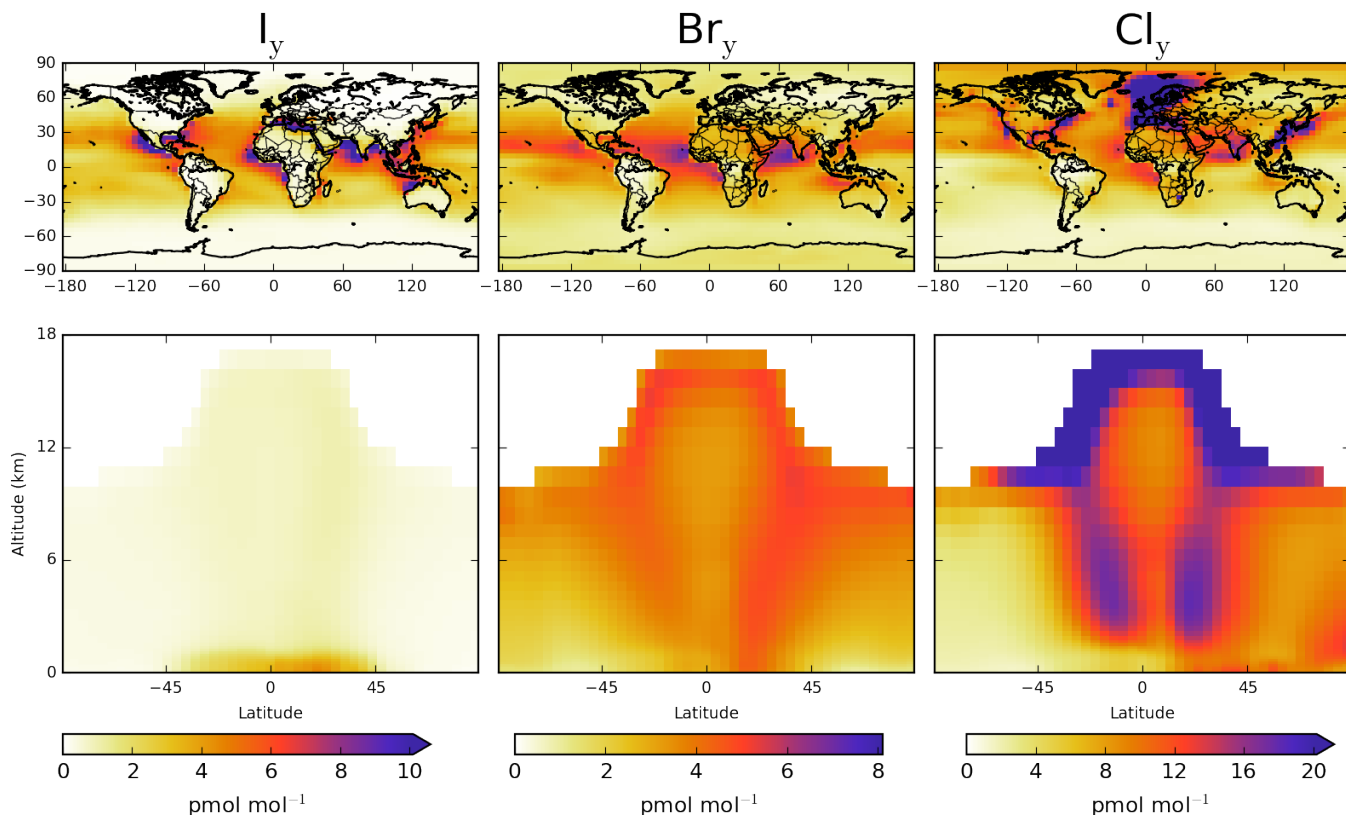
Figure 3. Tropospheric distribution of Cl_y , Br_y , and I_y (defined in Footnote 1) concentrations. Upper plots show surface and lower plots show zonal values. Only boxes that are entirely tropospheric are included in this plot. The Cl_y colourbar is capped at 20 \text{ pmol mol}^{-1} , with a maximum plotted value of 116 \text{ pmol mol}^{-1} at the surface over the North Sea. The I_y colourbar is capped at 10 \text{ pmol mol}^{-1} , with a maximum plotted value of 16.4 \text{ pmol mol}^{-1} at the surface over the Red Sea.
