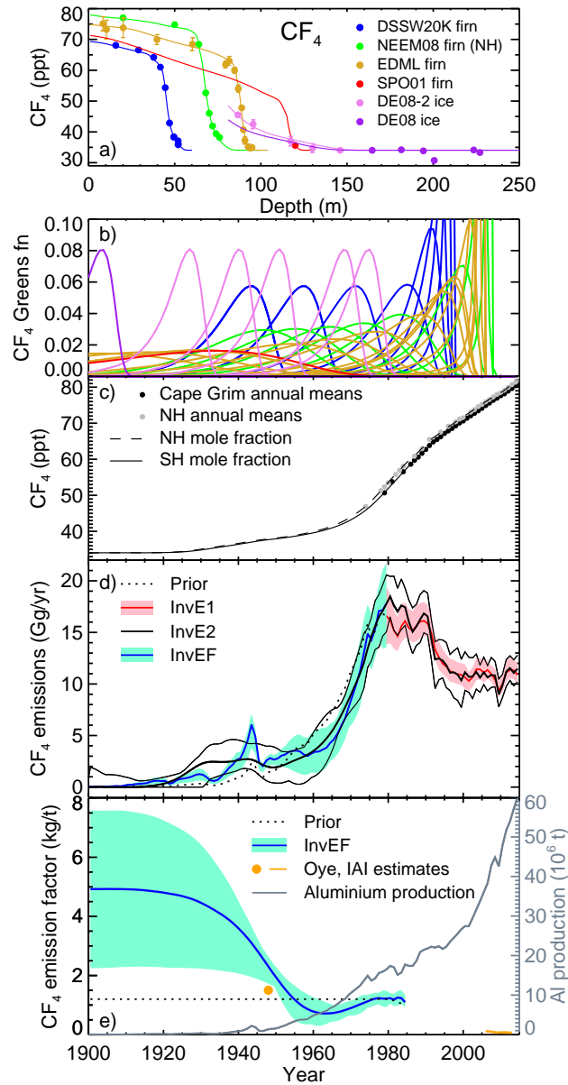
Figure 2. a) Depth profiles of CF_4 mole fraction in the firn and ice. Lines show model results corresponding to inferred emissions from InvE2; symbols are measurements with 1\sigma uncertainties. b) Green's functions from the CSIRO firn model (colors correspond to those in panel a)). c) Time history of mole fraction in the northern hemisphere (NH, dashed line) and southern hemisphere (SH, solid line) calculated with emissions inferred by InvE2. Symbols show annual values determined from atmospheric measurements in each hemisphere. d) Emissions inferred from the three inversions, with 95% confidence intervals. The dotted line shows the prior estimate based on a constant emission factor. e) Emission factor inferred by the InvEF inversion with 95% confidence intervals (blue), and constant prior (dotted). Emission factor estimated by Oye et al. (1999) for 1948 (orange circle) and recent estimates by the International Aluminium Institute (2014) (orange line, lower right corner). Primary aluminium production (U.S. Geological Survey, 2014; International Aluminium Institute, 2014) in 10^6 t (million metric tonnes) is shown with the grey line (right axis).
