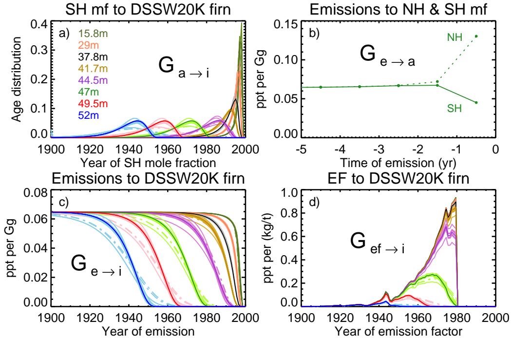
Figure 1. a) Green's functions ( G_{a \rightarrow i} ) relating the mole fraction at DSSW20K measurement depths to high latitude southern hemisphere (SH) atmospheric mole fraction, from the firm models, with different colours for each depth. The dark coloured lines show the preferred Green's functions from the CSIRO model, while the lighter coloured lines show the other members of the ensemble of Green's functions, with the Green's functions from the LGGE-GIPSA firm model shown with the dot-dashed lines. b) Green's functions ( G_{e \rightarrow a} ) describing the relationship between atmospheric mole fraction in ppt in the high latitude northern hemisphere (NH, dashed line) and high latitude southern hemisphere (solid line) and annual global \text{CF}_4 emissions in Gg in preceding years, from the AGAGE 12-box model based on the spatial emissions distribution described in the text. We define mole fractions to correspond to the start of the year and emissions to correspond to the middle of the year. The x-axis gives the time of emission relative to the time of atmospheric mole fraction. c) Green's functions ( G_{e \rightarrow i} ) relating the mole fraction at DSSW20K measurement depths to annual global \text{CF}_4 emissions, derived by combining the Green's functions in parts a) and b). Line styles and colors are as in a). d) Green's functions ( G_{ef \rightarrow i} ) relating the mole fraction at DSSW20K measurement depths to annual global \text{CF}_4 emission factor in kg/t, derived by combining the Green's functions in part c) with annual global primary aluminium production up to 1980. Line styles and colors are as in a).
