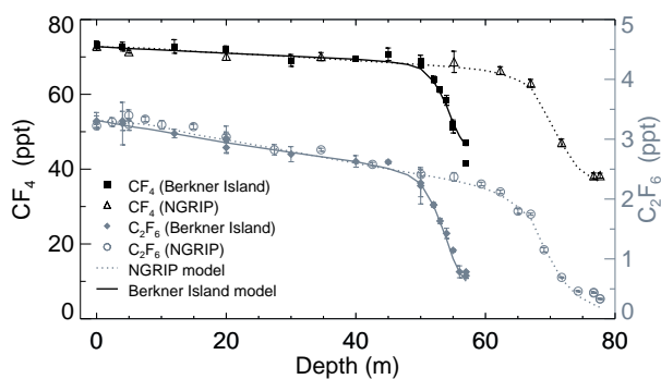
Figure 7. \text{CF}_4 and \text{C}_2\text{F}_6 at Berkner Island and North GRIP. Symbols show measurements from Worton et al. (2007), that were not used in our inversions. Lines show modelled depth profiles created by convolving our inferred atmospheric mole fraction timeseries in the appropriate hemisphere with Green's functions from the LGGE-GIPSA firm model. \text{CF}_4 is shown in black (left axis) and \text{C}_2\text{F}_6 in grey (right axis).
