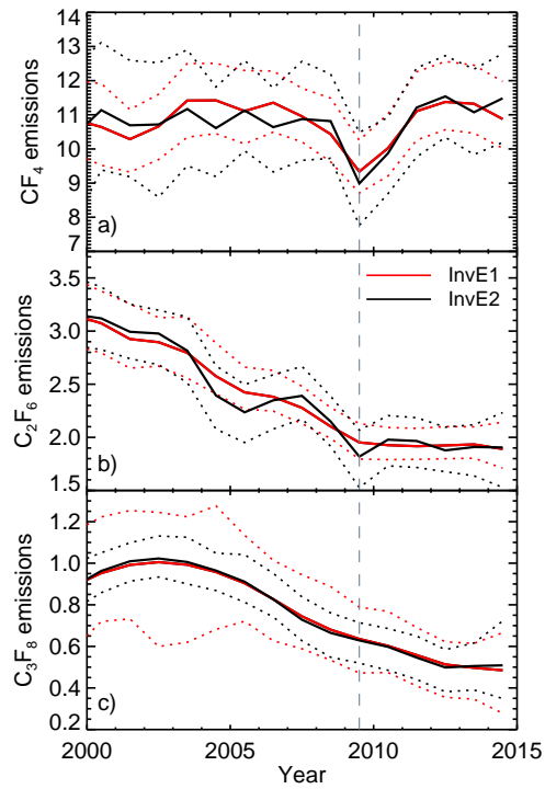
Figure 8. a) CF_4 , b) C_2F_6 and c) C_3F_8 emissions (Gg/yr) from 2000 for the InvE1 inversion in red and the InvE2 inversion in black. Uncertainty ranges shown for both models are 95% confidence intervals.
